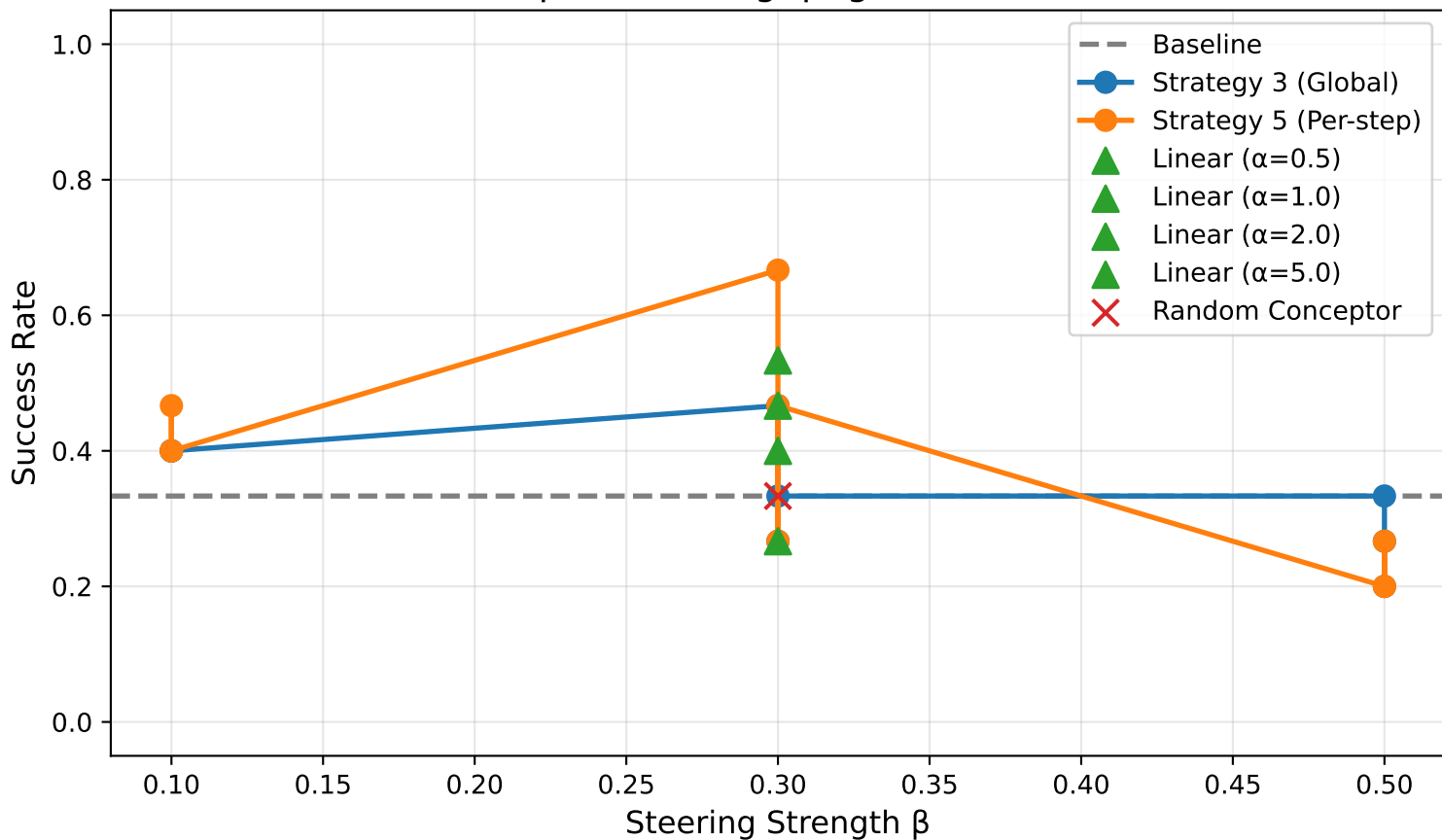
Conceptor Steering: peg-insert-side-v3
