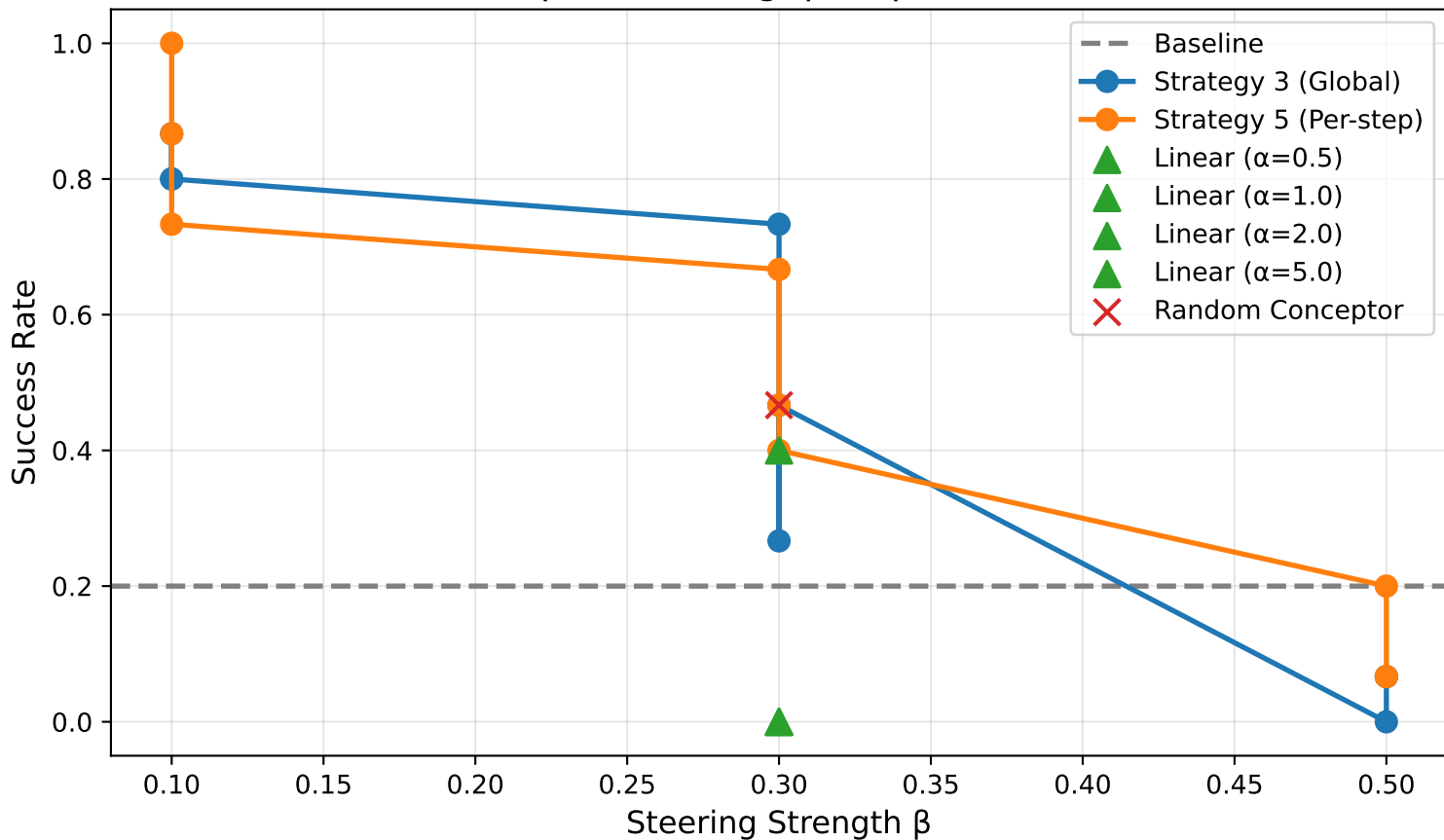
Conceptor Steering: pick-place-wall-v3
