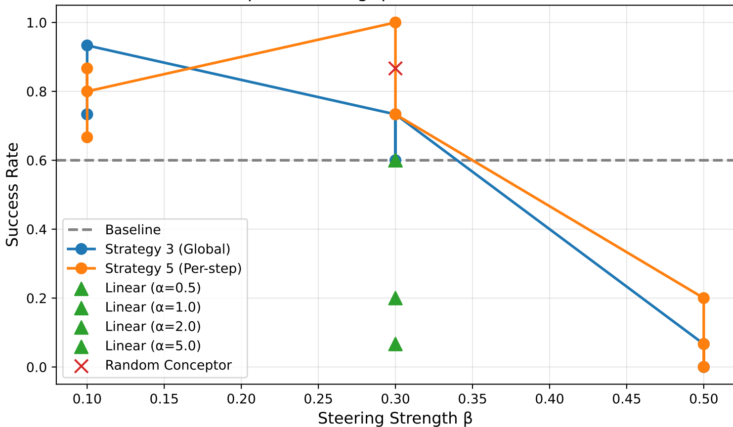
Conceptor Steering: plate-slide-back-side-v3
