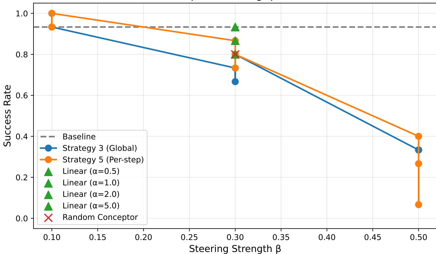
Conceptor Steering: push-v3
