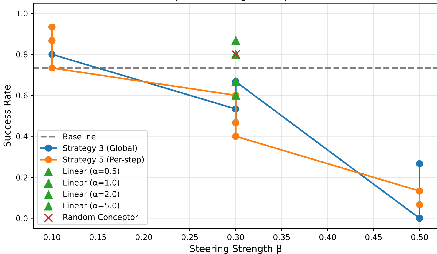
Conceptor Steering: shelf-place-v3
