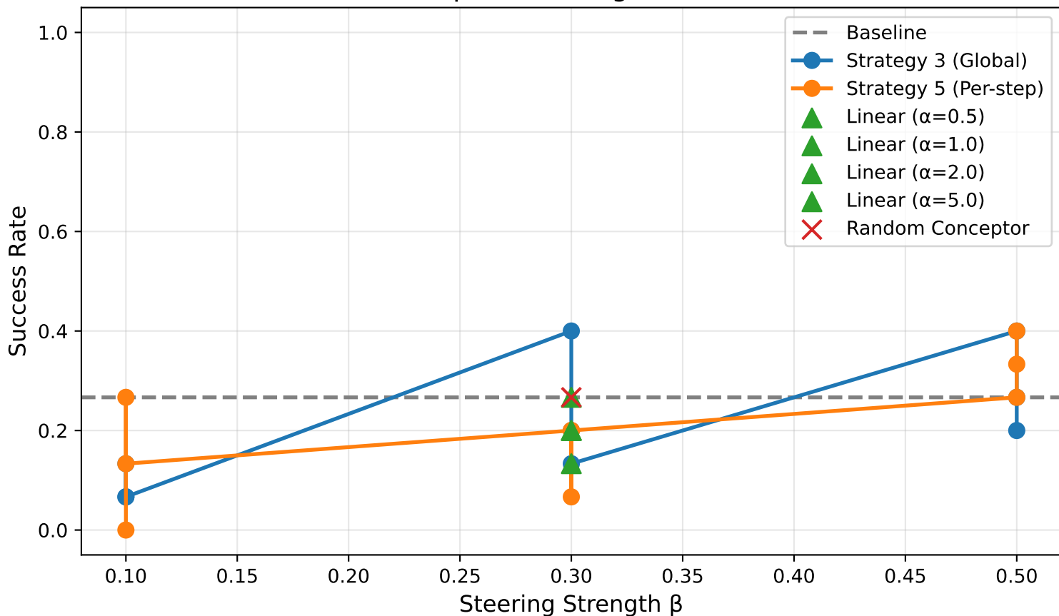
Conceptor Steering: soccer-v3
