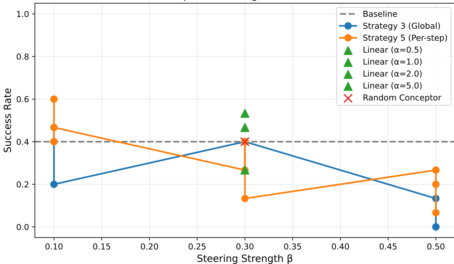
Conceptor Steering: basketball-v3
