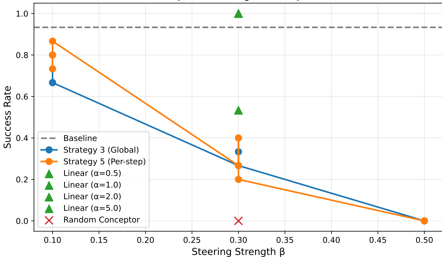
Conceptor Steering: coffee-pull-v3
