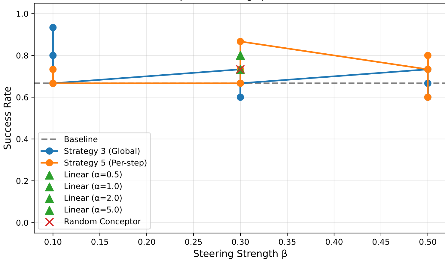
Conceptor Steering: push-back-v3
