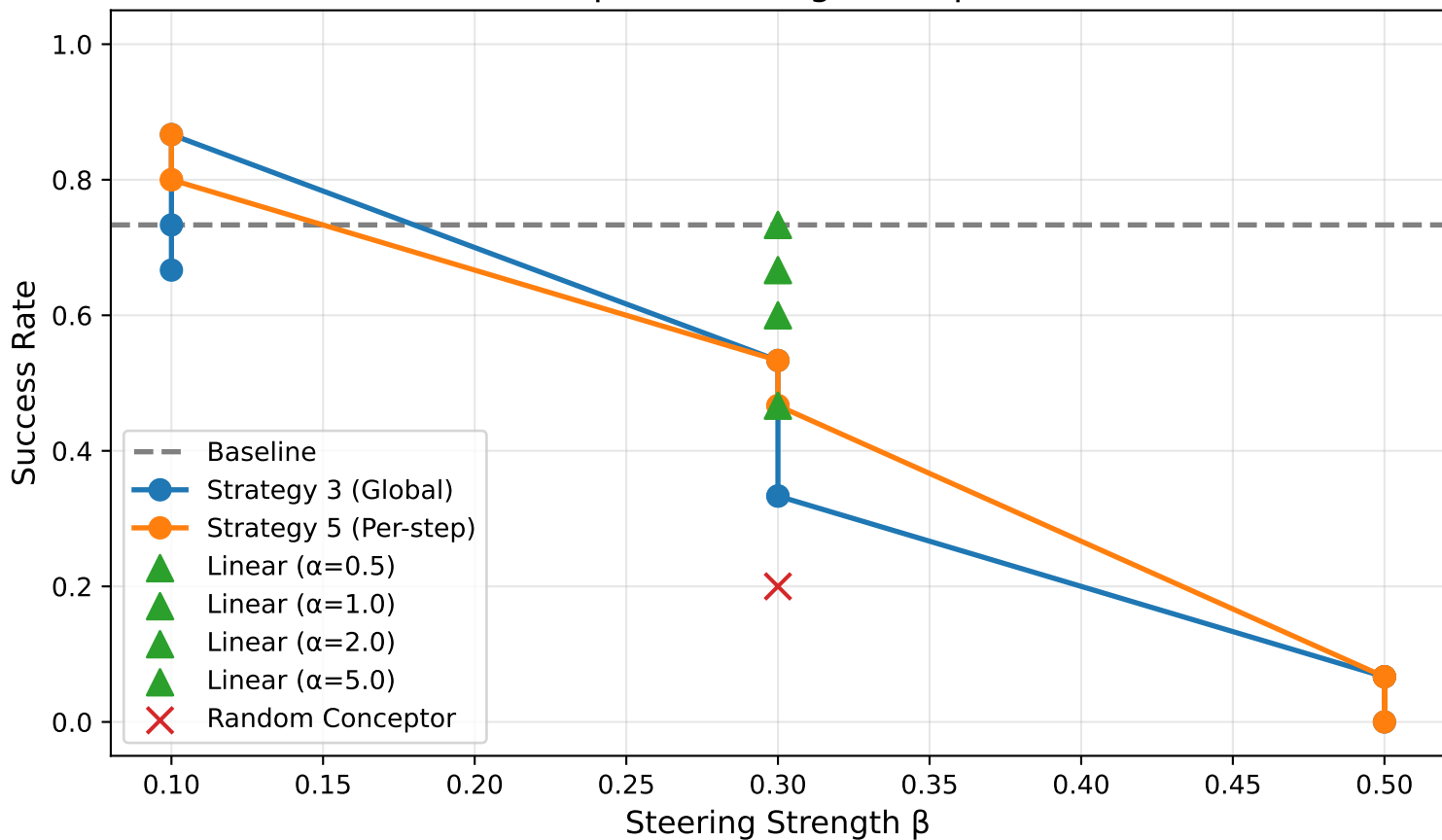
Conceptor Steering: stick-pull-v3
