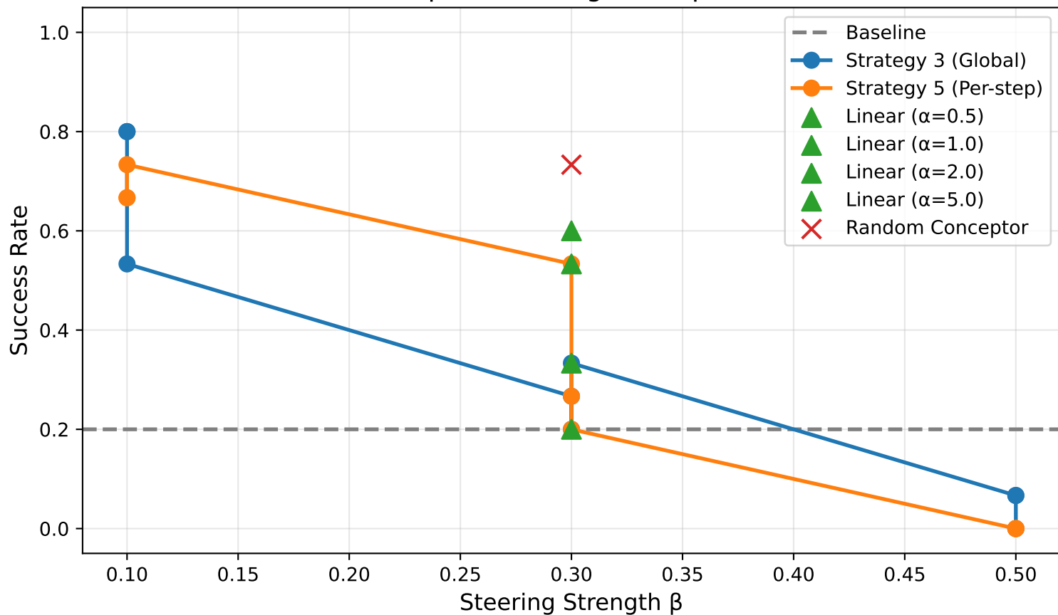
Conceptor Steering: stick-push-v3
