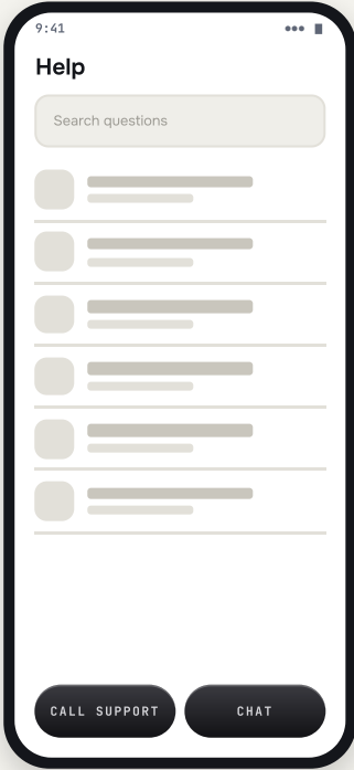
C9 Help & FAQ LANELISTSCAFFOLD Grievance contact (DPDP) at the bottom.
