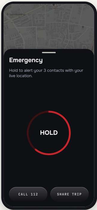
U1-SOS SOS sheet LANESHEET 1.5 s hold, Gradient Beam ring fills red. Opens SMS app pre-filled.
