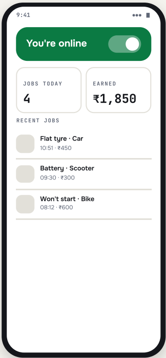
M3 Dashboard LANELISTSCAFFOLD Toggle 64 dp. Online = location every 60 s / 100 m.
