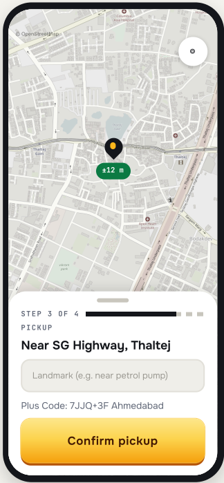
U6 Confirm location LANEMAPSCAFFOLD Drag map under fixed pin. Badge: green ≤20 m, amber ≤50 m.
