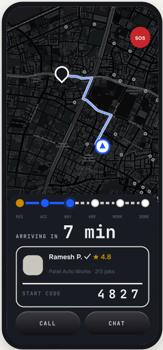
U10 Live tracking LANEMAPSCAFFOLD Marker glides between 5 s fixes. Tap code = fullscreen.
