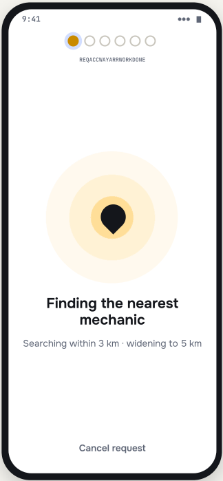
U8 Searching LANESTATUSSCAFFOLD BreathingPulse 10 s cycle. No spinner.
