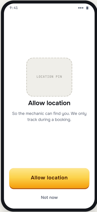
C7 Permission explainer LANESTATUSSCAFFOLD Shown BEFORE each system prompt (Play policy). Same for camera, notifications.
