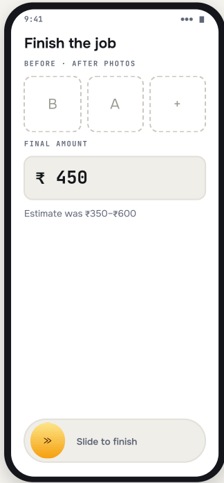
M7 Job complete LANEFLOWSCAFFOLD ≥1 after photo required. Amount outside 0.5–3× needs a reason.
