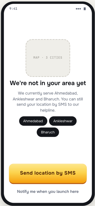
U1-Area Outside service area LANESTATUSSCAFFOLD createBooking rejects pickups outside an active serviceAreas/{cityId}.
