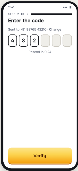
C6 Enter OTP LANEFLOWSCAFFOLD Auto-fill via SMS Retriever (no SMS permission).
