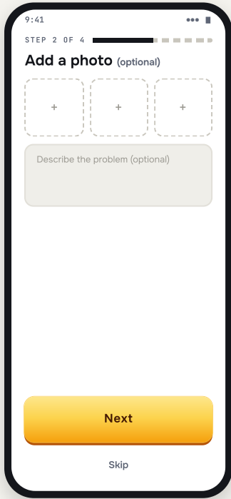
U5 Photos + details LANEFLOWSCAFFOLD Compress ≤ 500 KB, strip EXIF before upload.
