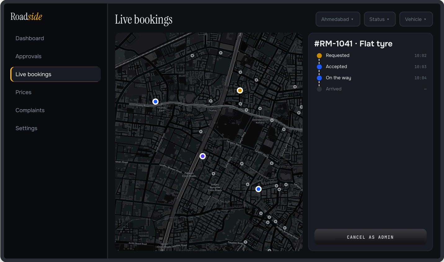
A3 Live bookings Only active bookings shown on the map.
