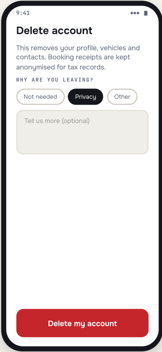
C10 Delete account LANEFORMSCAFFOLD Needs re-login within 5 min. Also a web deletion page.
