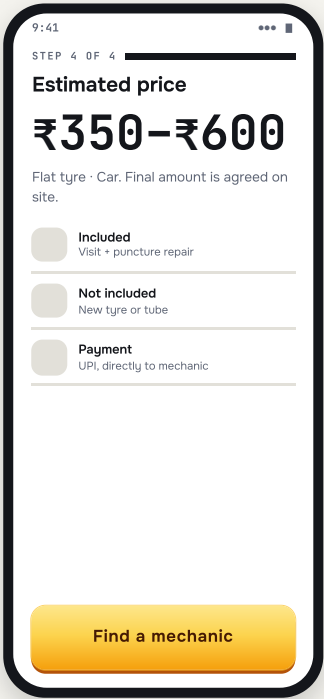
U7 Price estimate LANEFLOWSCAFFOLD Price computed by server from prices/collection.
