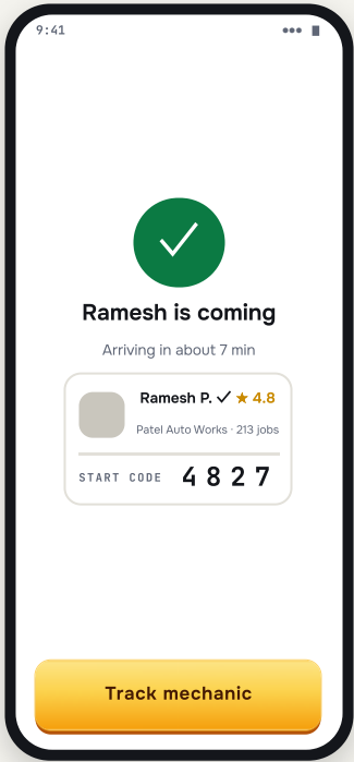
U9 Mechanic assigned LANESTATUSSCAFFOLD TrustPass slides up + success haptic.
