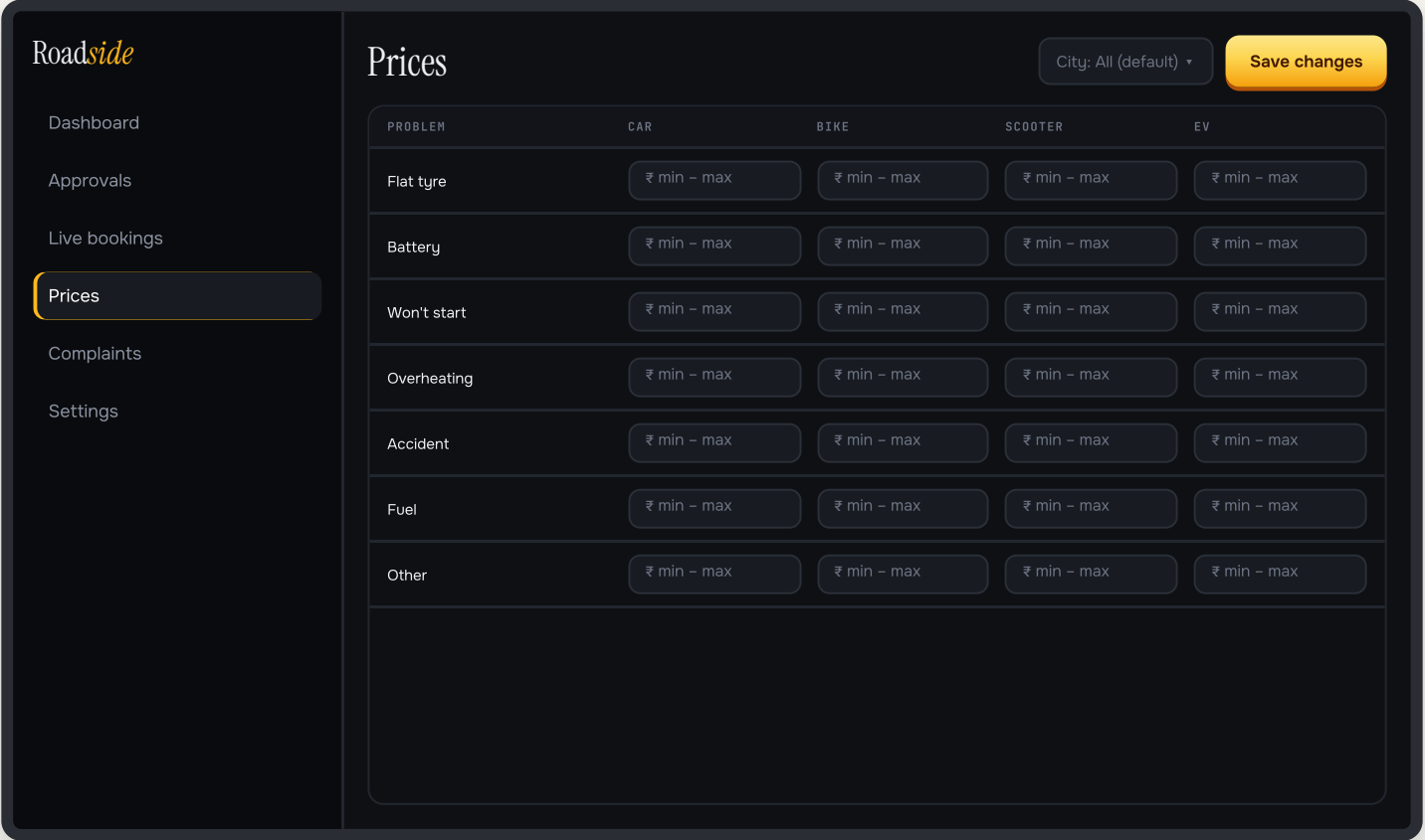
A4 Price editor Validates min < max. Change logged in auditLogs.
