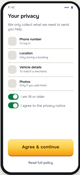
C4 Privacy & consent LANEFORMSCAFFOLD DPDP notice in en/hi/gu. Save consent.version + time.
