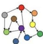
Graph
