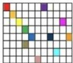
Column-Family
