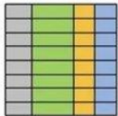
Relational
