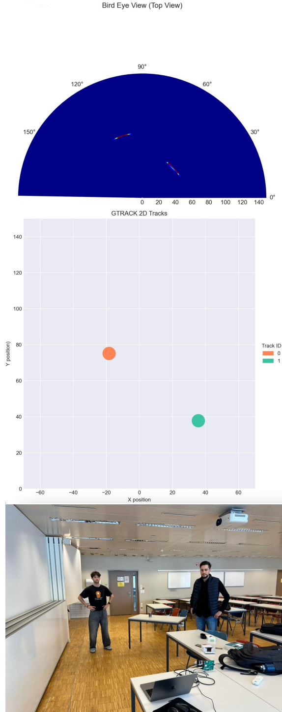
Figure 1: Real-time visualization showing tracked positions on polar and cartesian 2D projections after GTrack, and the corresponding real-scene with 2 persons in a classroom with obstacles.
