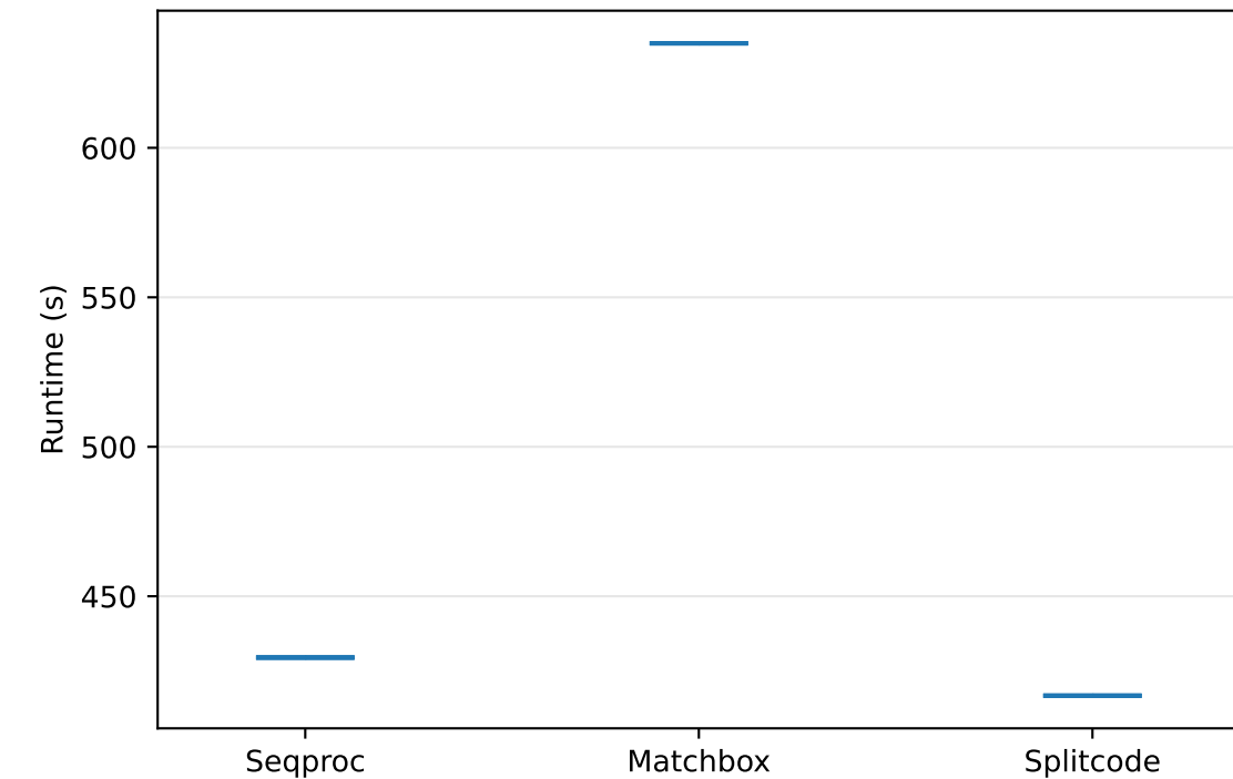
sci-RNA-seq3 - Runtime
