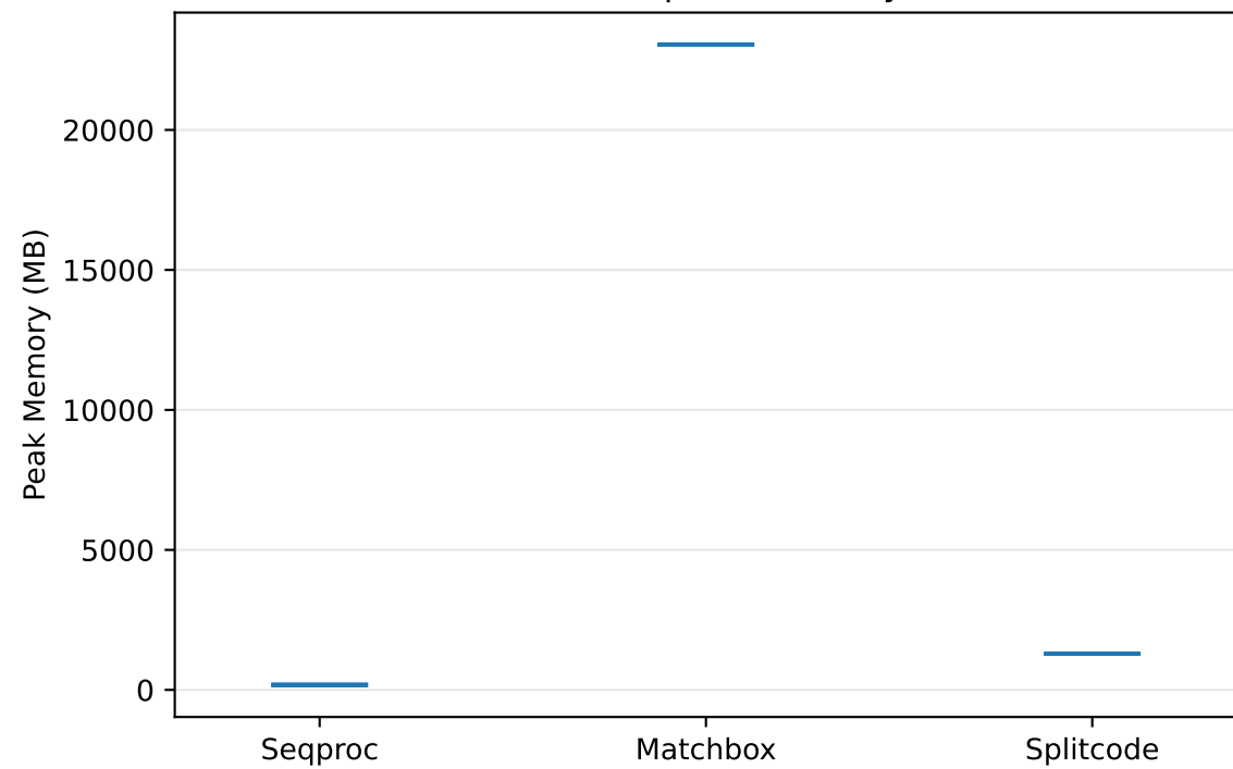
LR-SPLiT-seq - Memory
