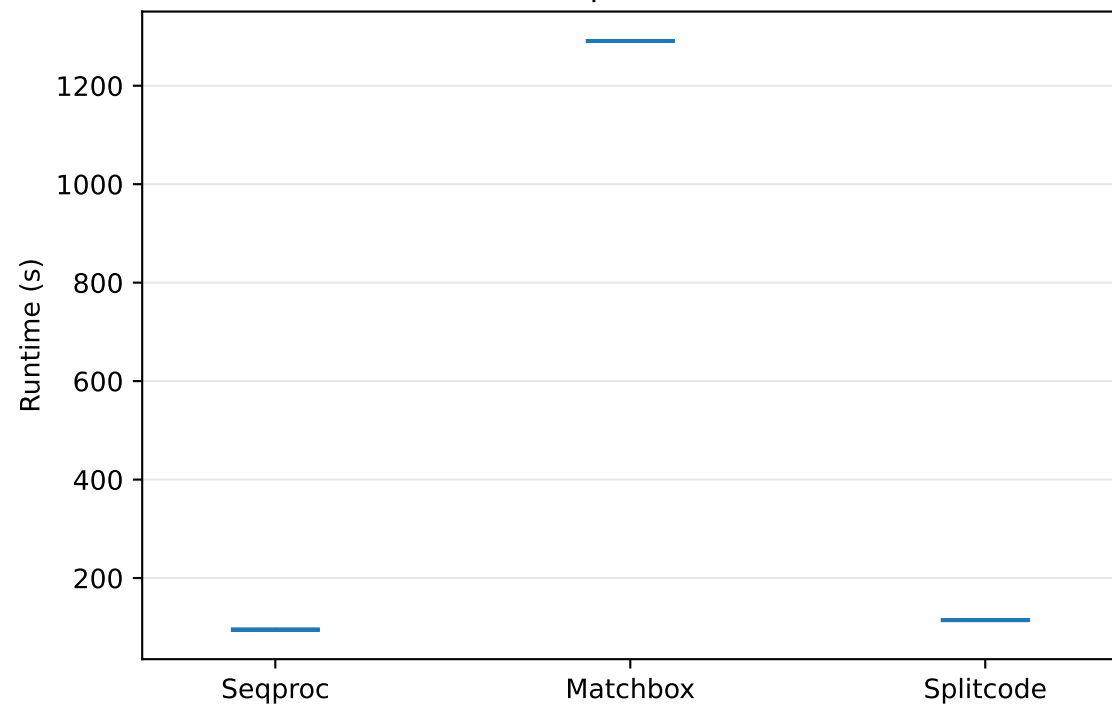
LR-SPLiT-seq - Runtime
