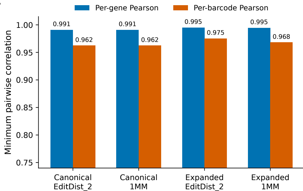
Worst-pair count concordance
