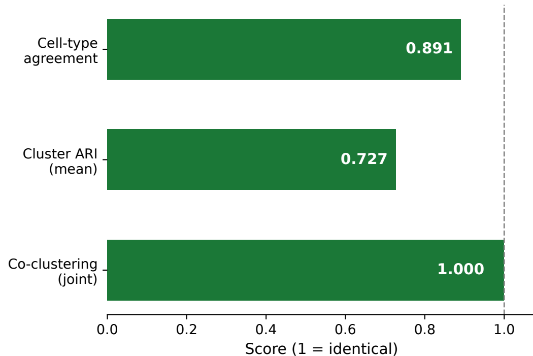
Tool concordance shared cells n=220, 3 tools
