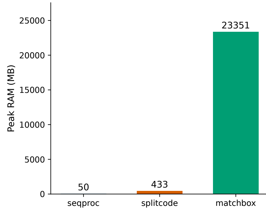
Read processing peak memory
