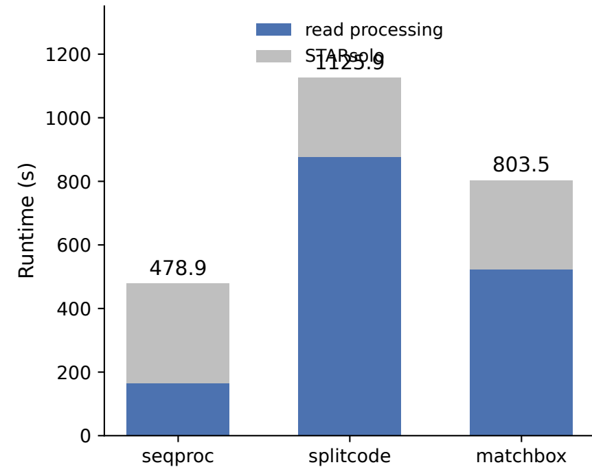
Total runtime per tool
