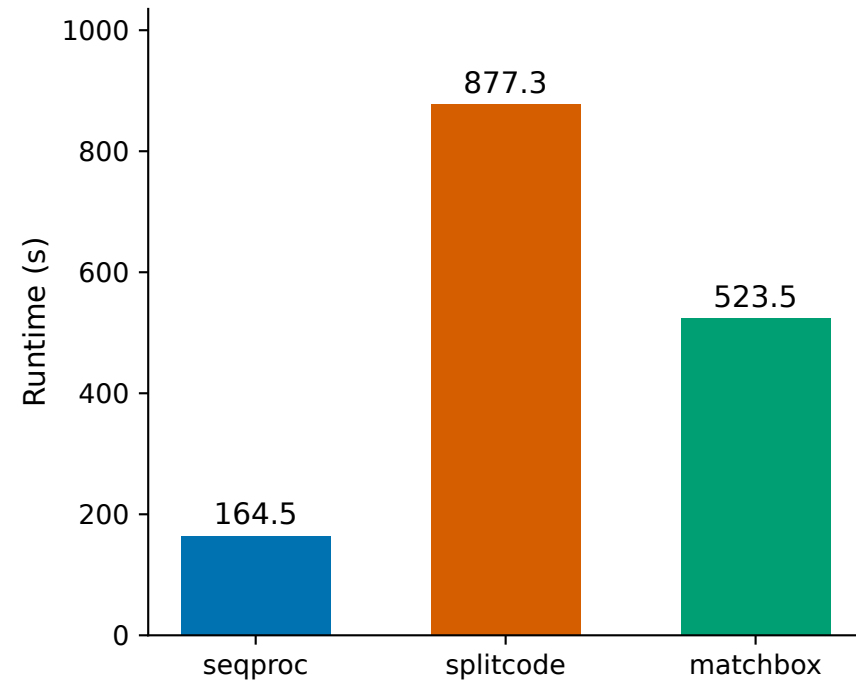
Read processing runtime
