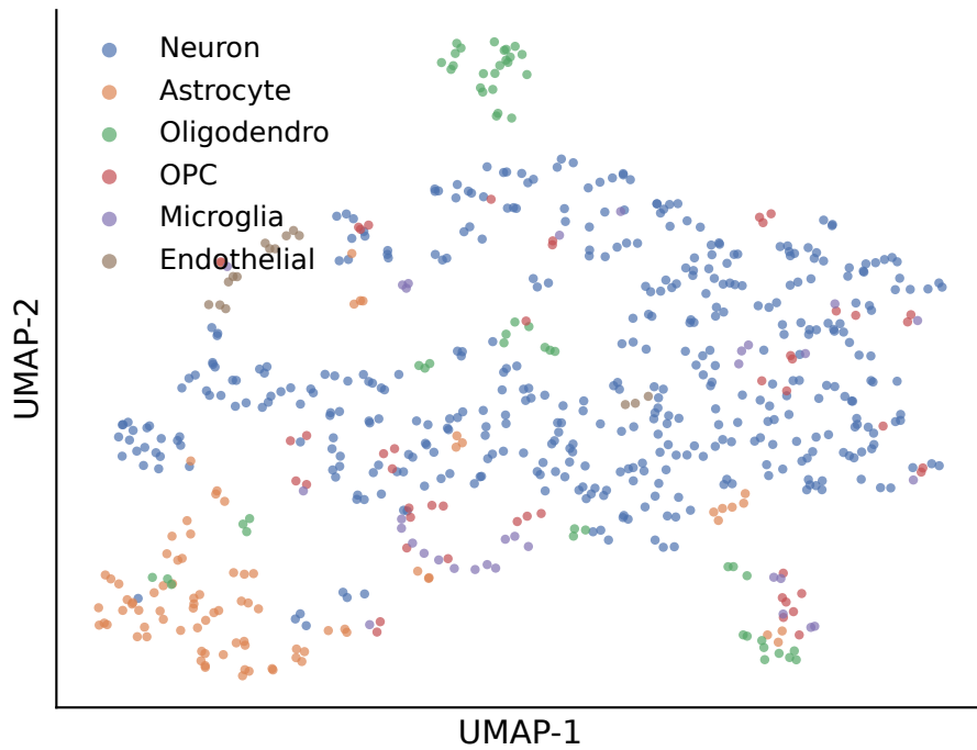
Joint embedding by cell type
