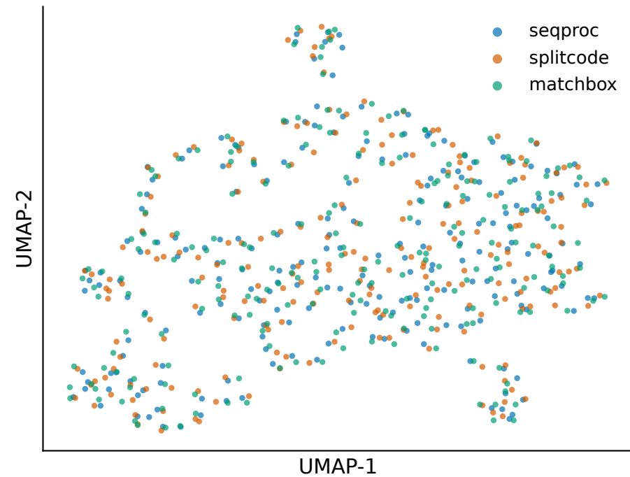
Joint embedding by tool (overlap = agreement)
