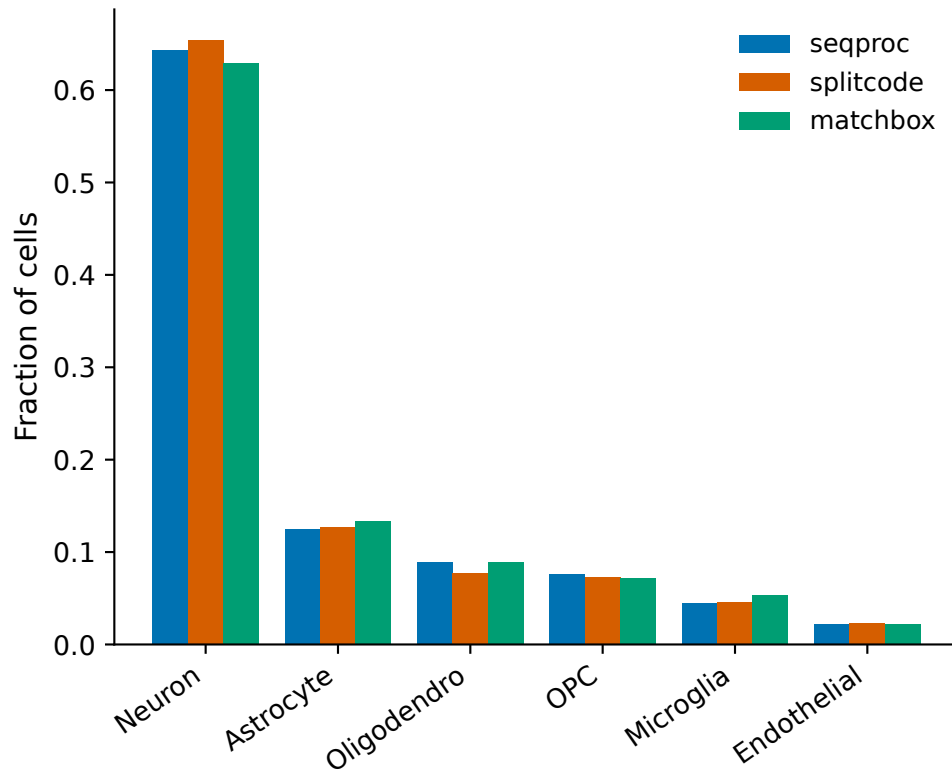
Cell-type composition
