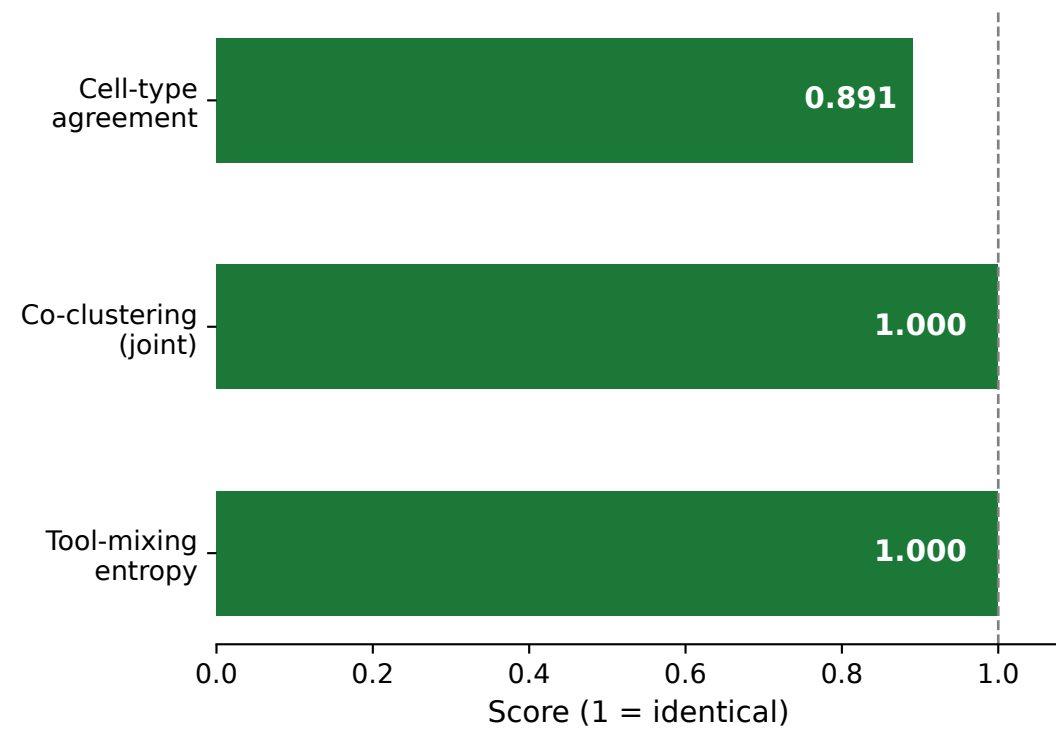
Tool concordance (robust) shared cells n=220, 3 tools
