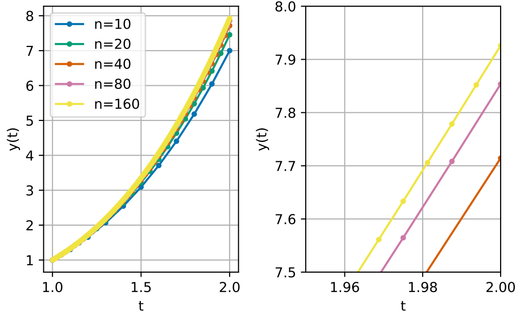
Figure 3.1: Plots of solution using Euler's method
