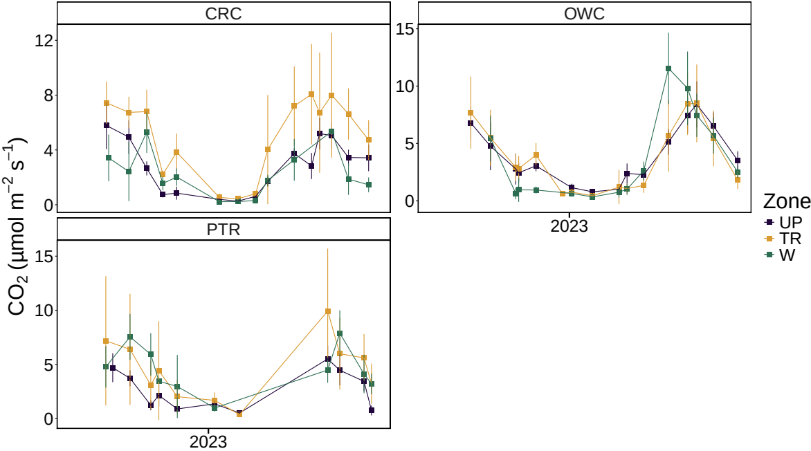
CO 2 Soil Fluxes by Year, Site & Zone
