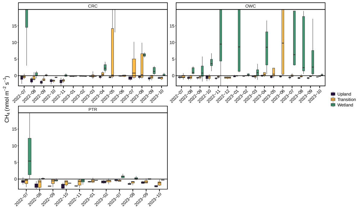
Summary Boxplot of CH 4 Soil Fluxes by Site & Zone
