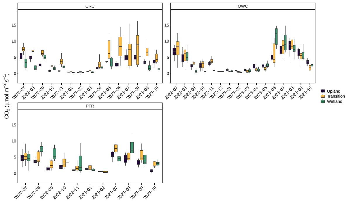
Summary Boxplot of CO 2 Soil Fluxes by Site & Zone
