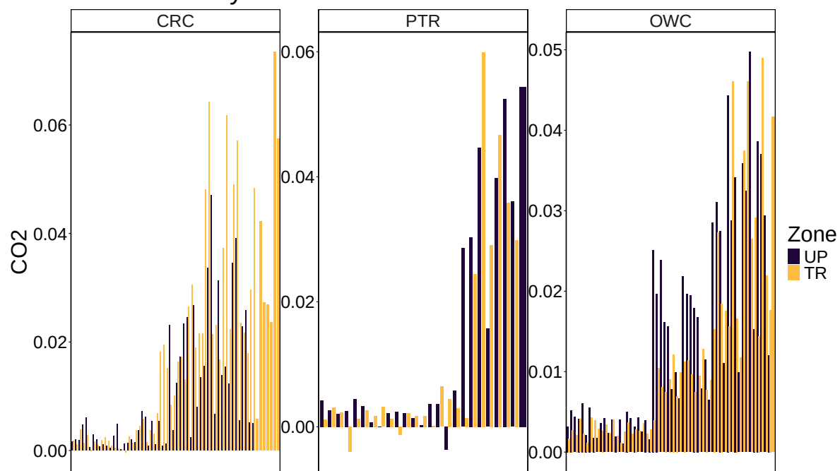
CO2 Fluxes by Site
