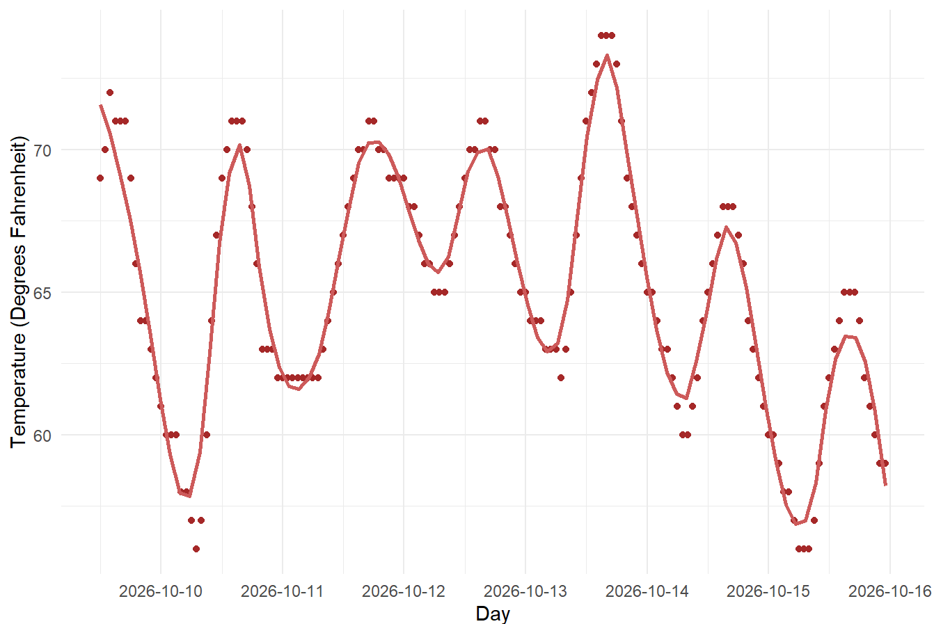
MSM Temperature Forecasts for the Week of 2026-10-09
