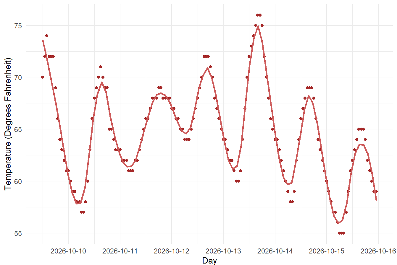
TMP Temperature Forecasts for the Week of 2026-10-09
