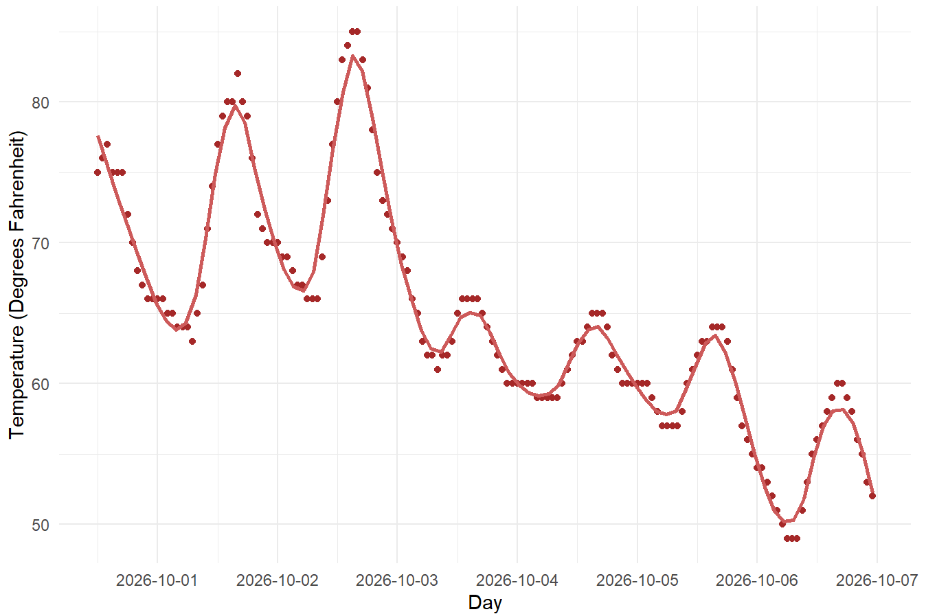
TMP Temperature Forecasts for the Week of 2026-09-30
