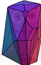
progressive simplification
