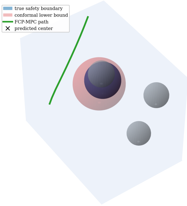
Fig. 4. True and conformal safety bounds in 3D, zoomed onto a single obstacle. The solid blue ball is the true safety boundary D_{t+i}(x) = r_{\text{safe}} around the actual obstacle (used only for evaluation); the translucent red shell is the conformal lower-bound boundary \underline{D}_{t+i|t}(x) = r_{\text{safe}} obtained from the functional calibration, i.e. the nominal safety region around the predicted center inflated by the calibrated margin. The conformal surface encloses the true one, certifying coverage, and the executed FCP-MPC path (green) threads just outside it—progressing efficiently while respecting the worst-case safety constraint. Faint gray spheres are other obstacles in the scene.
