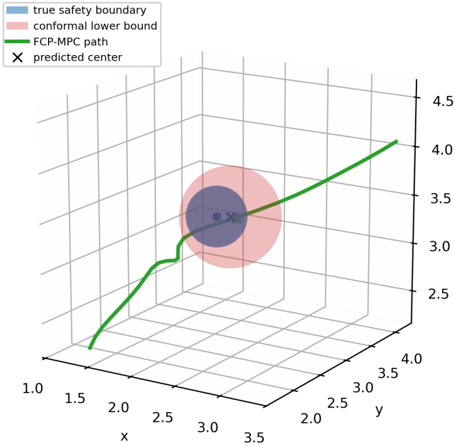
Fig. 4. The conformal safety bound in 3D, zoomed onto a single obstacle (the 3D analogue of the 2D illustration in Fig. 2). The solid blue surface is the true safety boundary D_{t+i}(x) = r_{\text{safe}} around the actual obstacle (used only for evaluation); the translucent red surface is the conformal lower-bound boundary \underline{D}_{t+i|t}(x) = r_{\text{safe}} obtained from the functional calibration, i.e. the nominal safety region around the predicted center (x) inflated by the calibrated margin. The conformal surface encloses the true one, certifying coverage, and the executed FCP-MPC path (green) threads just outside it—progressing efficiently while respecting the worst-case safety constraint.
