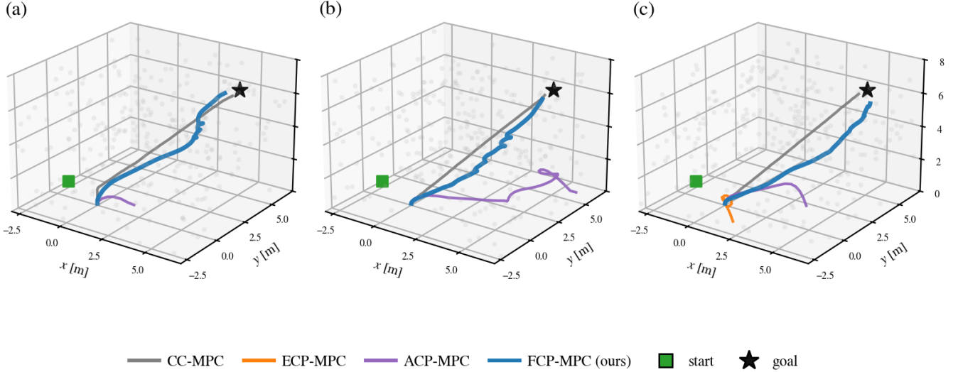
Fig. 6. Closed-loop trajectory comparison in the dense 3D quadrotor task ( M=280 dynamic obstacles) across three random seeds, shown in panels (a)–(c). Each panel overlays all four controllers—CC-MPC (gray), ECP-MPC (orange), ACP-MPC (purple), and FCP-MPC (ours, blue). Green square: start; black star: goal; gray points: obstacles. FCP-MPC makes consistent progress toward the goal across seeds despite the heavy obstacle density.
