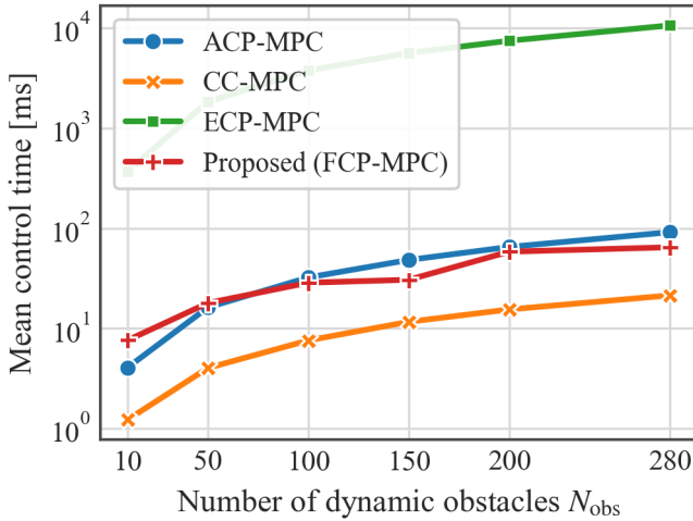
Fig. 7. Scalability comparison of MPC methods in dense 3D environments. The figure reports the mean control computation time per planning step as a function of the number of dynamic obstacles.
