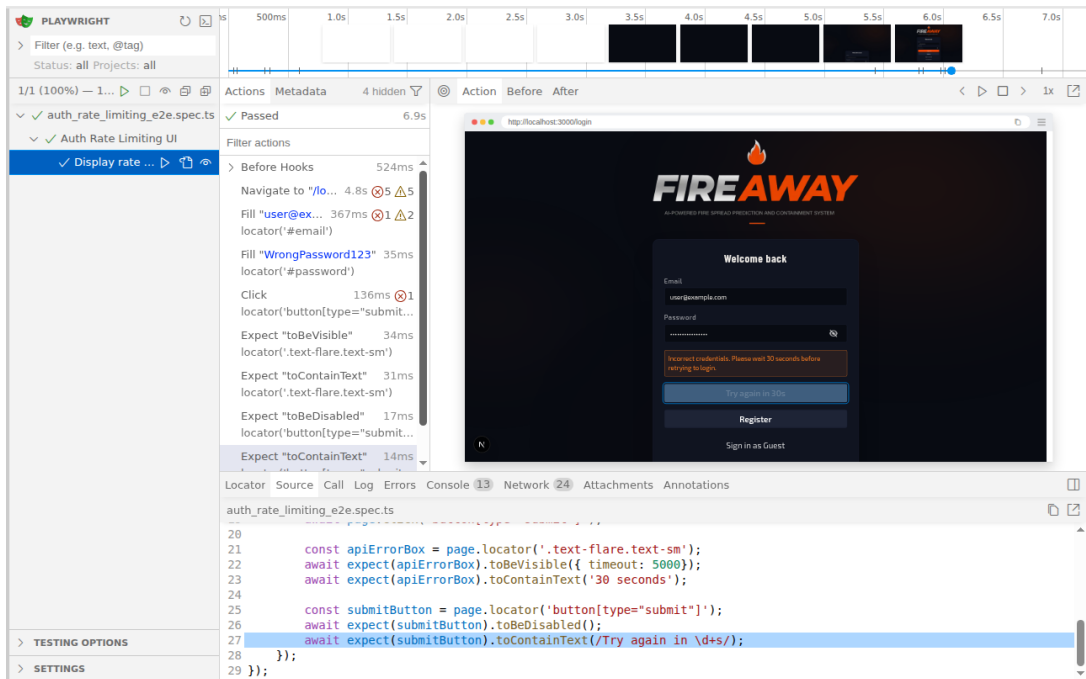
Figure 17: Playwright E2E assertion confirming UI cooldown timer and disabled submission button upon rate limit response.
