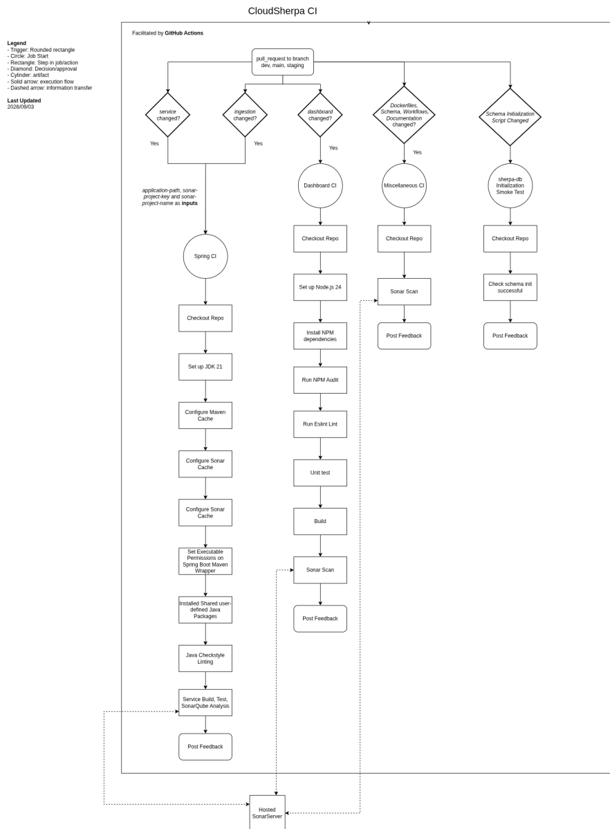
Figure 24: CI Pipeline Flow
