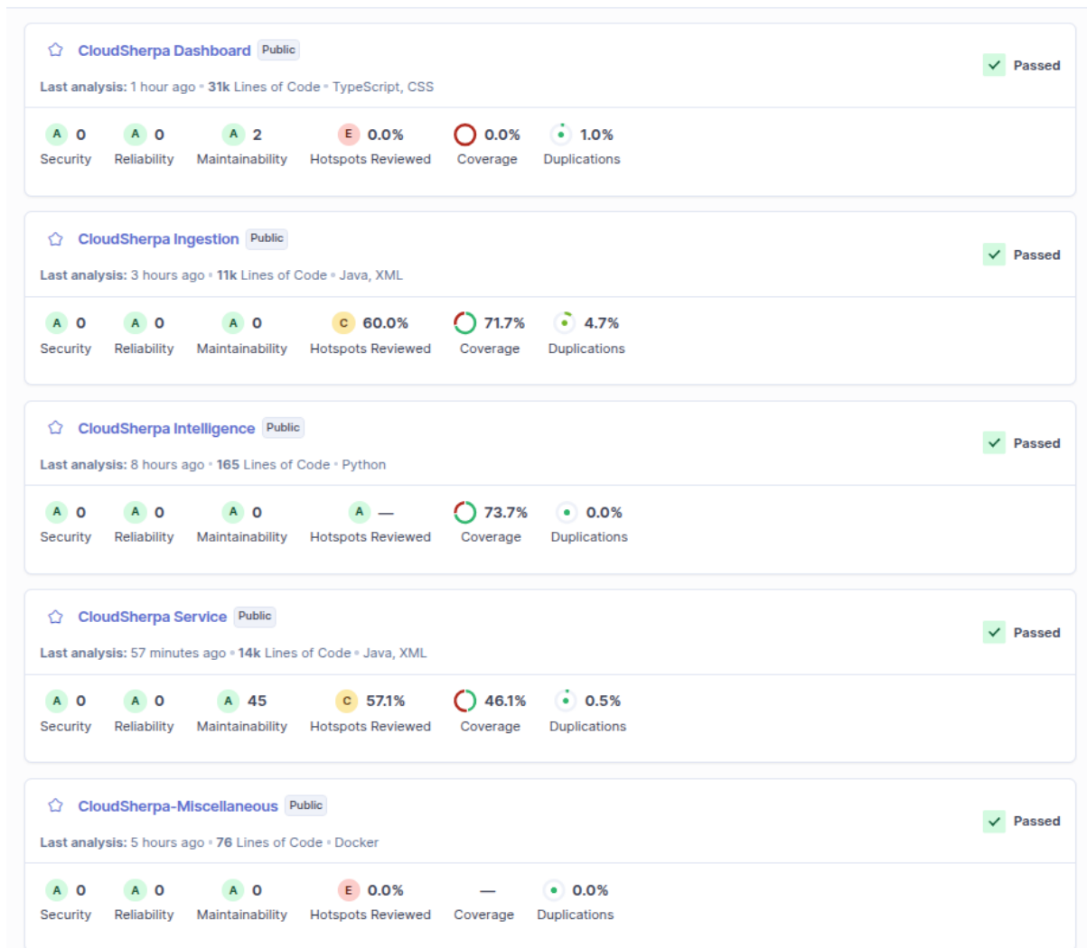
Figure 20: Self hosted SonarQube Results
