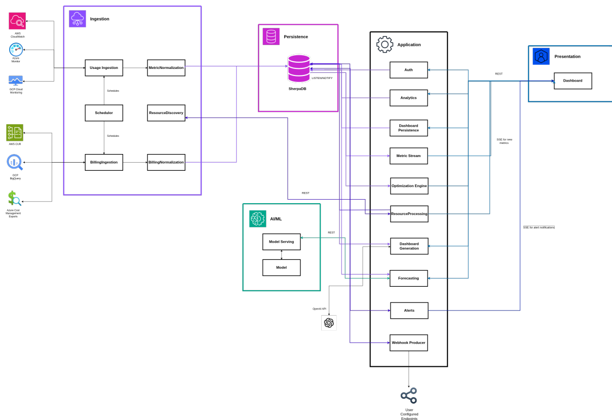
Figure 1: Architectural Diagram
