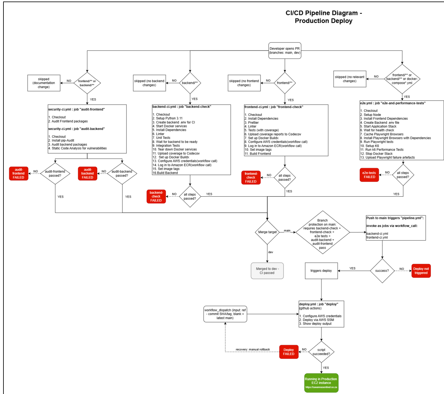
Figure 4 - CI/CD Workflow
