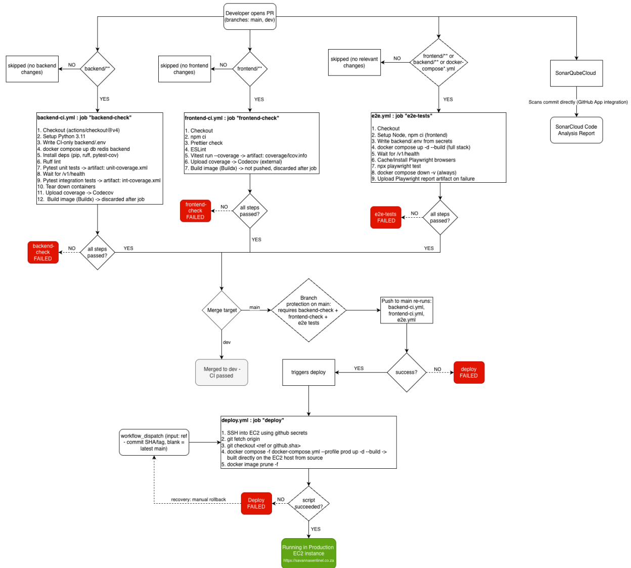
CI/CD Pipeline Diagram - Production Deploy
