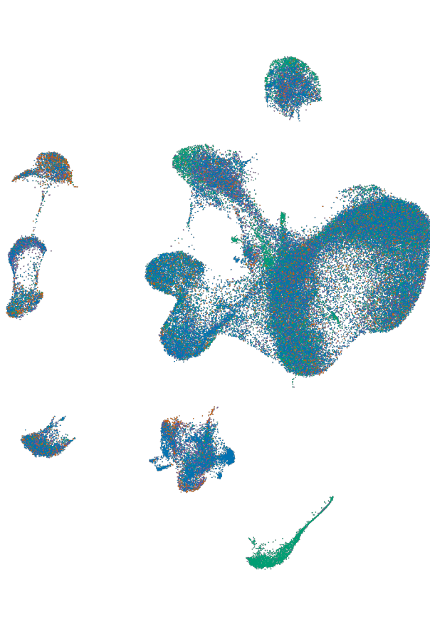
dims20_neighbor30
