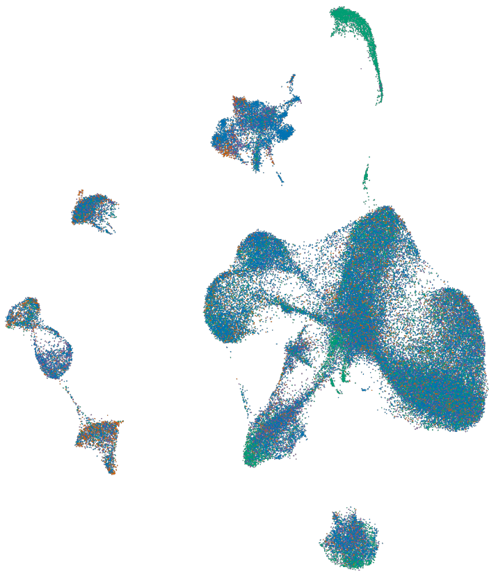
neighbor30
