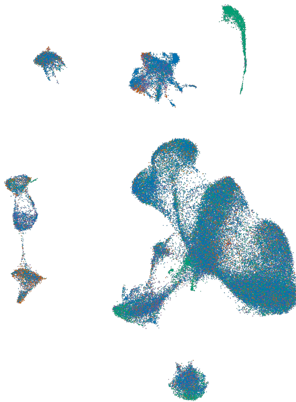
neighbor50
