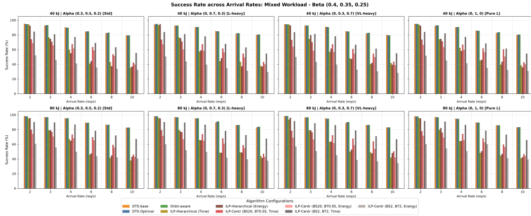
Figure 5.1. Success Rate across arrival rates under Mixed Workload \beta = (0.40, 0.35, 0.25) for 40 kJ (top) and 80 kJ (bottom) across payload distributions \alpha [cite: 1].
