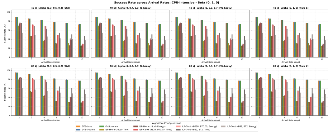
Figure 5.4. Success Rate across arrival rates under CPU-Intensive Workload \beta = (0, 1, 0) for 40 kJ (top) and 80 kJ (bottom) across payload distributions \alpha [cite: 1].
