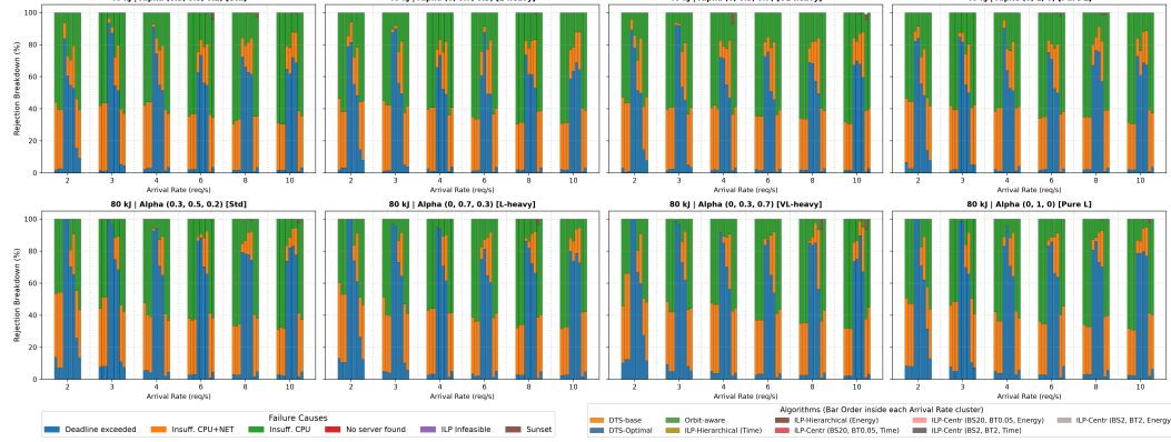
Figure 5.3. Rejection Causes distribution under Mixed Workload \beta = (0.40, 0.35, 0.25) across arrival rates, battery budgets, and payload distributions[cite: 1].
