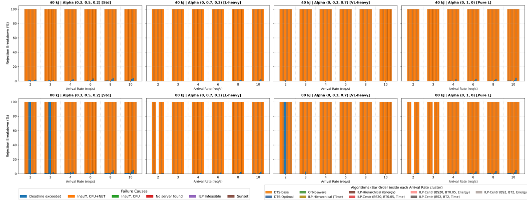
Figure 5.9. Rejection Causes distribution under Data-Intensive Workload \beta = (0, 0, 1) , showing near-total dominance of physical ISL and energy saturation ( Insuff. CPU+NET )[cite: 1].
