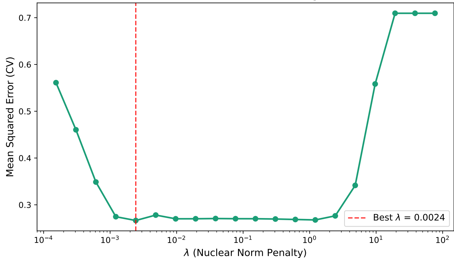
Cross-Validation for Nuclear Norm Regularization
