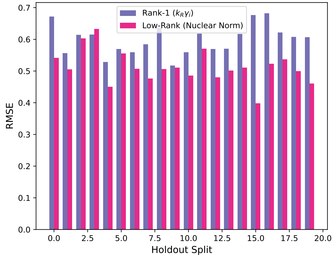
Holdout RMSE: Rank-1 vs Low-Rank
