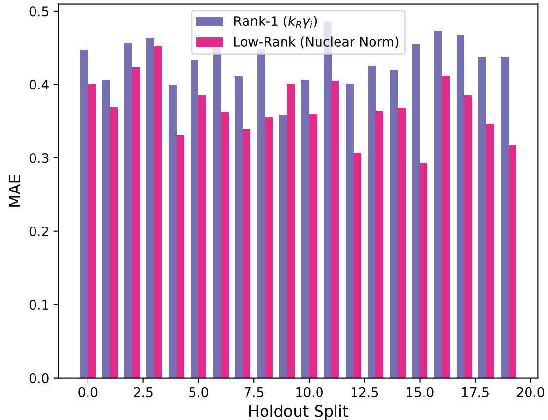
Holdout MAE: Rank-1 vs Low-Rank
