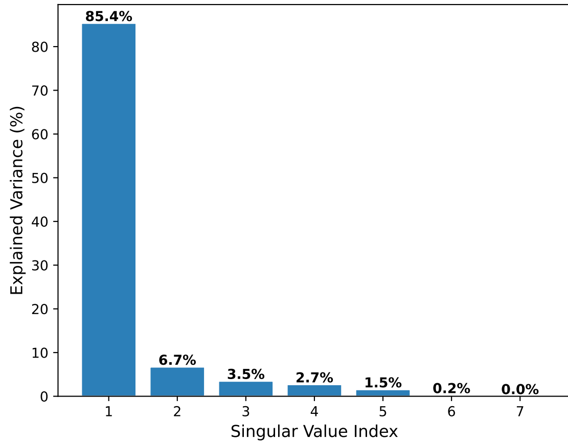
Scree Plot: Singular Value Decomposition of \Gamma
