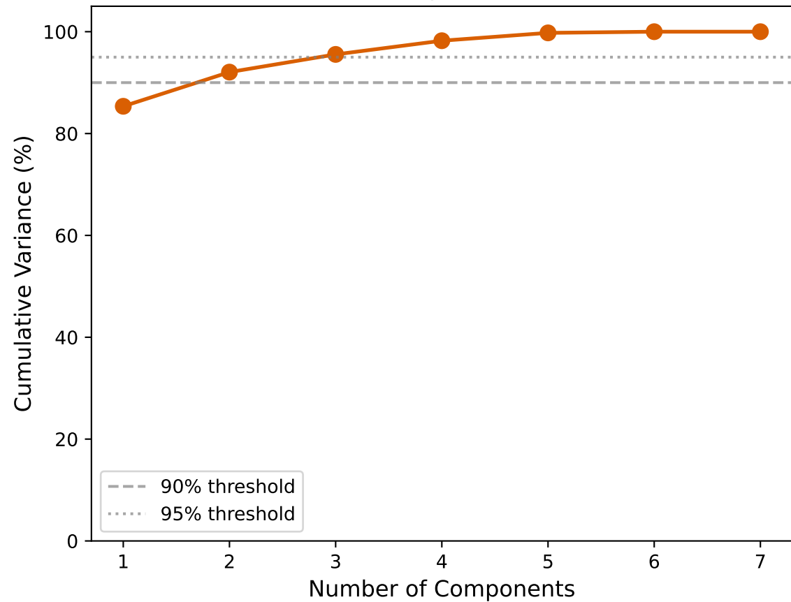
Cumulative Explained Variance
