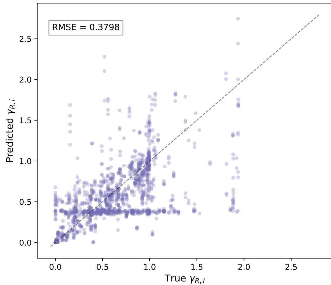
Rank-1 Holdout Predictions
