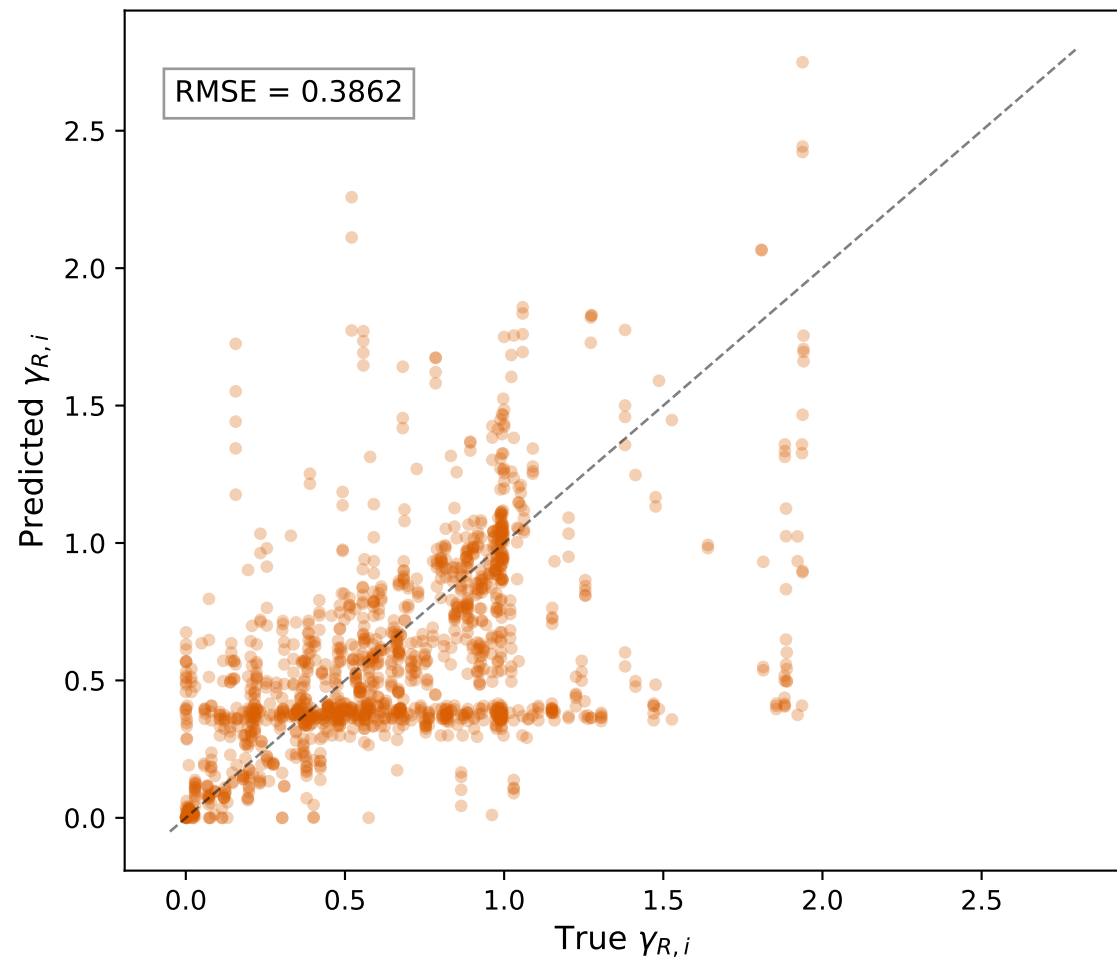
Rank-3 Holdout Predictions
