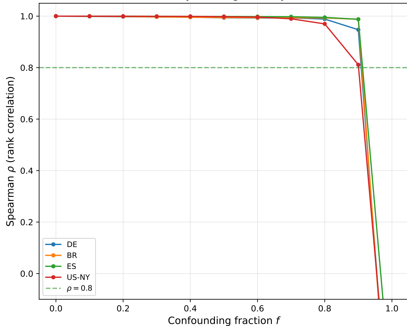
Policy Ranking Stability
