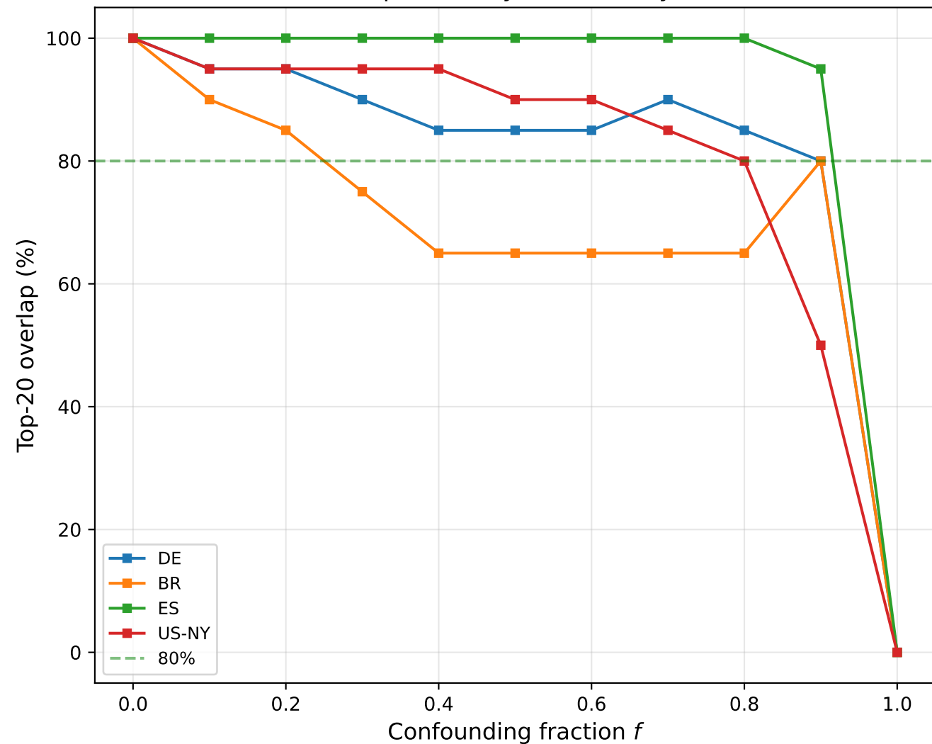
Top-20 Policy Set Stability
