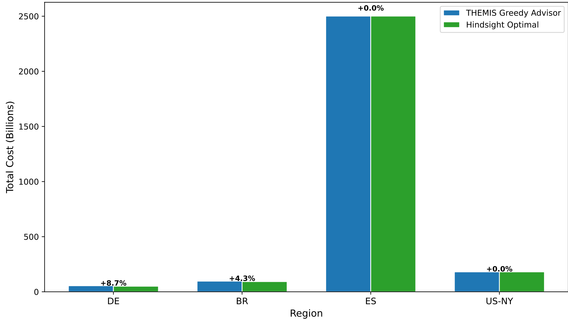
Rolling Greedy Advisor vs Hindsight-Optimal Policy
