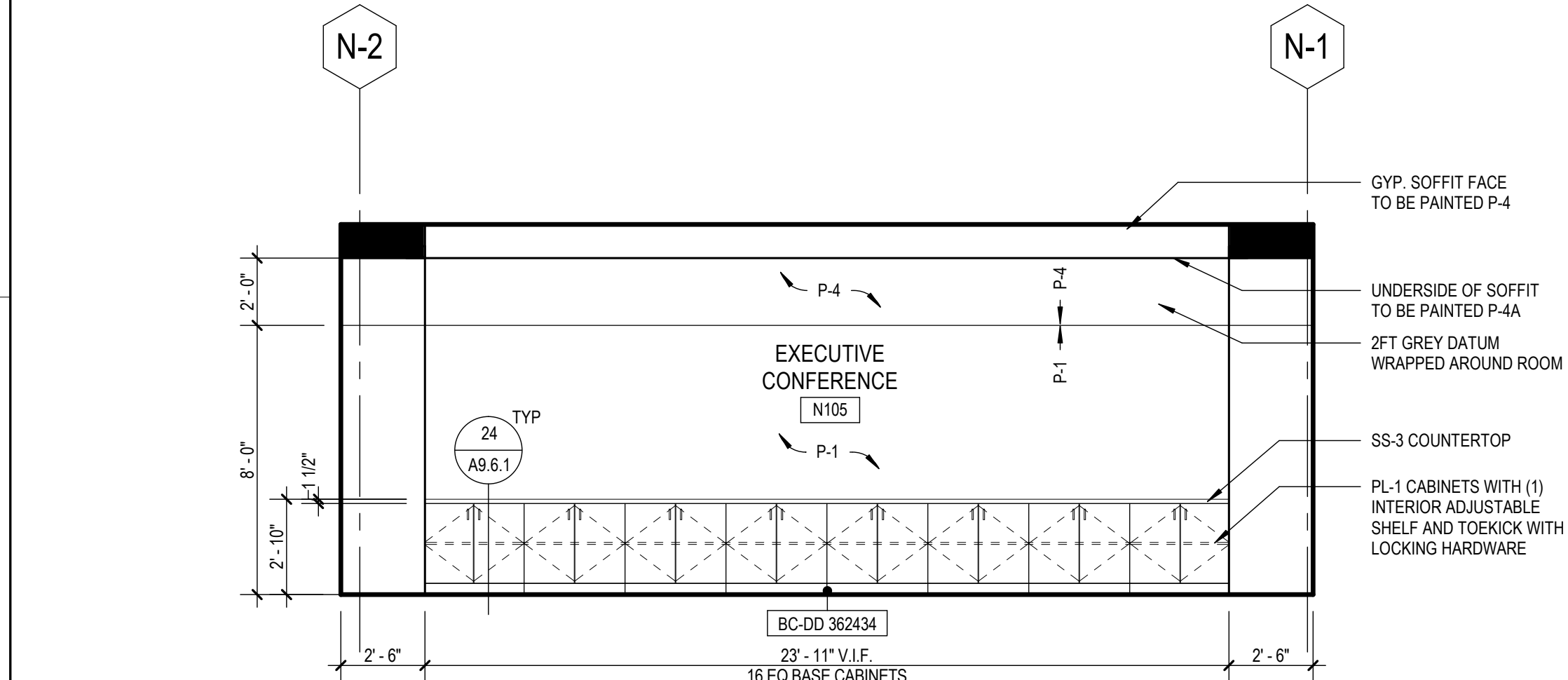
68 EXECUTIVE CONFERENCE ROOM - EAST ELEVATION
