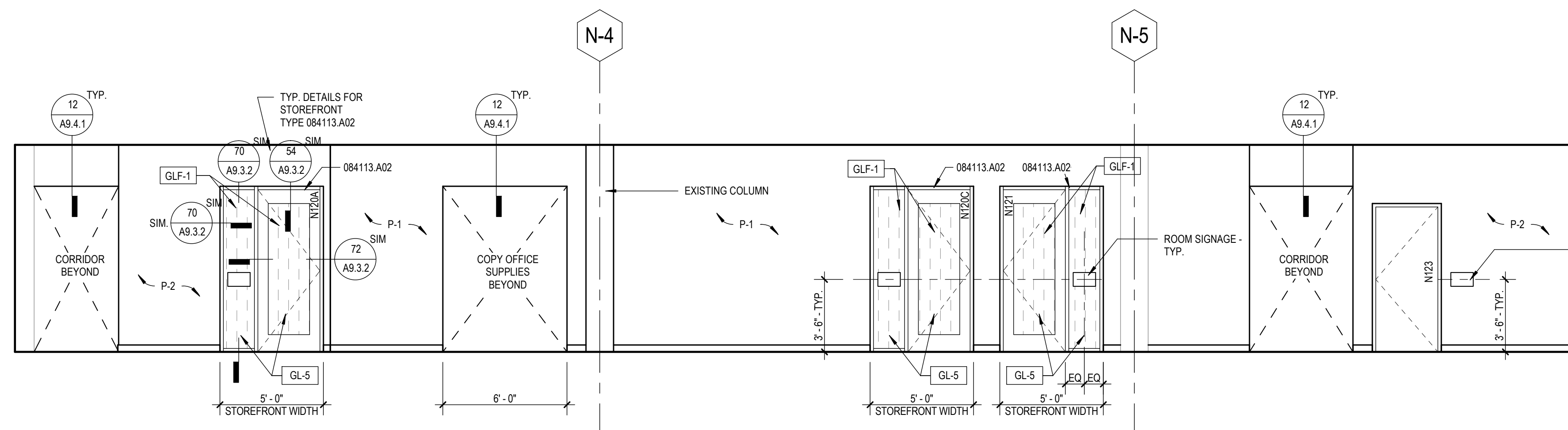
66 UCCS OFFICES - WEST ELEVATION SCALE: 1/4" = 1'-0"
