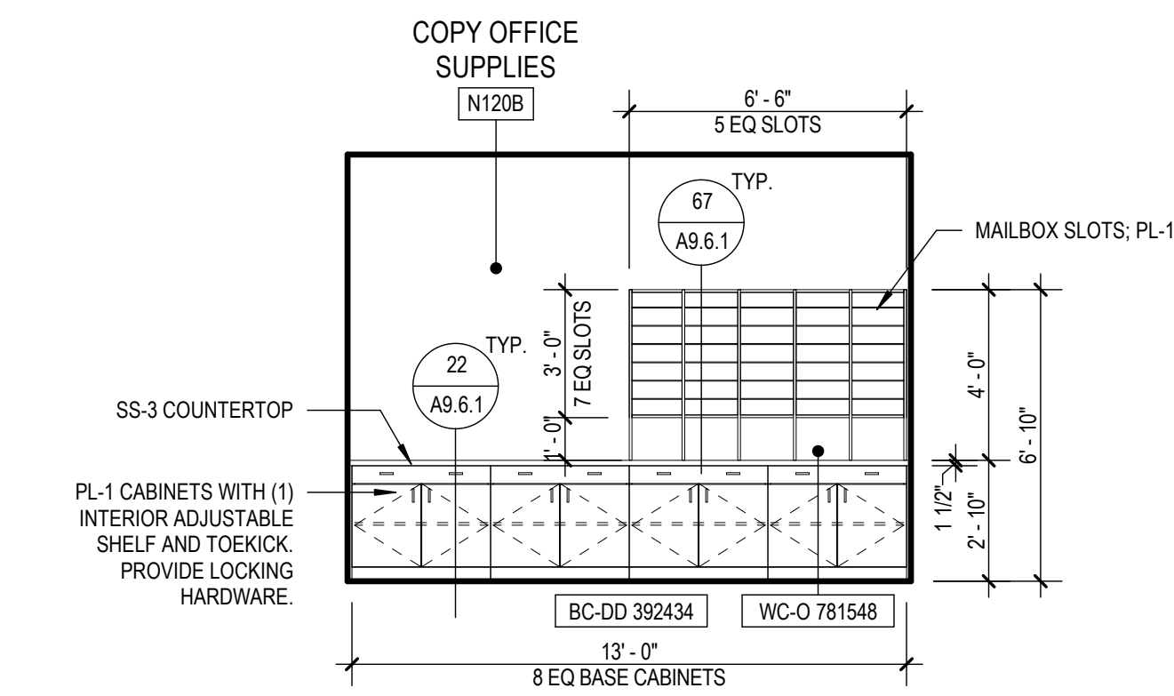
18 COPY OFFICE SUPPLIES - SOUTH ELEVATION SCALE: 1/4" = 1'-0"
