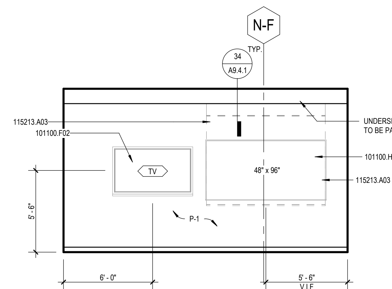
20 LARGE RESEARCH GRAD LABS - TEACHING WALL ELEVATION SCALE: 1/4" = 1'-0"
