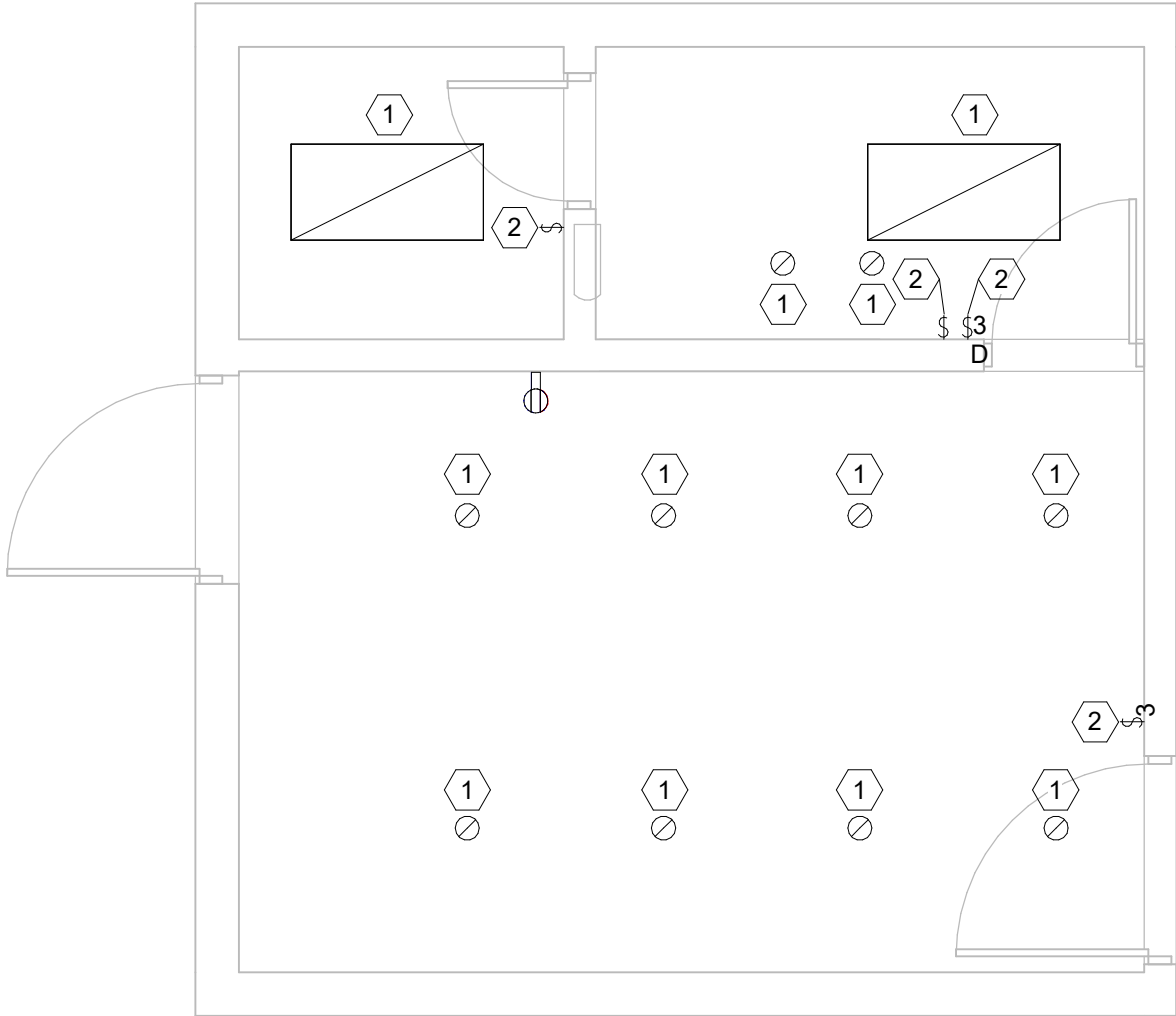
1 ELECTRICAL DEMOLITION 1/4" = 1'-0"
