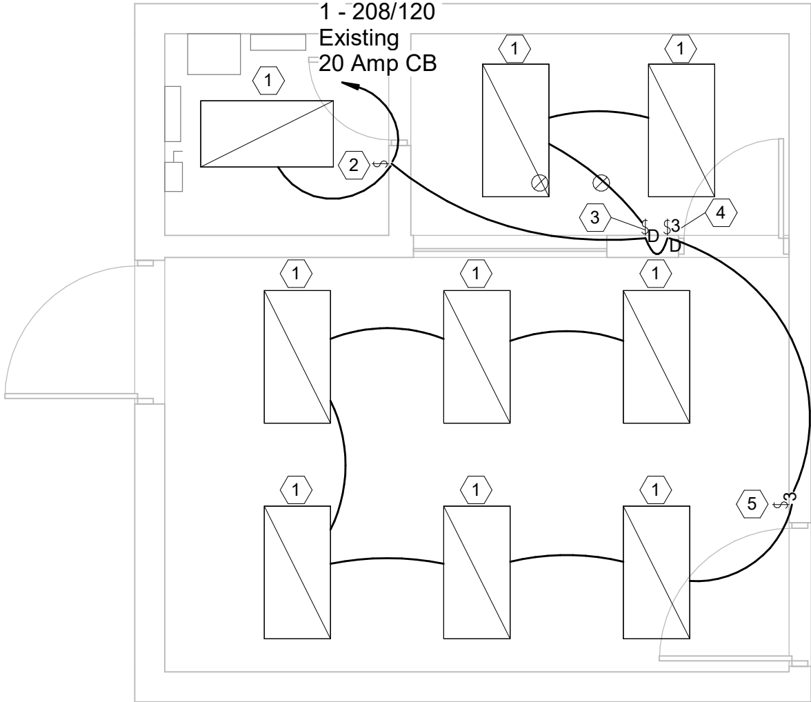
1 ELECTRICAL INSTALLATION 1/4" = 1'-0"
