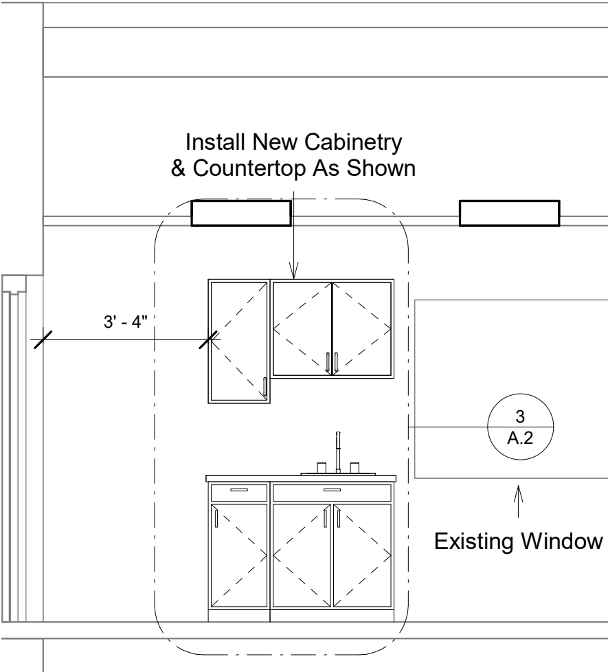
① North Wall Cabinets Copy 1 3/8" = 1'-0"
