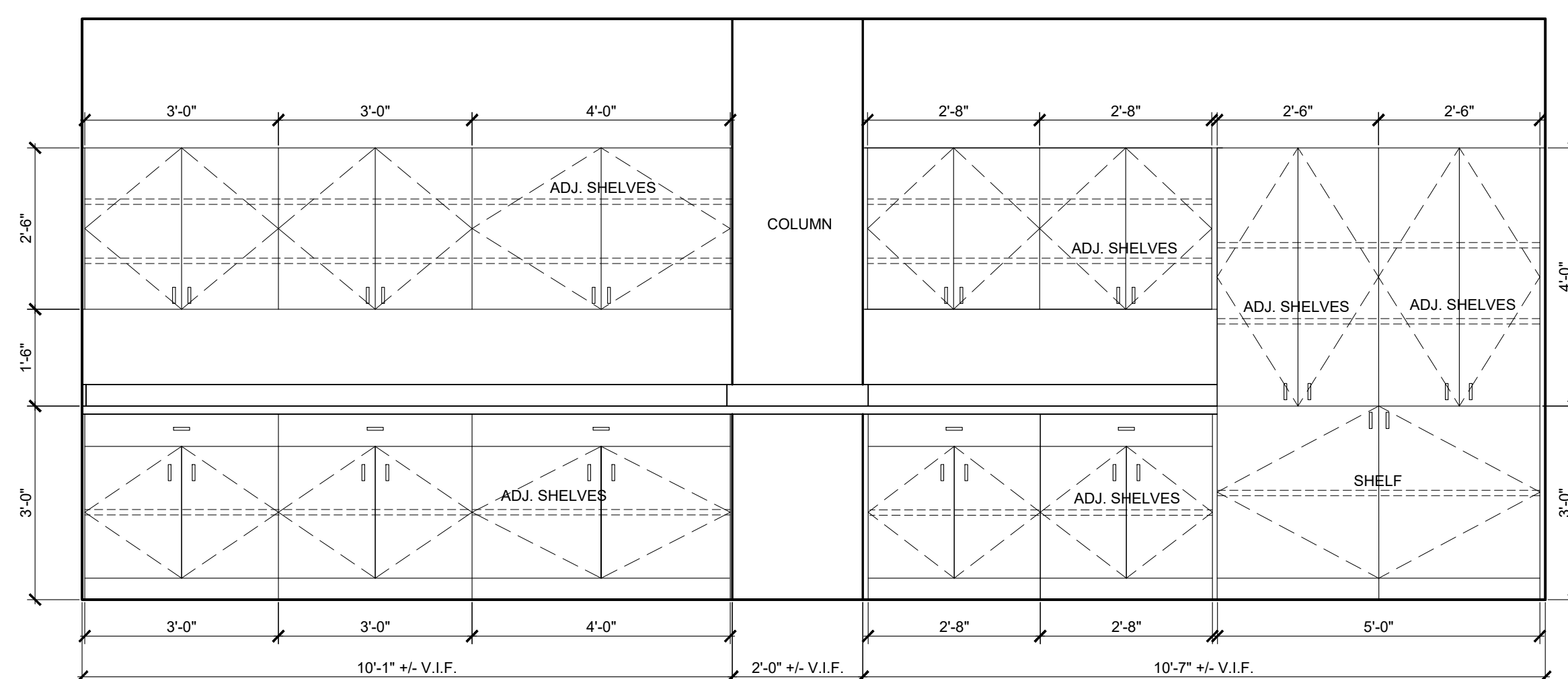
7 MRI SCAN ROOM 107 AE401 SCALE: 1/2" = 1'-0"
