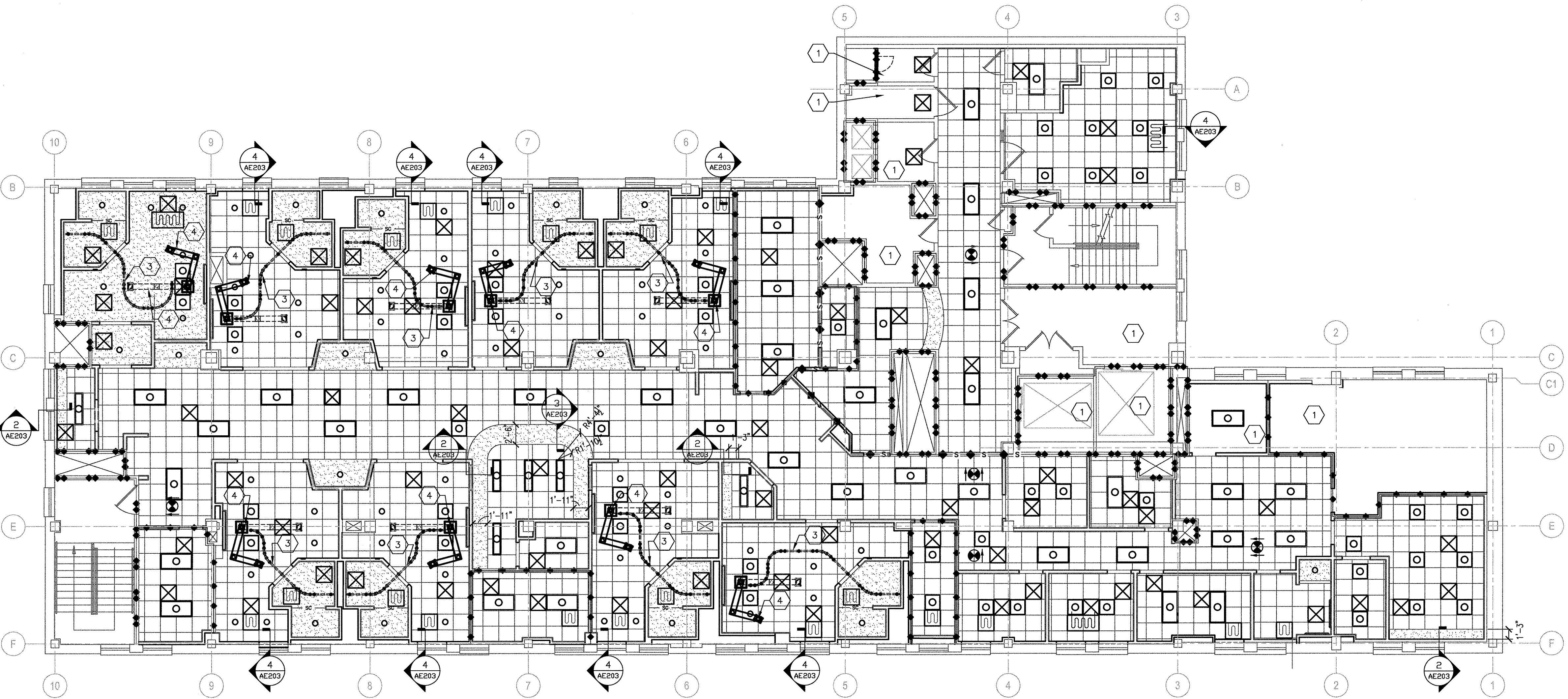
F1 FIFTH FLOOR REFLECTED CEILING PLAN SCALE 1/8" = 1'-0"
