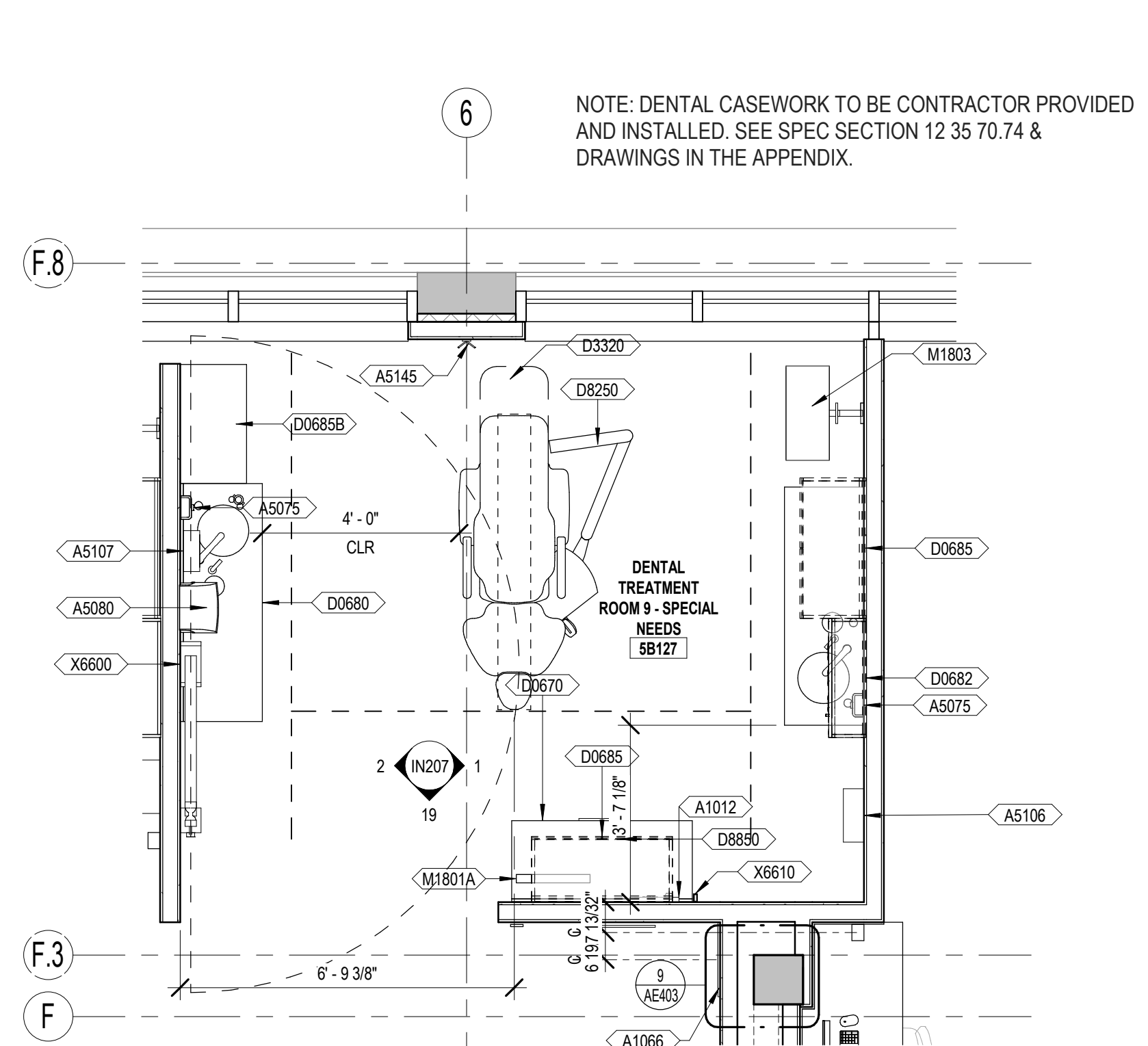
5 DENTAL TREATMENT ROOM 9 - SPECIAL NEEDS
