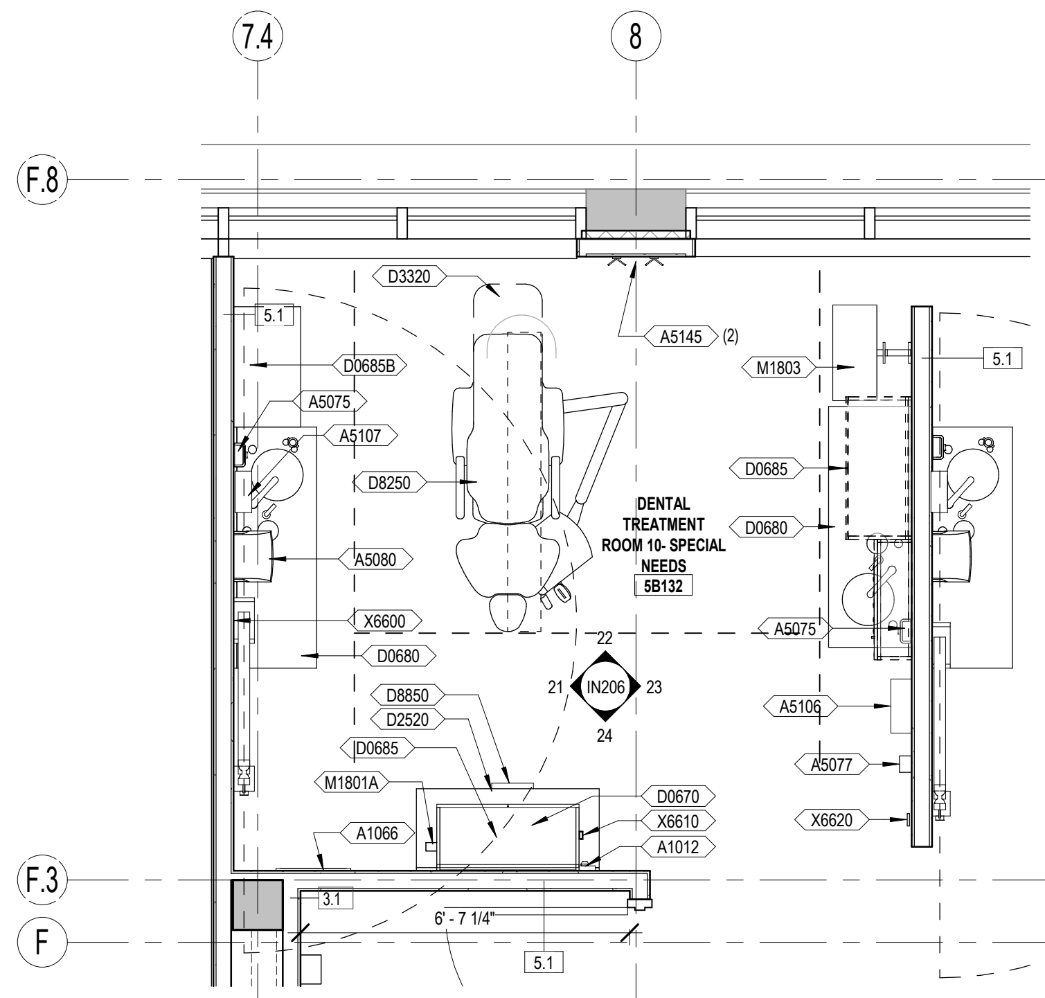
3 DENTAL TREATMENT ROOM 10 - SPECIAL NEEDS
