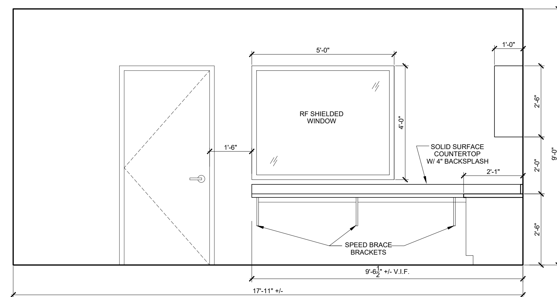
6 CONTROL ROOM 105 AE401 SCALE: 1/2" = 1'-0"
