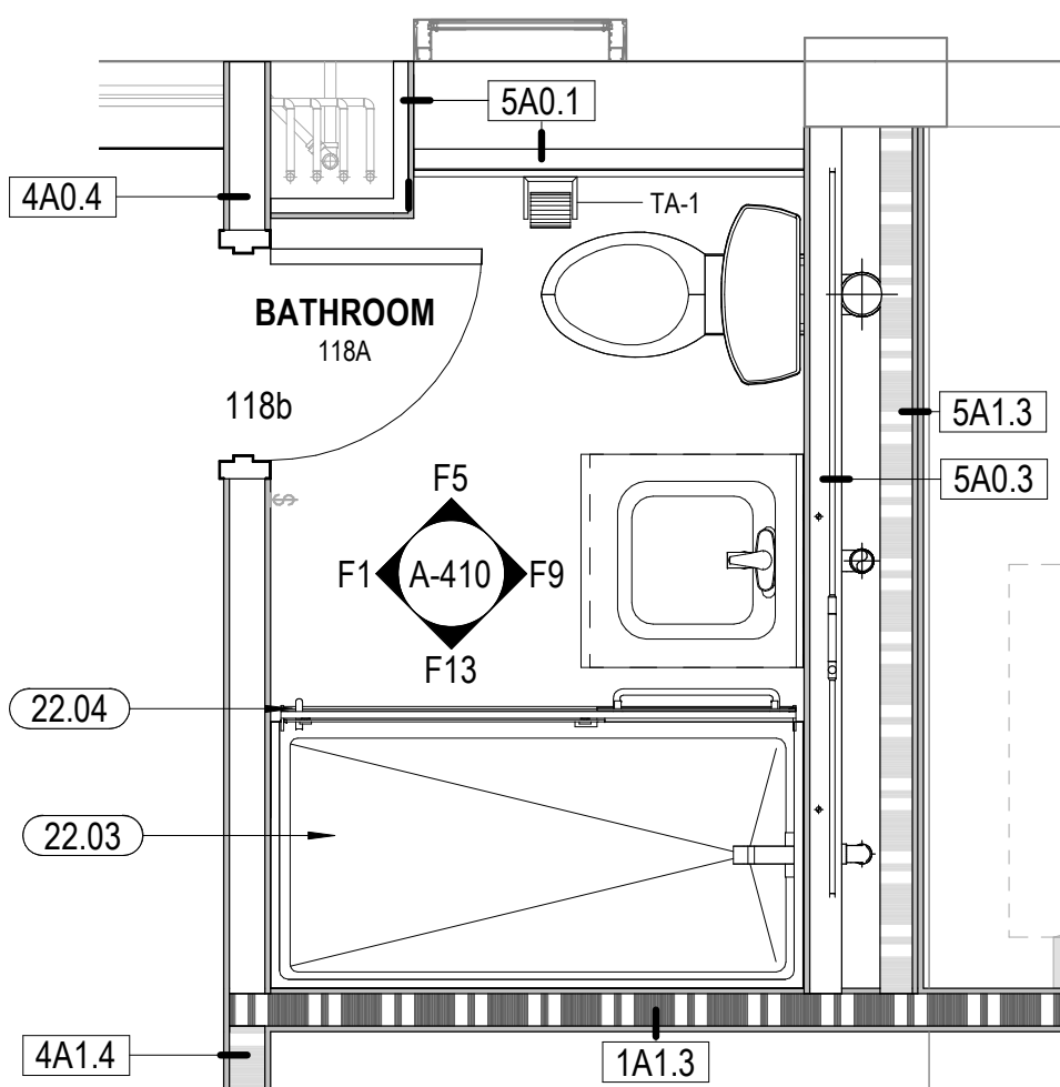
A1 BATHROOM - 1ST/2ND/3RD FL - RM 118A, 218A, 318A 1/2" = 1'-0"
