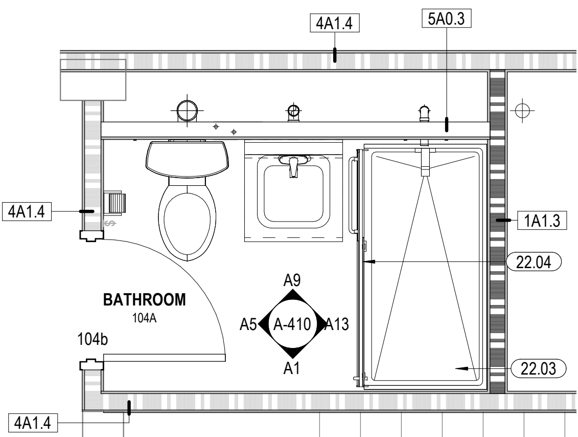
A7 BATHROOM - 1ST/2ND/3RD FL - RM 104A, 204A, 304A 1/2" = 1'-0"
