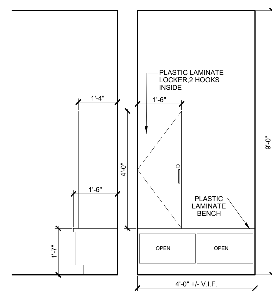
1 DRESS 101 ELEVATION AE401 SCALE: 1/2" = 1'-0"
