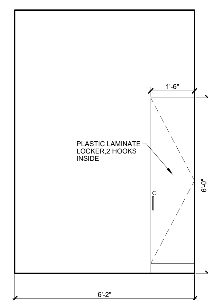
2 DRESS 102 ELEVATION AE401 SCALE: 1/2" = 1'-0"
