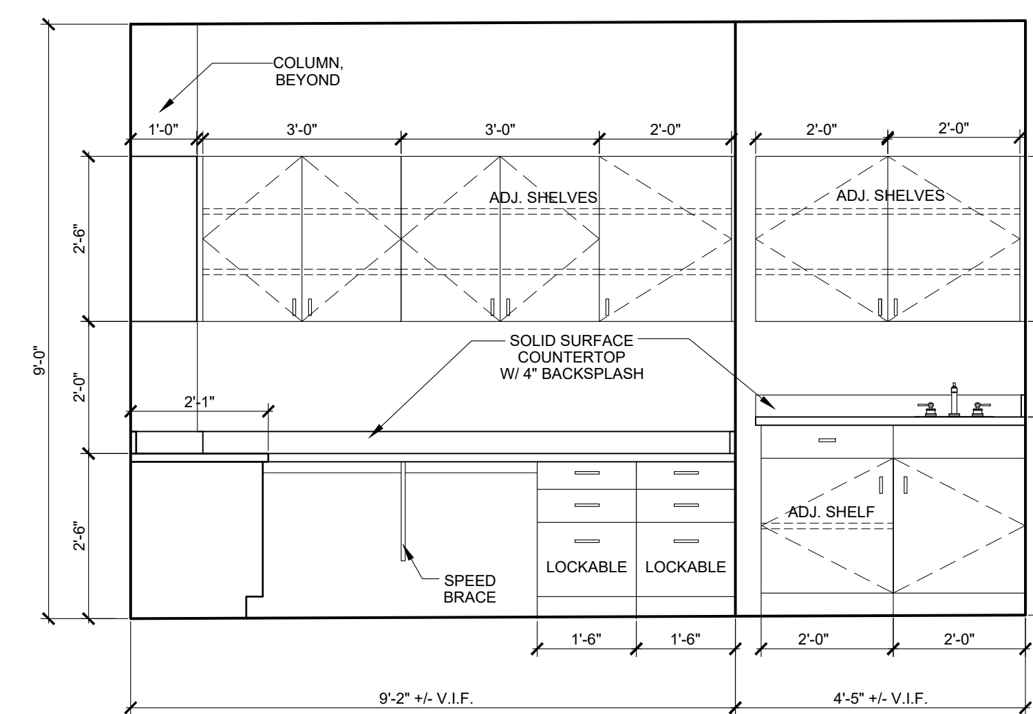
4 CONTROL ROOM 105 AE401 SCALE: 1/2" = 1'-0"
