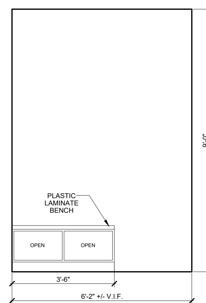
3 DRESS 102 ELEVATION AE401 SCALE: 1/2" = 1'-0"
