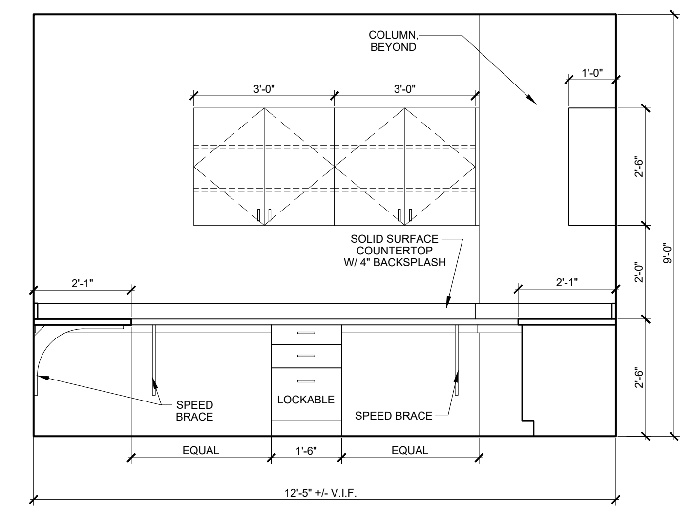
5 CONTROL ROOM 105 AE401 SCALE: 1/2" = 1'-0"
