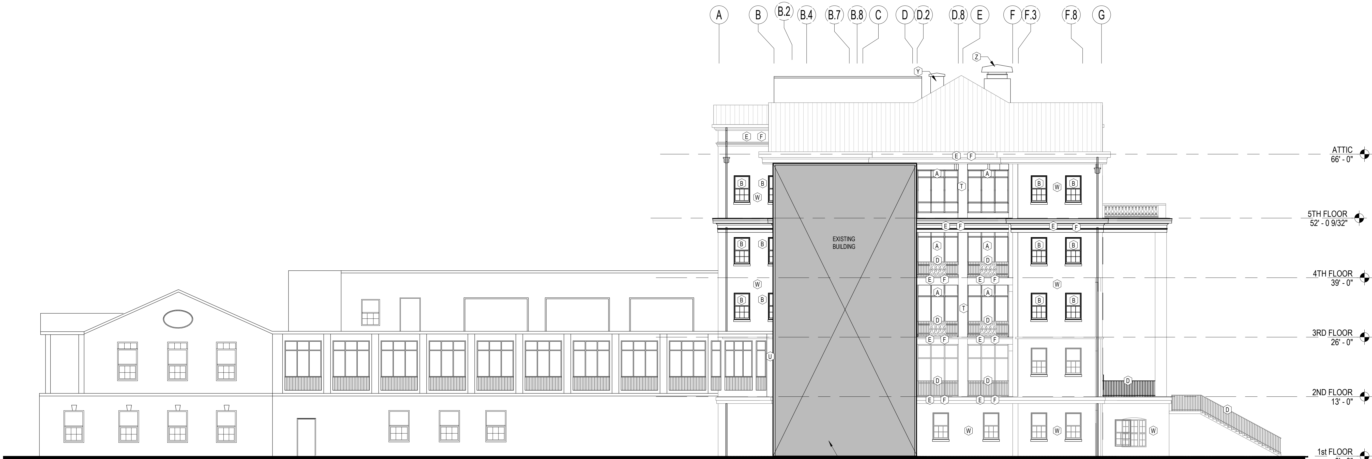
1 NORTH EXTERIOR ELEVATION 3/32" = 1'-0"
