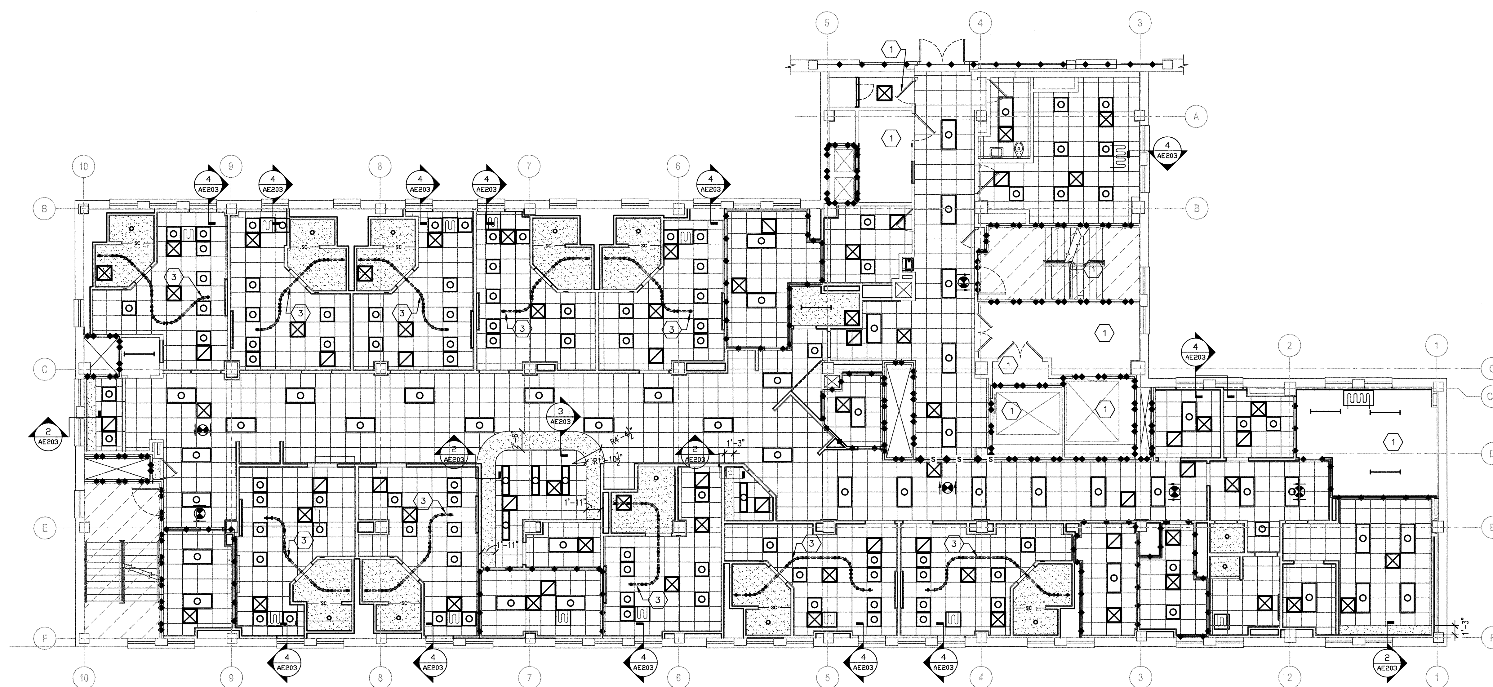
F1 THIRD FLOOR REFLECTED CEILING PLAN SCALE 1/8" = 1'-0"
