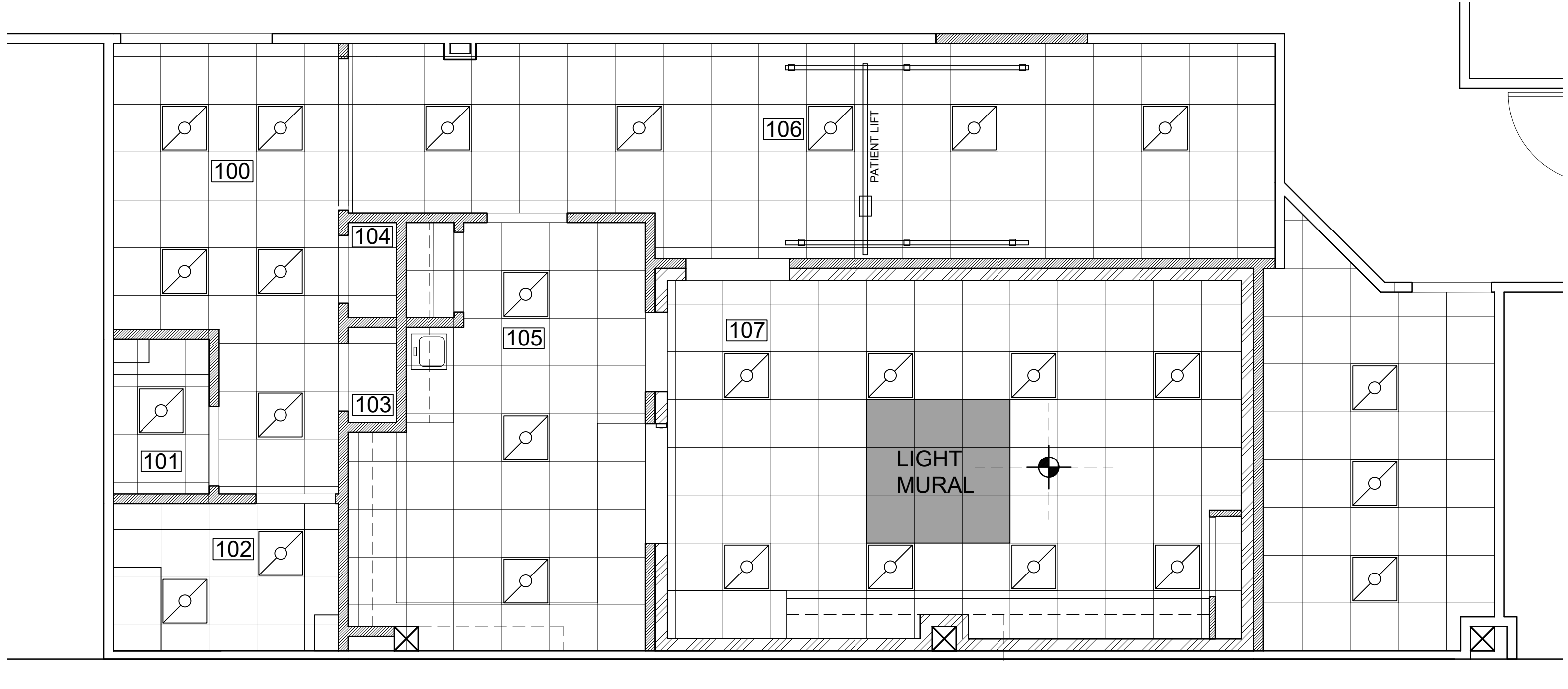
1 REFLECTED CEILING PLAN SCALE: 1/4" = 1'-0"
