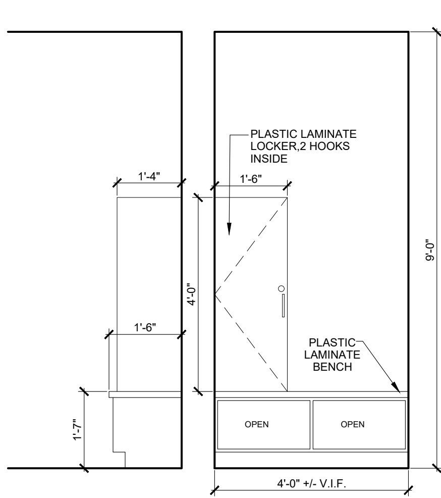
1 DRESS 101 ELEVATION SCALE: 1/2" = 1'-0"
