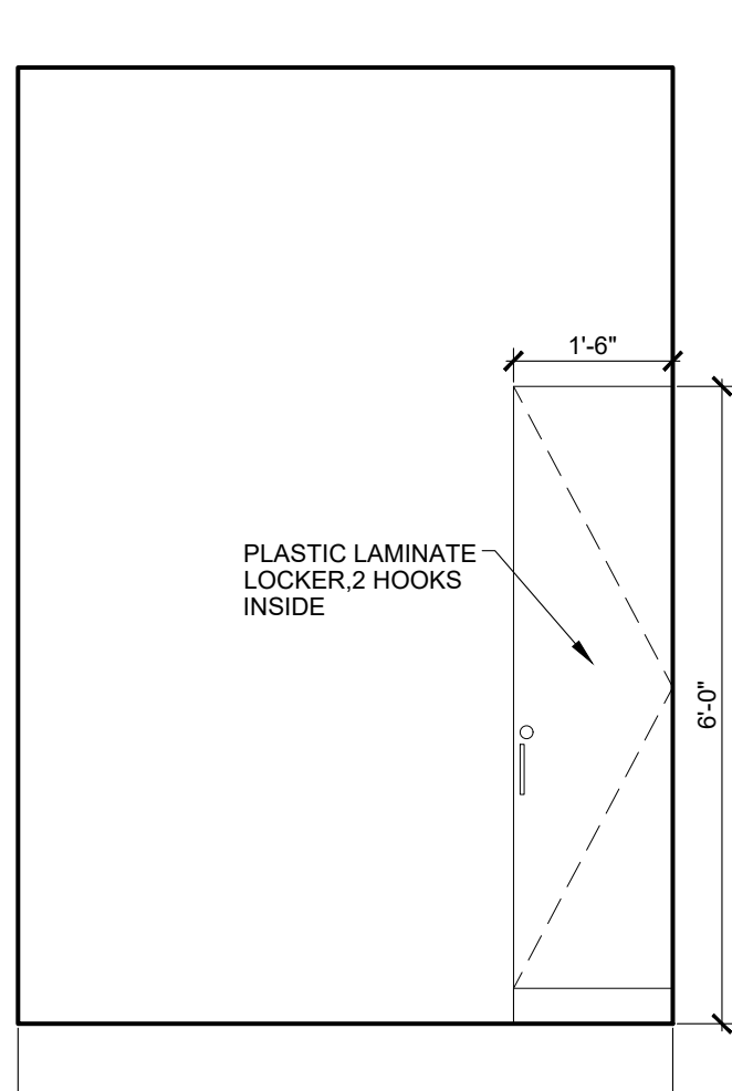
2 DRESS 102 ELEVATION SCALE: 1/2" = 1'-0"
