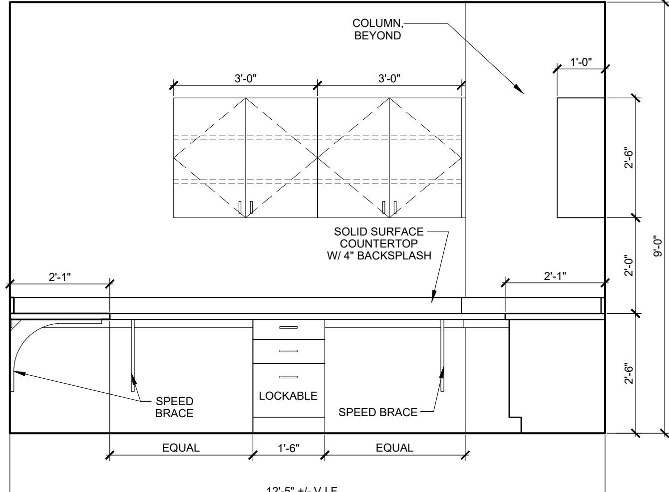
5 CONTROL ROOM 105 SCALE: 1/2" = 1'-0"
