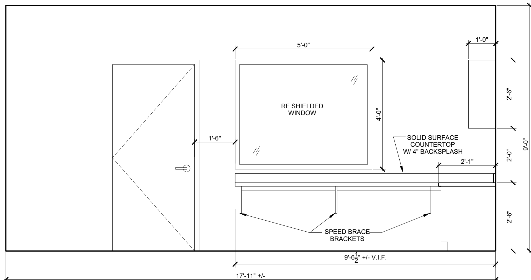
6 CONTROL ROOM 105 SCALE: 1/2" = 1'-0"
