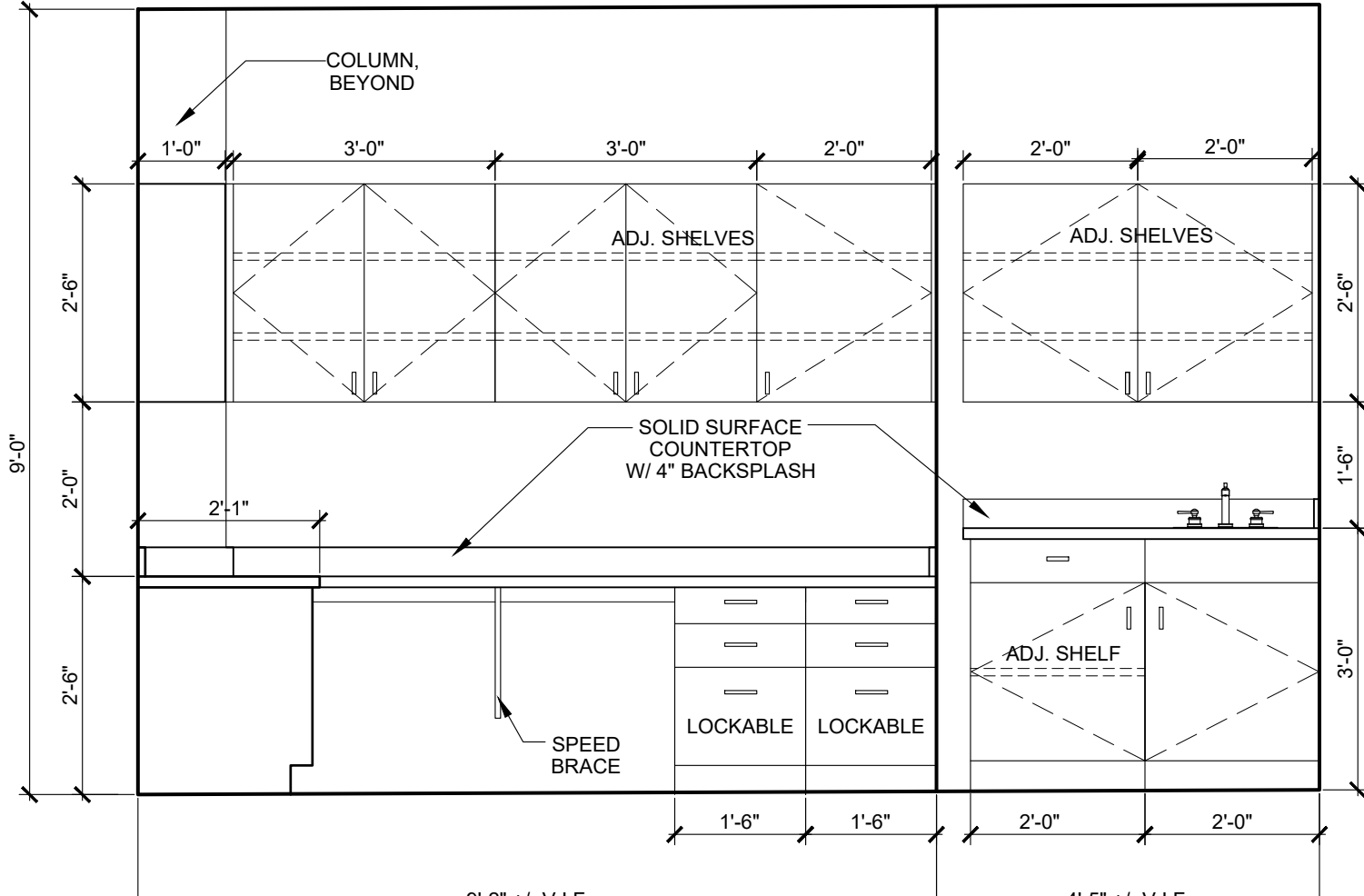
4 CONTROL ROOM 105 SCALE: 1/2" = 1'-0"
