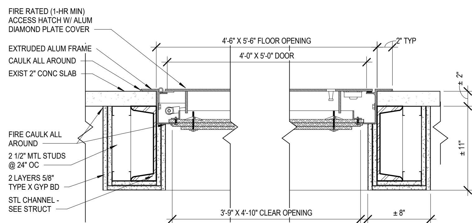
3 ACCESS HATCH DETAIL AE110/ 1 1/2" = 1'-0"
