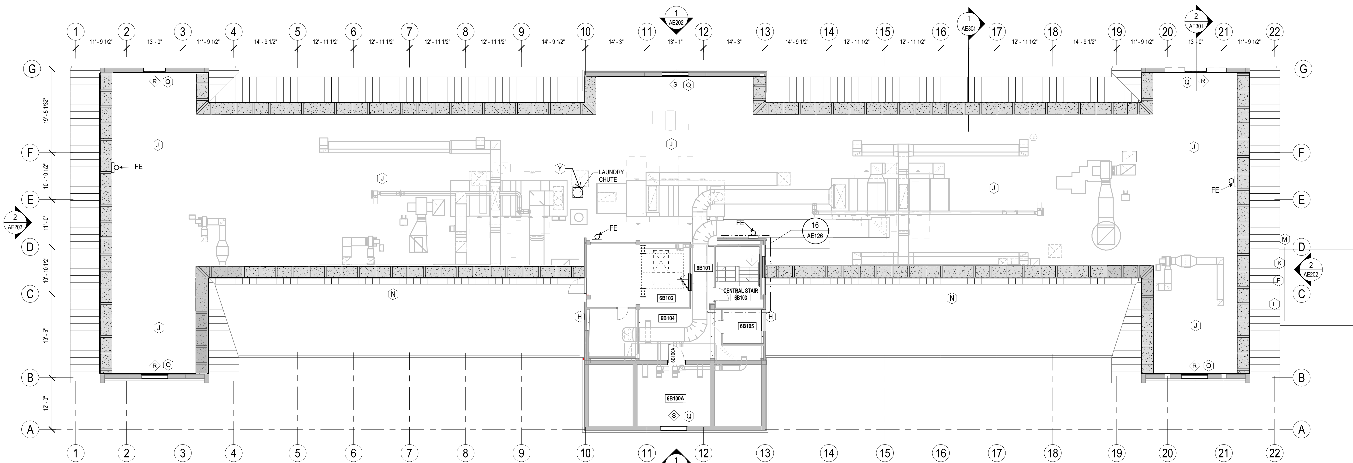
2 ATTIC PLAN 3/32" = 1'-0"
