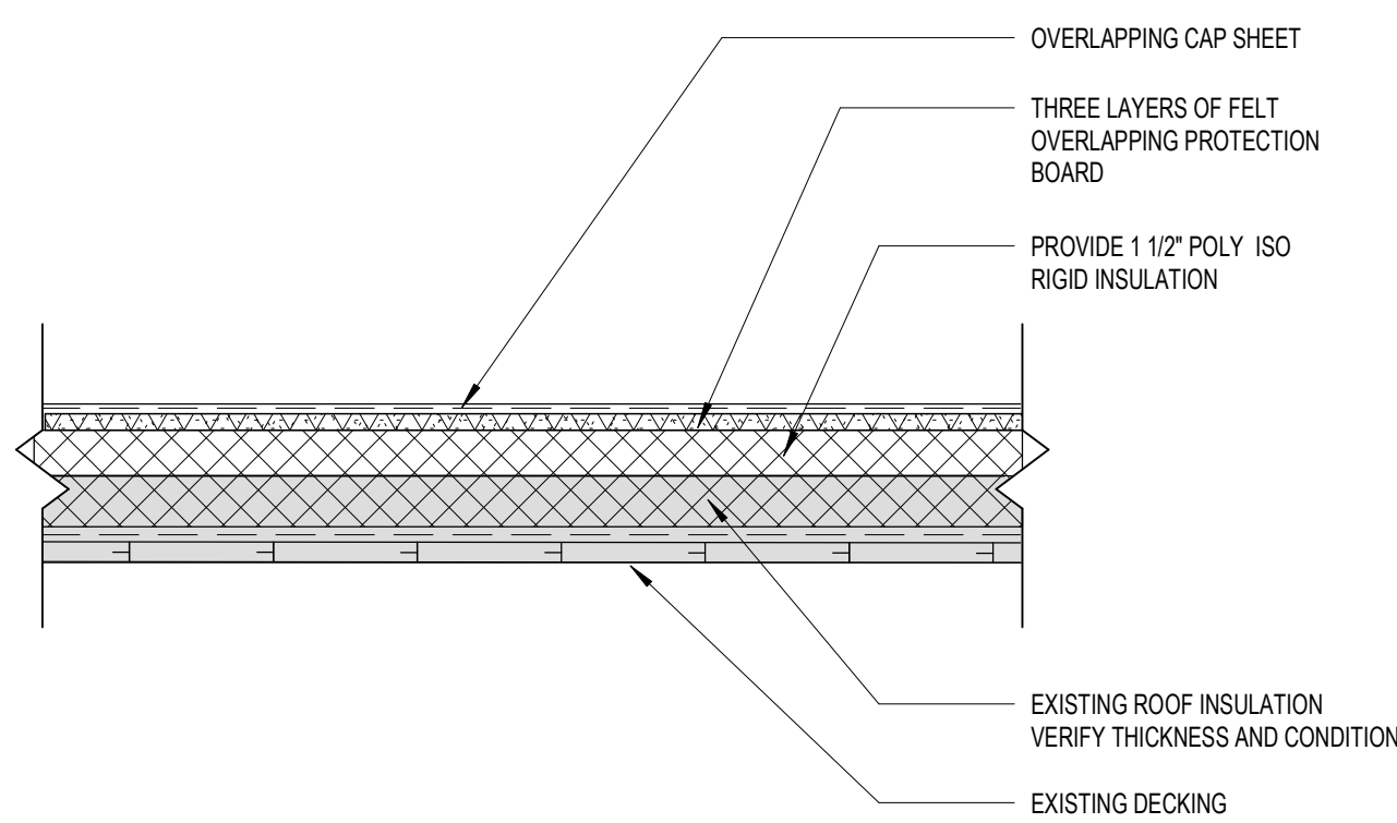
4 MODIFIED - BITUMEN ROOF TYPE 3 AE106/ 1 1/2" = 1'-0"
