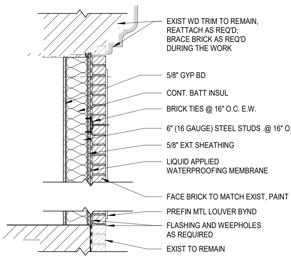
2 BRICK INFILL DETAIL AE110/ 3/4" = 1'-0"
