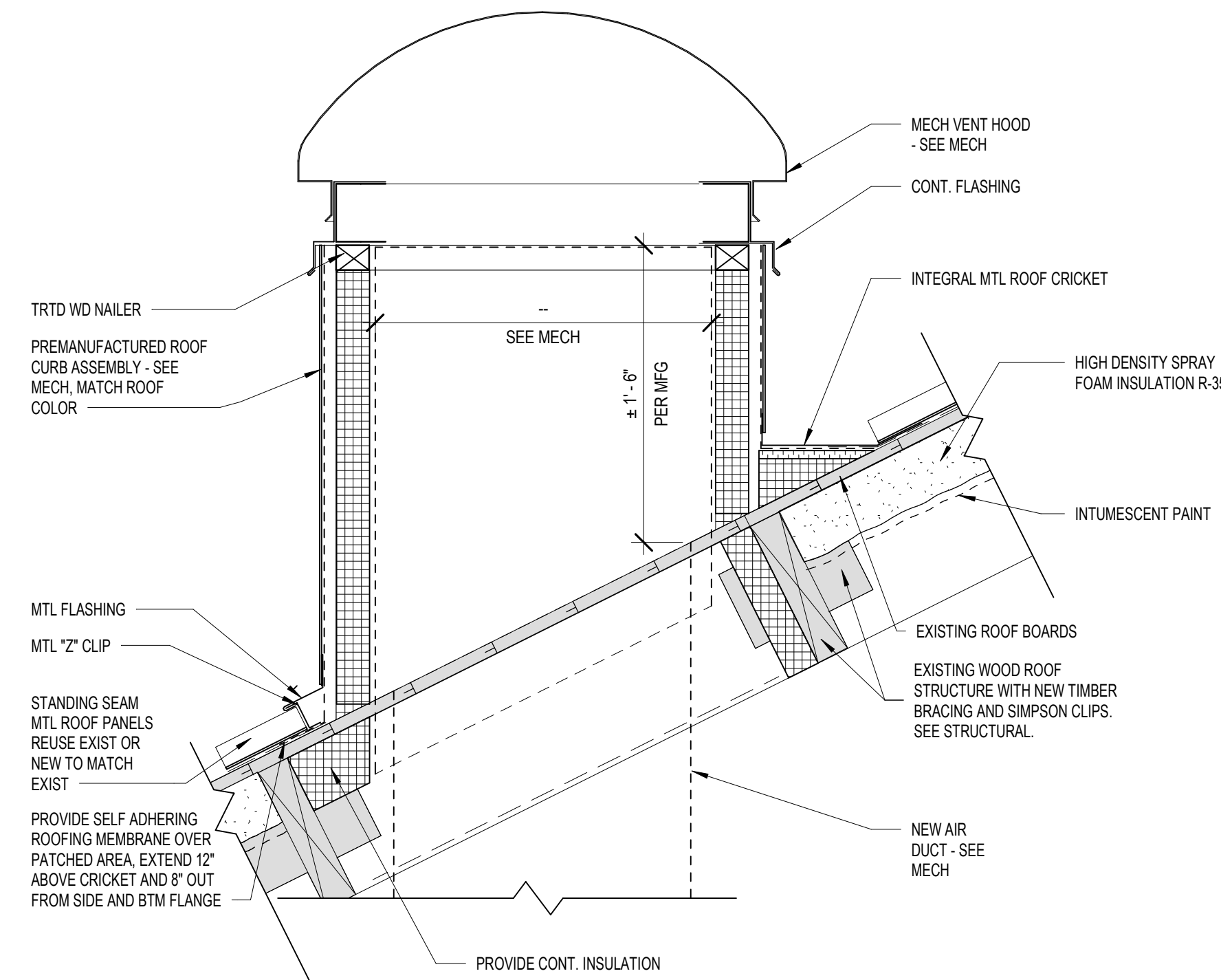
5 ROOF HOOD DETAIL AE106/ 1 1/2" = 1'-0"
