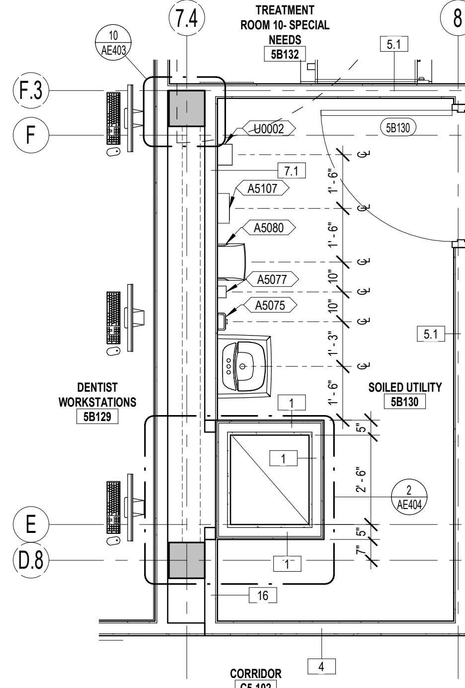
6 ENLARGED FLOOR PLAN AE125 3/8" = 1'-0"
