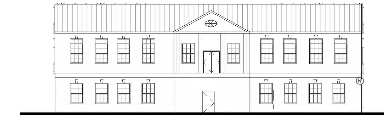
3 SOUTH ELEVATION AE203 3/32" = 1'-0"
