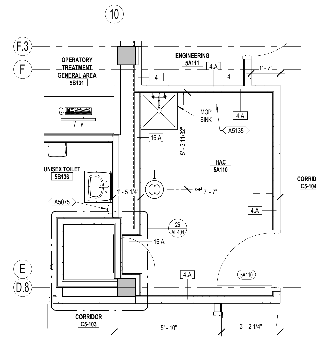
5 ENLARGED FLOOR PLAN AE125 3/8" = 1'-0"
