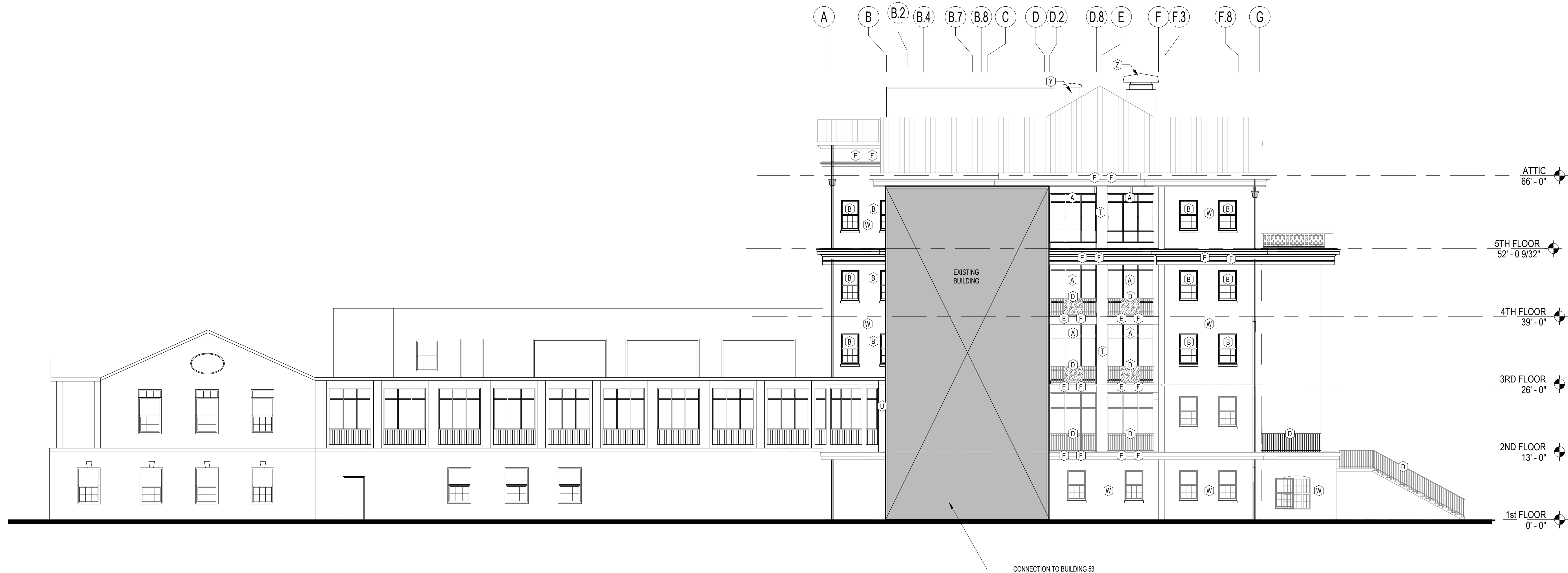
2 EAST EXTERIOR ELEVATION 3/32" = 1'-0"
