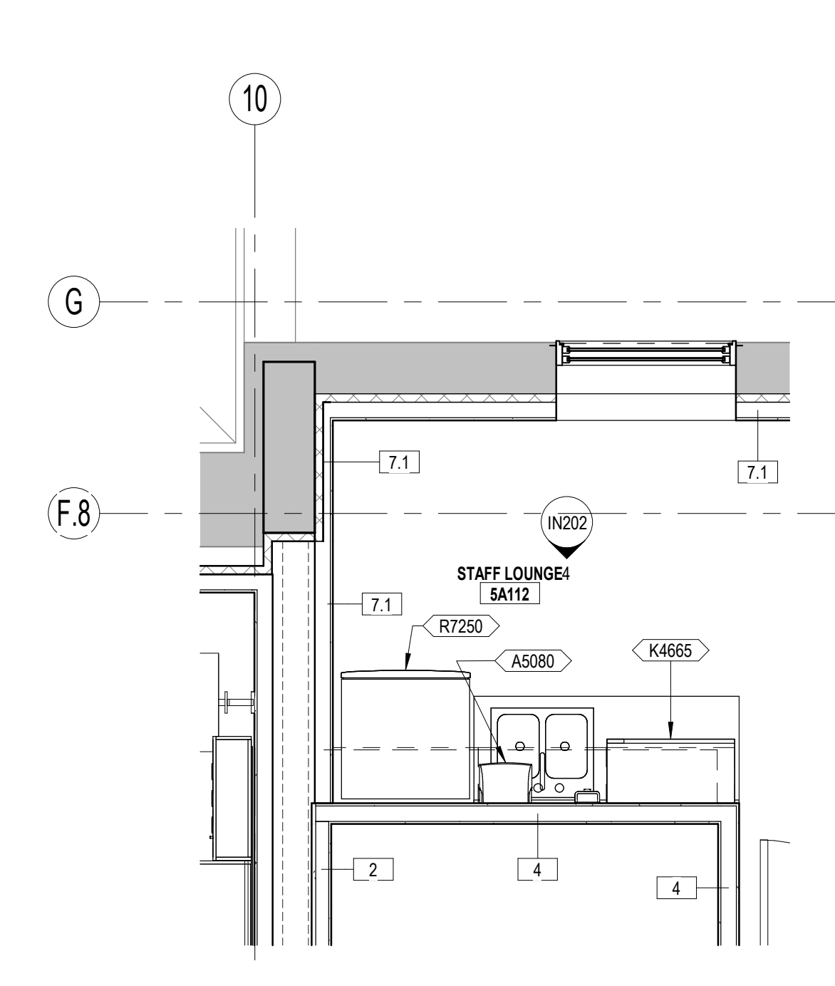
7 ENLARGED FLOOR PLAN AE125 3/8" = 1'-0"
