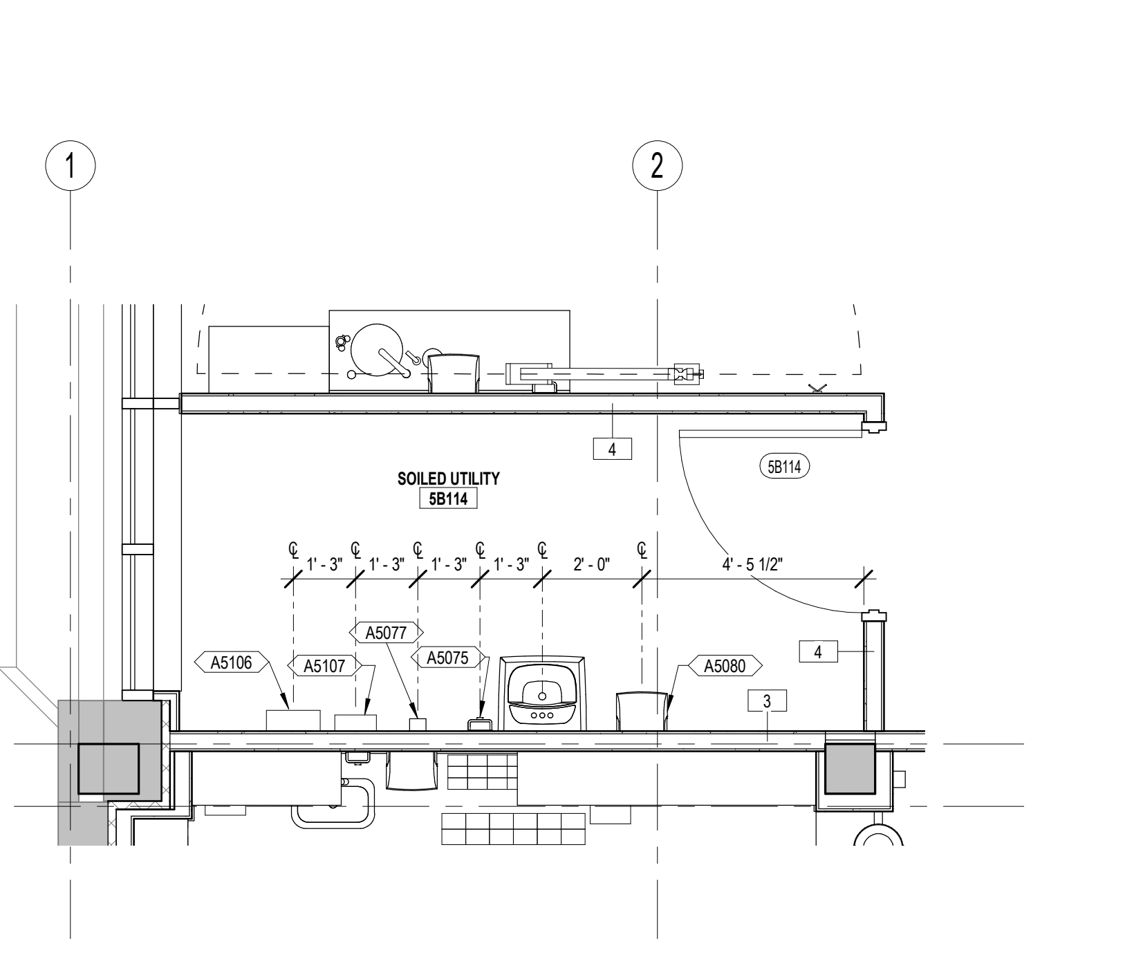
8 ENLARGED FLOOR PLAN AE125 3/8" = 1'-0"
