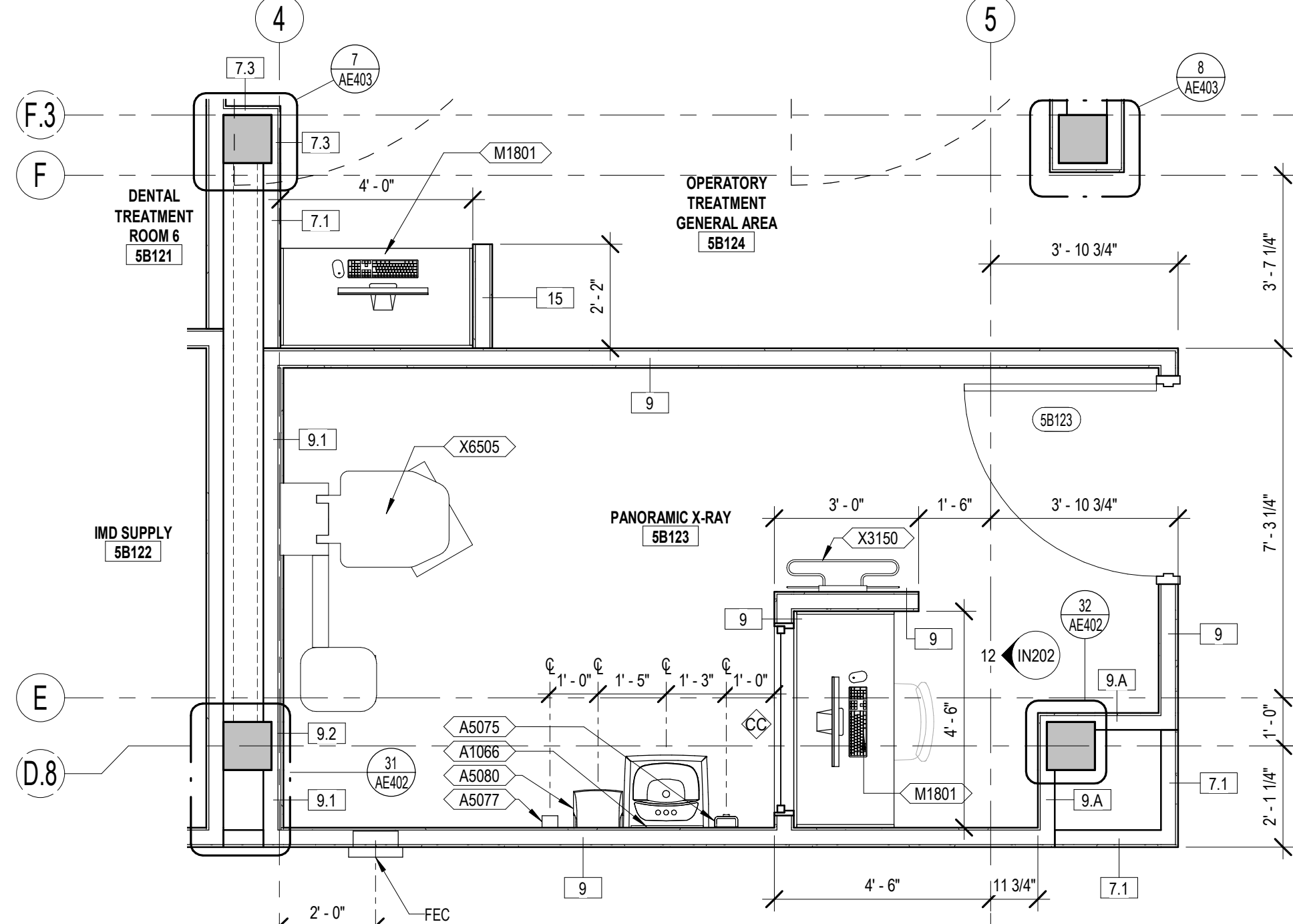
2 ENLARGED FLOOR PLAN AE125 3/8" = 1'-0"
