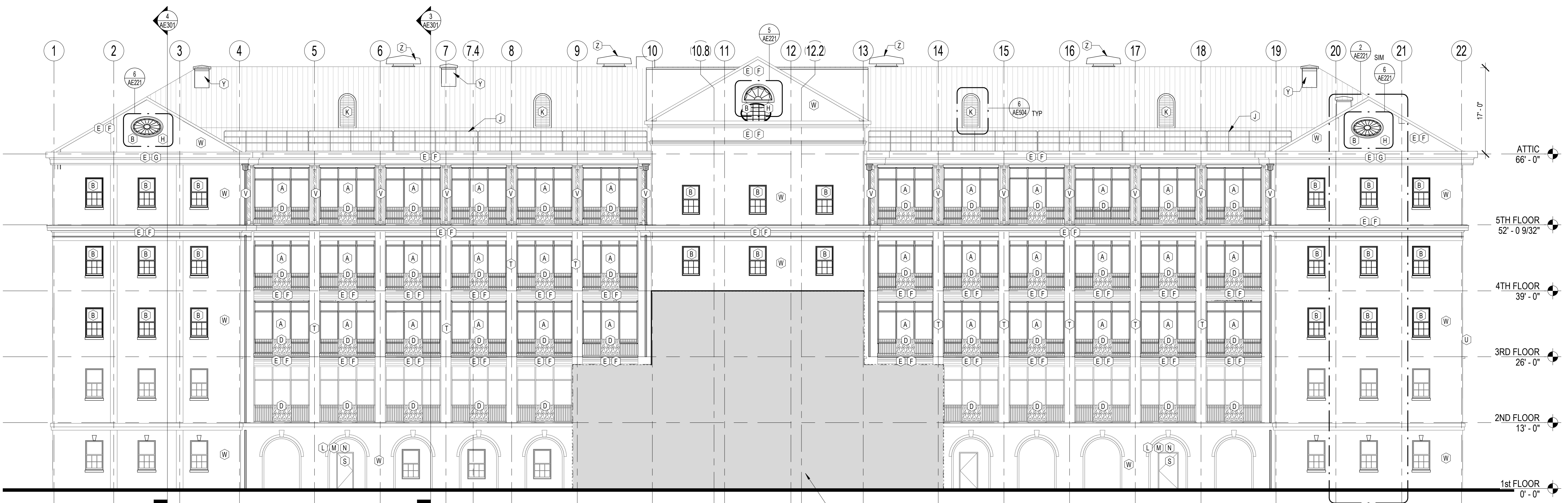
1 SOUTH EXTERIOR ELEVATION AE203 3/32" = 1'-0"
