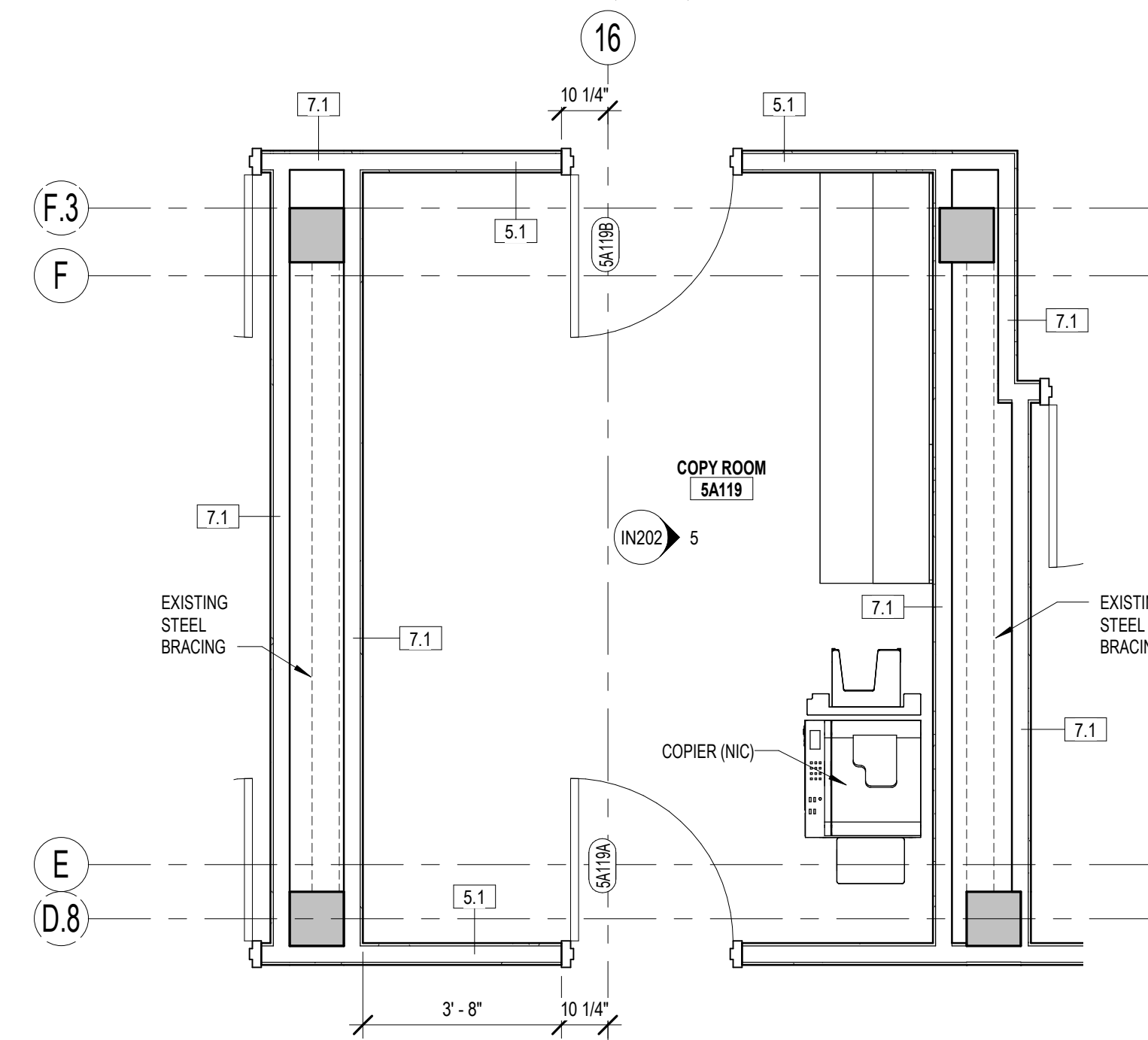
10 ENLARGED FLOOR PLAN AE125 3/8" = 1'-0"
