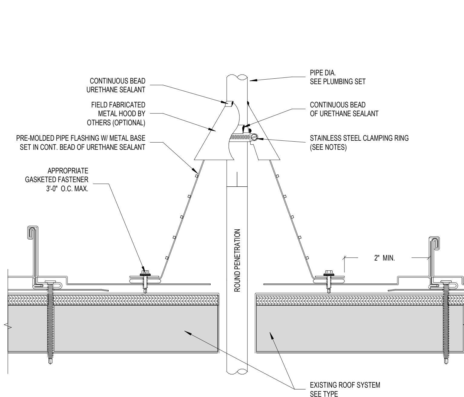
6 VENT THRU METAL ROOF AE106/ 6" = 1'-0"
