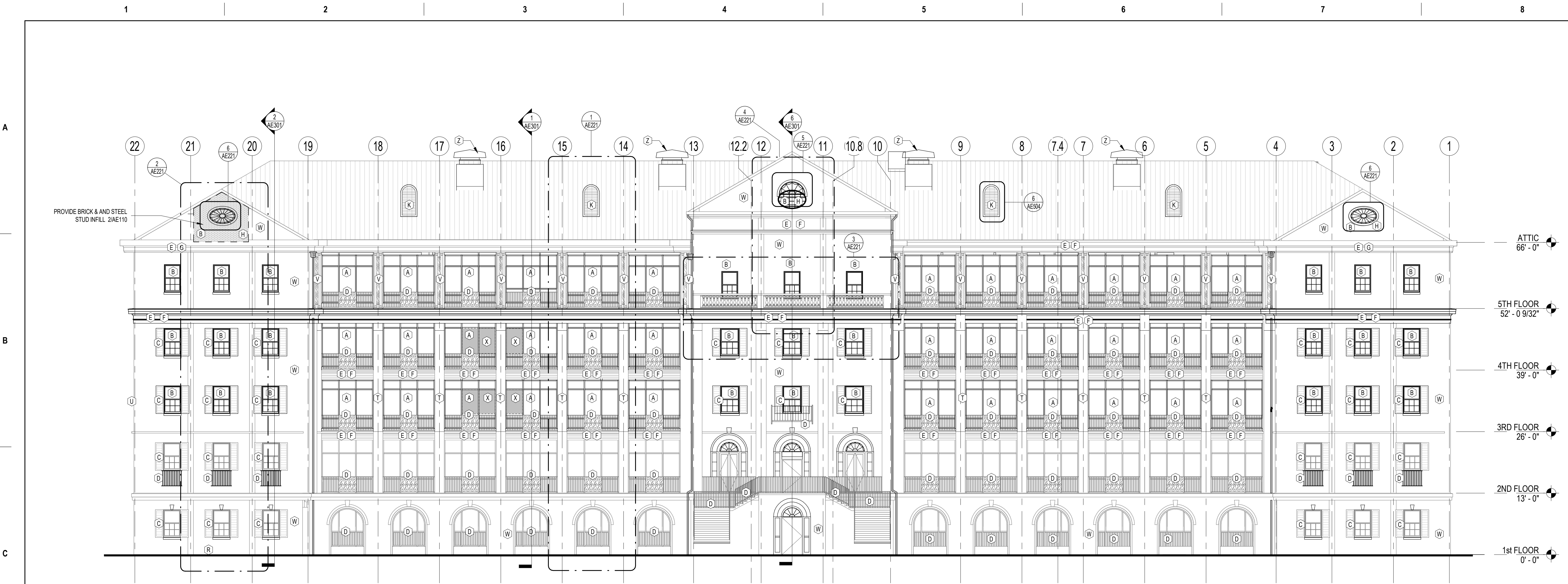
1 NORTH EXTERIOR ELEVATION 3/32" = 1'-0"
