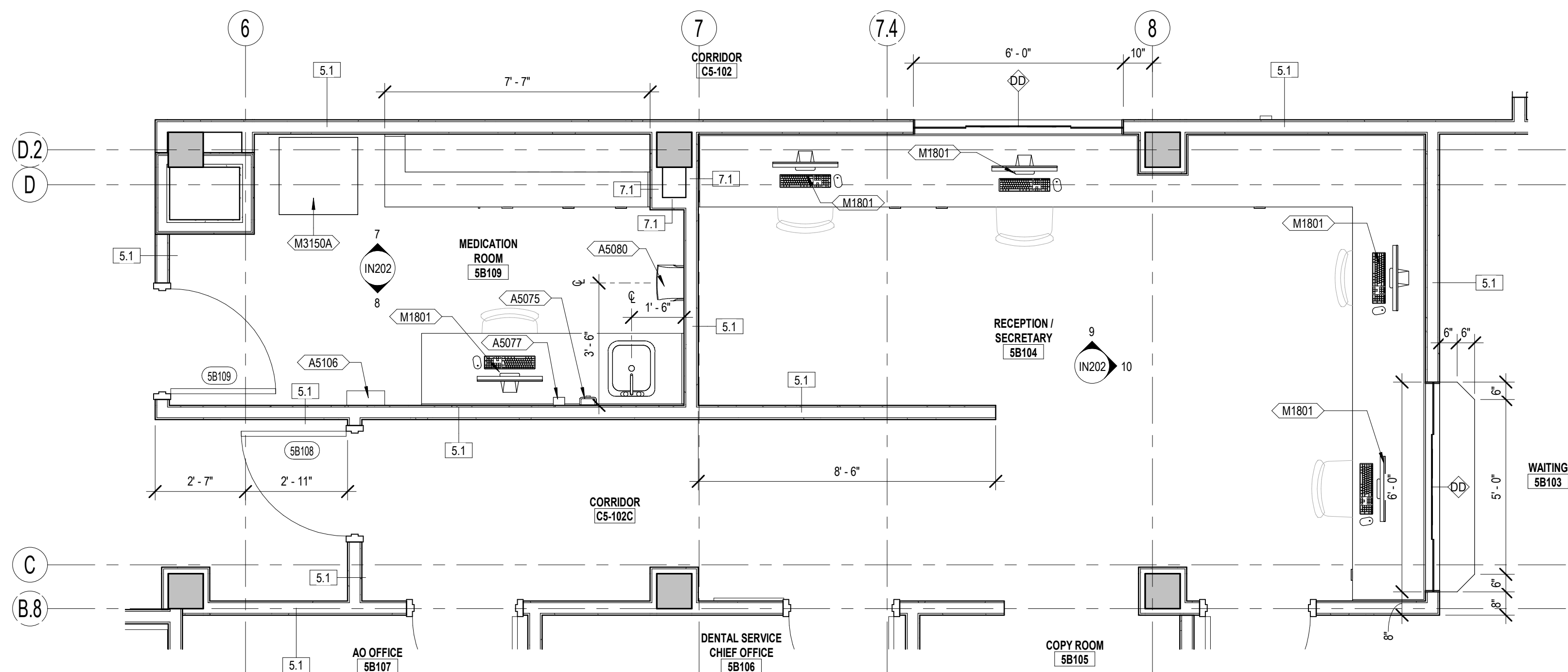
1 ENLARGED FLOOR PLAN AE125 3/8" = 1'-0"
