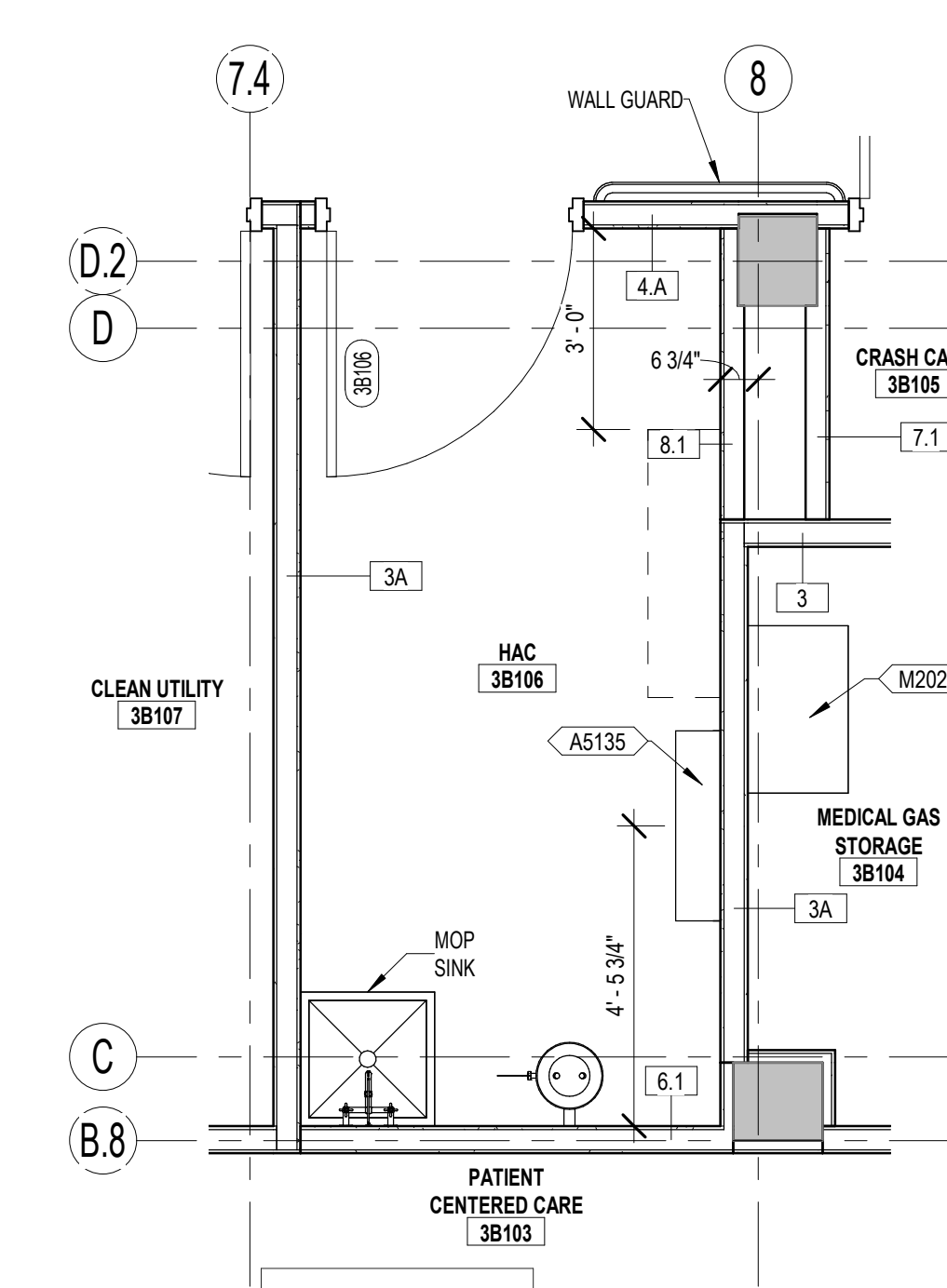
4 ENLARGED FLOOR PLAN AE125 3/8" = 1'-0"
