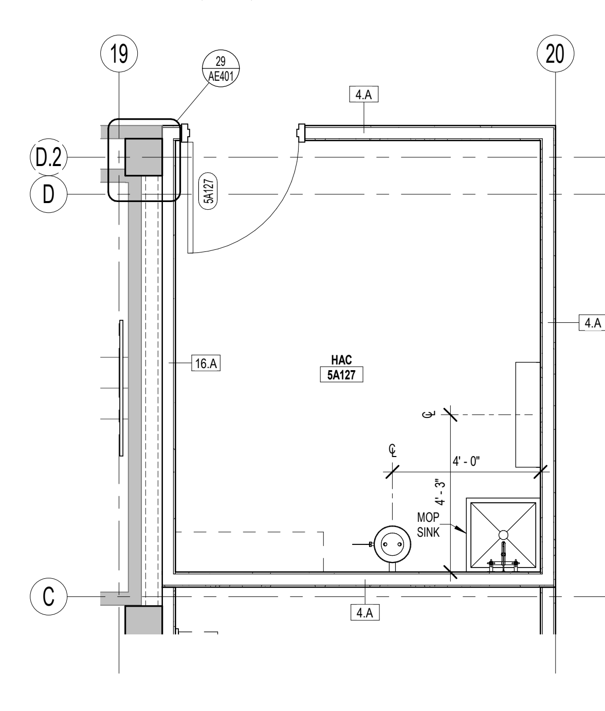
11 ENLARGED FLOOR PLAN AE125 3/8" = 1'-0"
