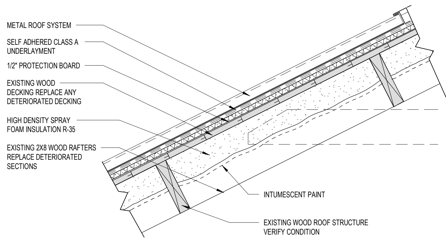
2 METAL ROOF TYPE 1 - BASE BID CONSTRUCTION AE106/ 1 1/2" = 1'-0"
