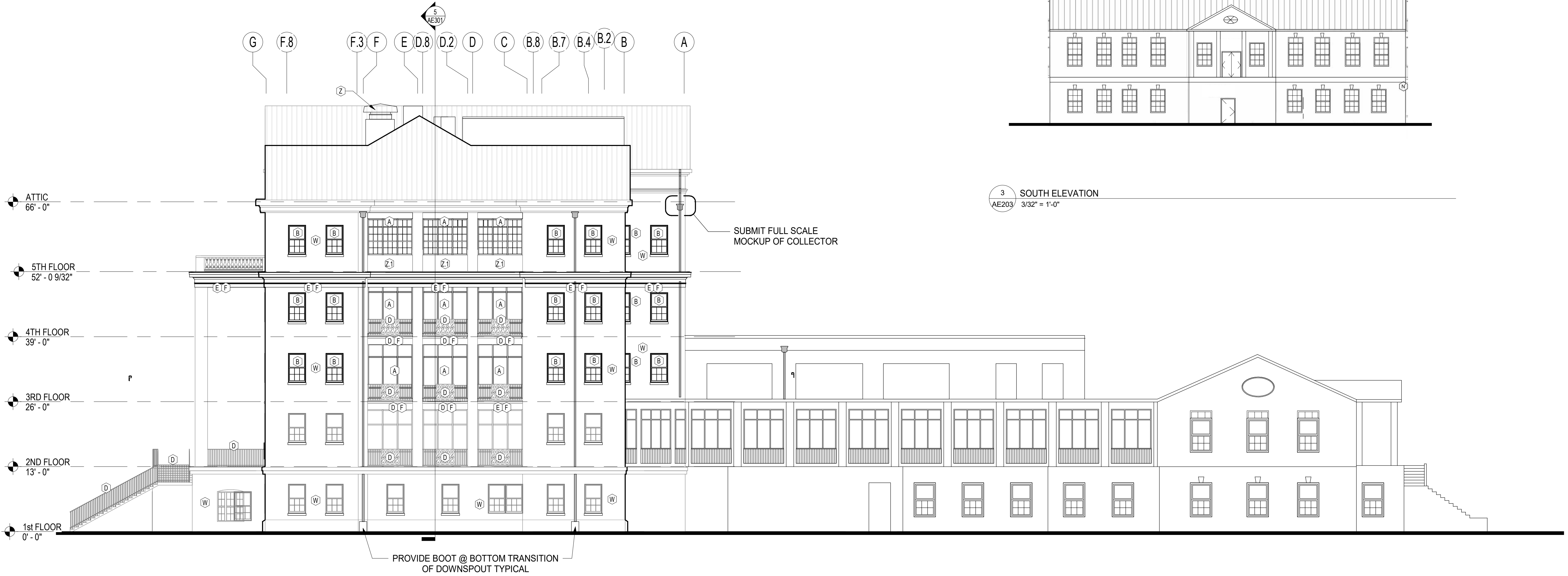
2 WEST EXTERIOR ELEVATION AE203 3/32" = 1'-0"
