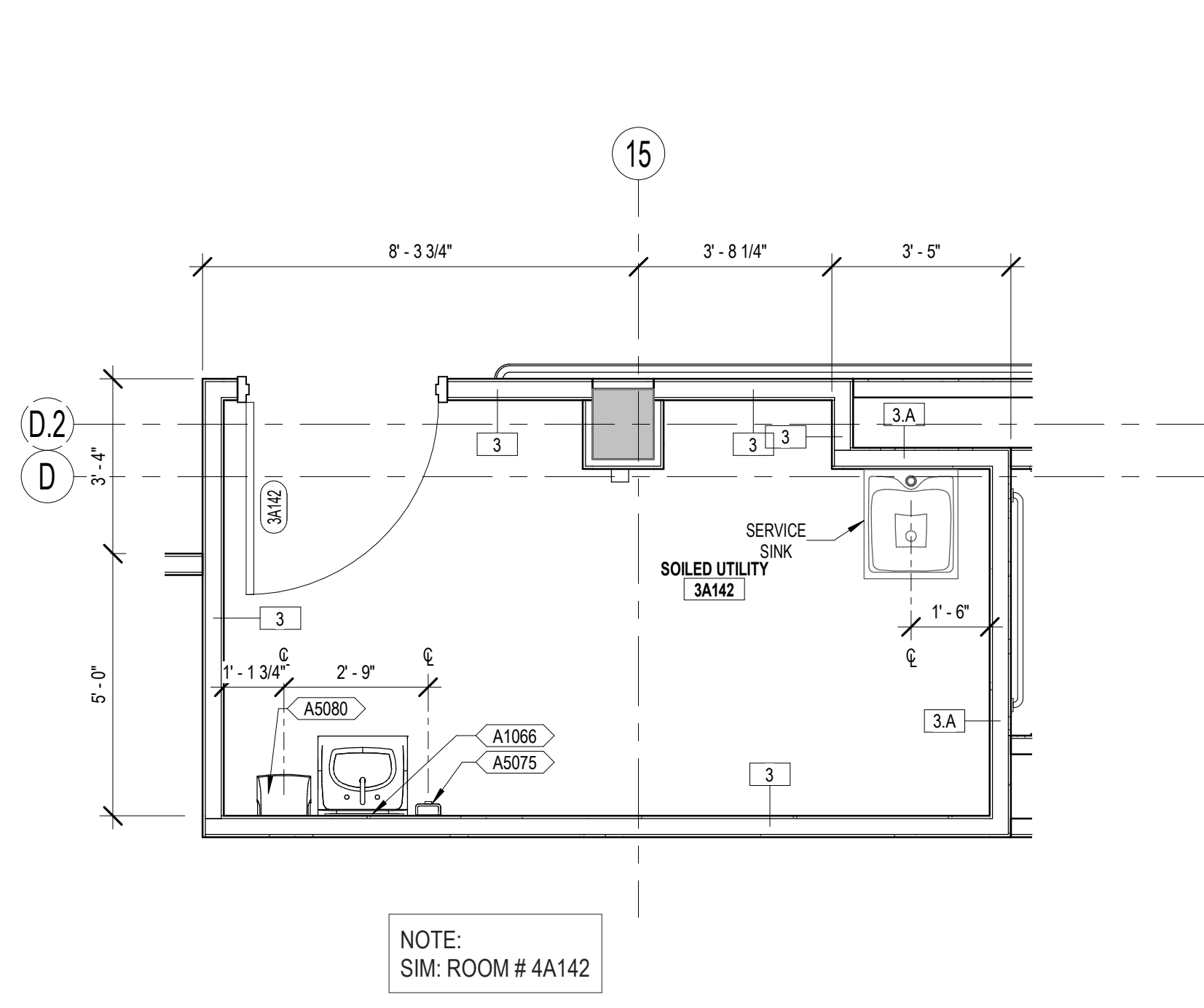
3 ENLARGED FLOOR PLAN AE125 3/8" = 1'-0"
