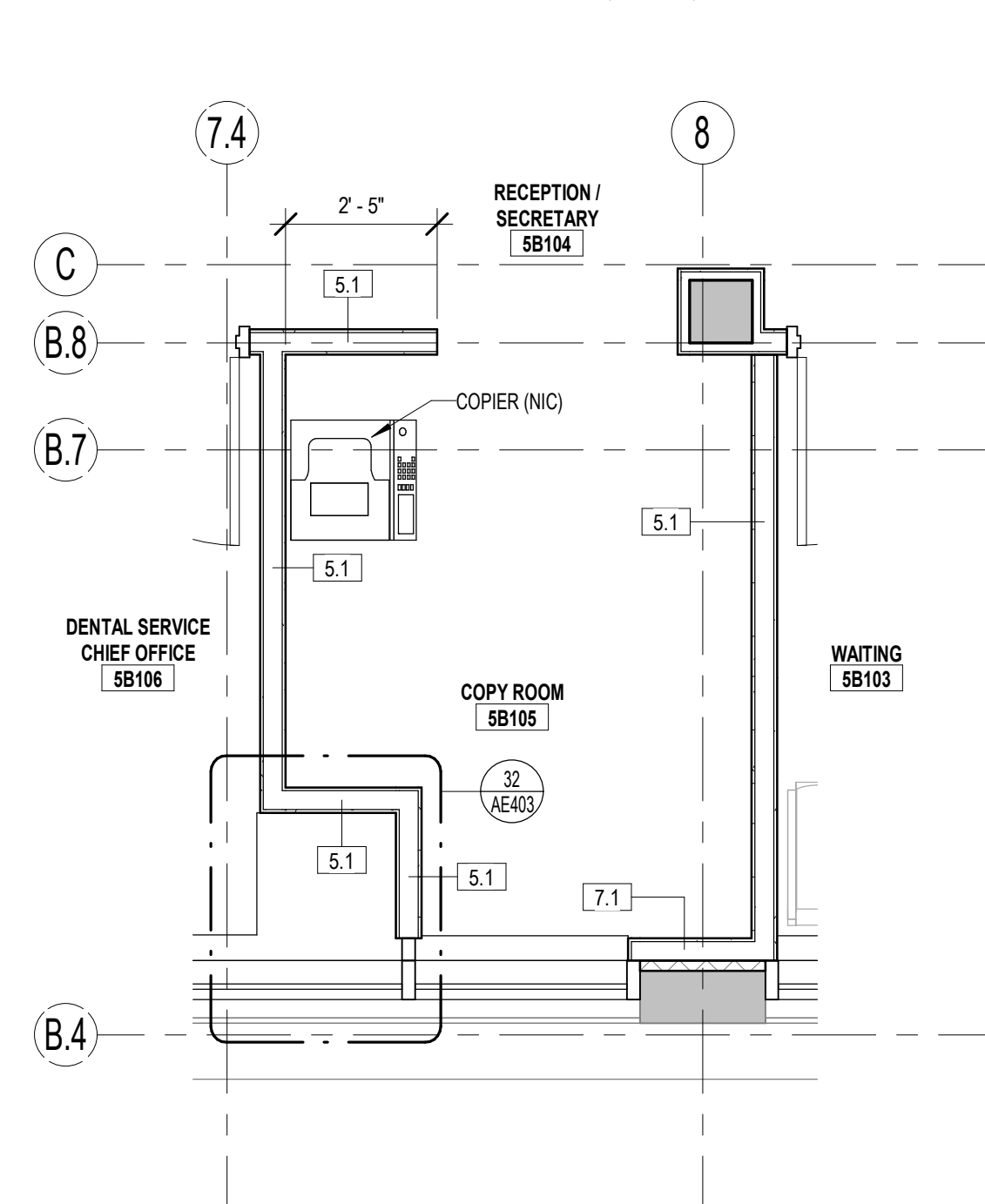
9 ENLARGED FLOOR PLAN AE125 3/8" = 1'-0"
