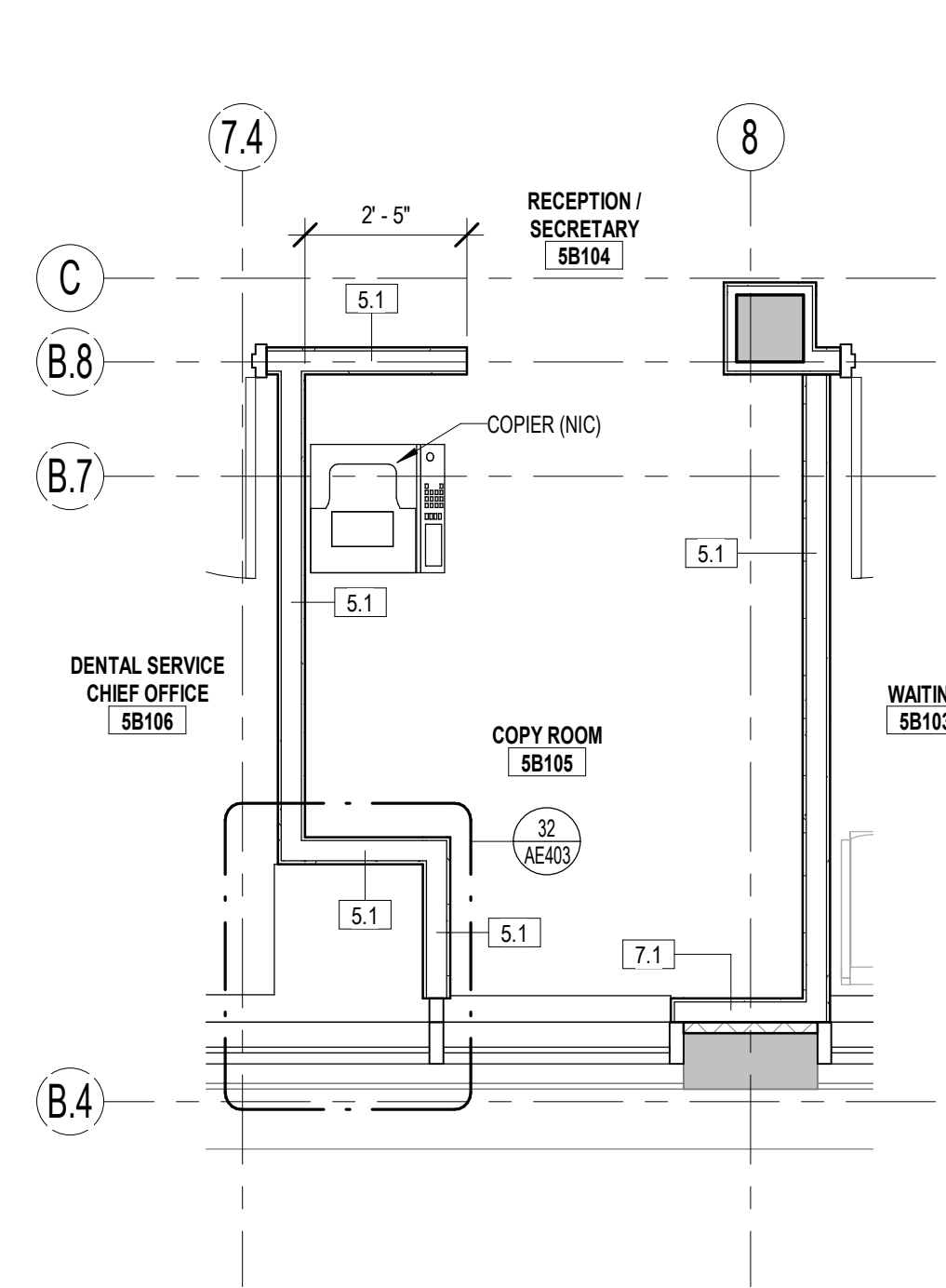
9 ENLARGED FLOOR PLAN AE125 3/8" = 1'-0"
