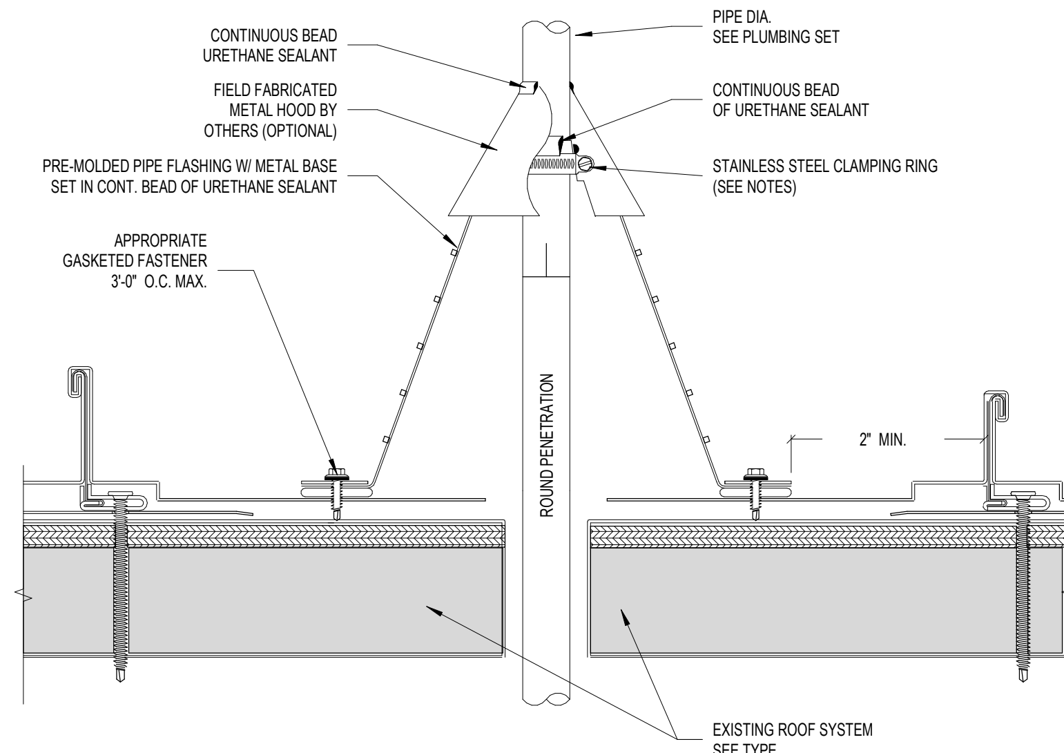
6 VENT THRU METAL ROOF AE106/ 6" = 1'-0"
