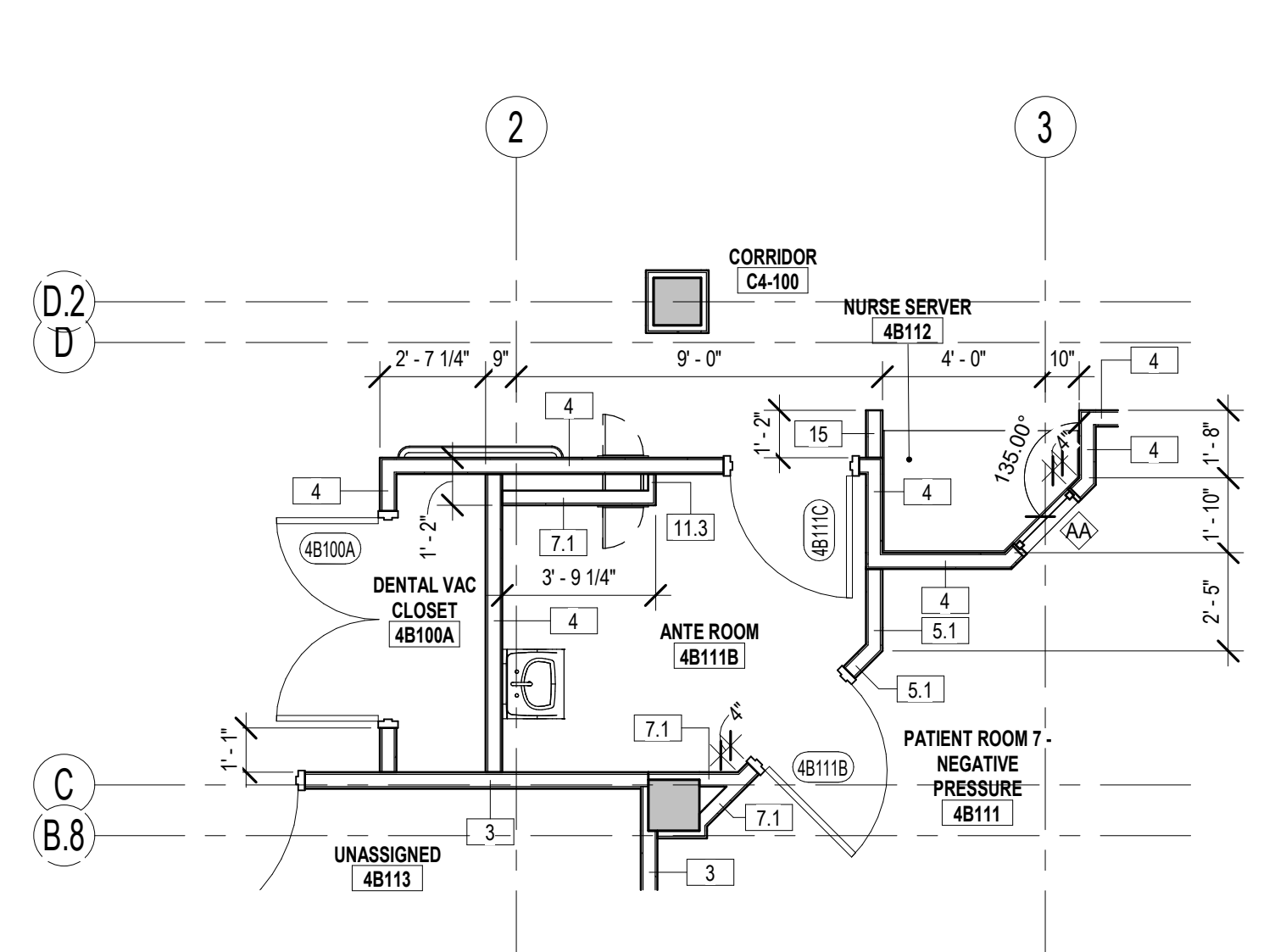
10 ENLARGED DIMENSION PLAN - 4B111B AE108.2 1/4" = 1'-0"
