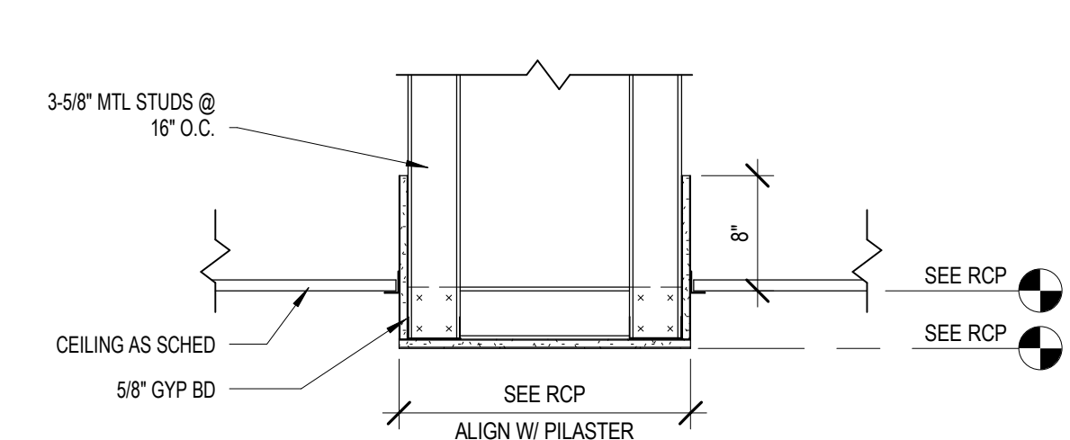
2 TYPICAL CORRIDOR FURDOWN AE111 1" = 1'-0"
