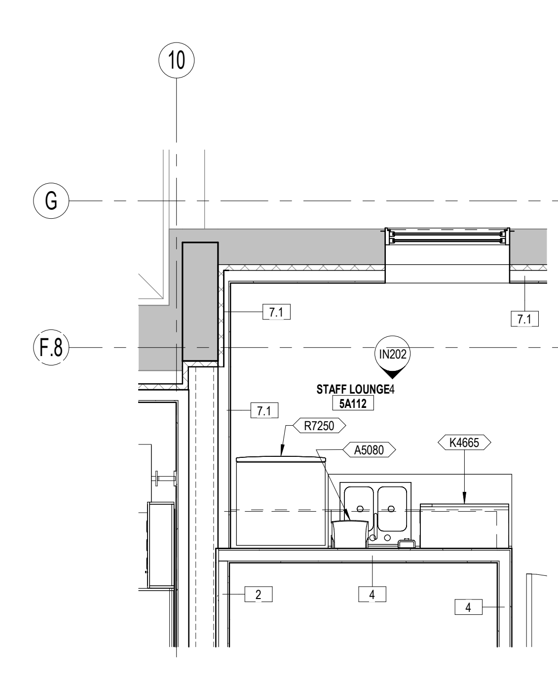
7 ENLARGED FLOOR PLAN AE125 3/8" = 1'-0"
