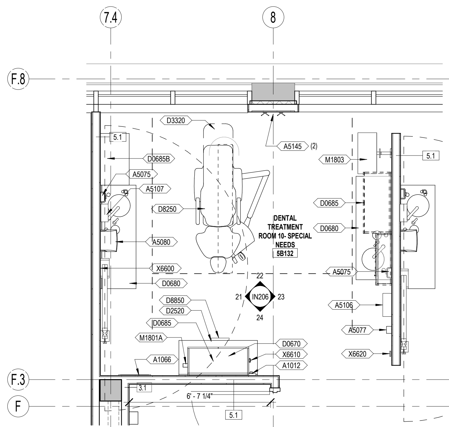
3 DENTAL TREATMENT ROOM 10 - SPECIAL NEEDS AE124 3/8" = 1'-0"
