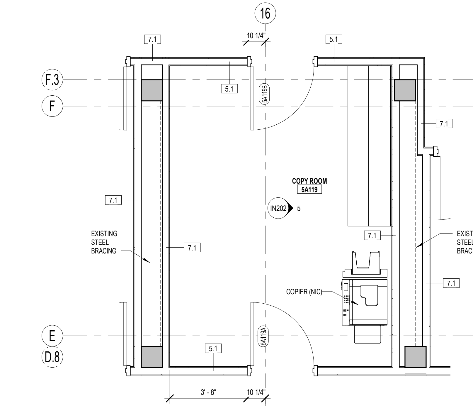
10 ENLARGED FLOOR PLAN AE125 3/8" = 1'-0"
