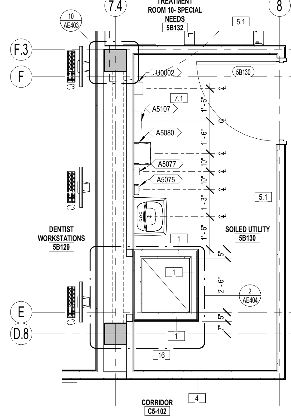
6 ENLARGED FLOOR PLAN AE125 3/8" = 1'-0"
