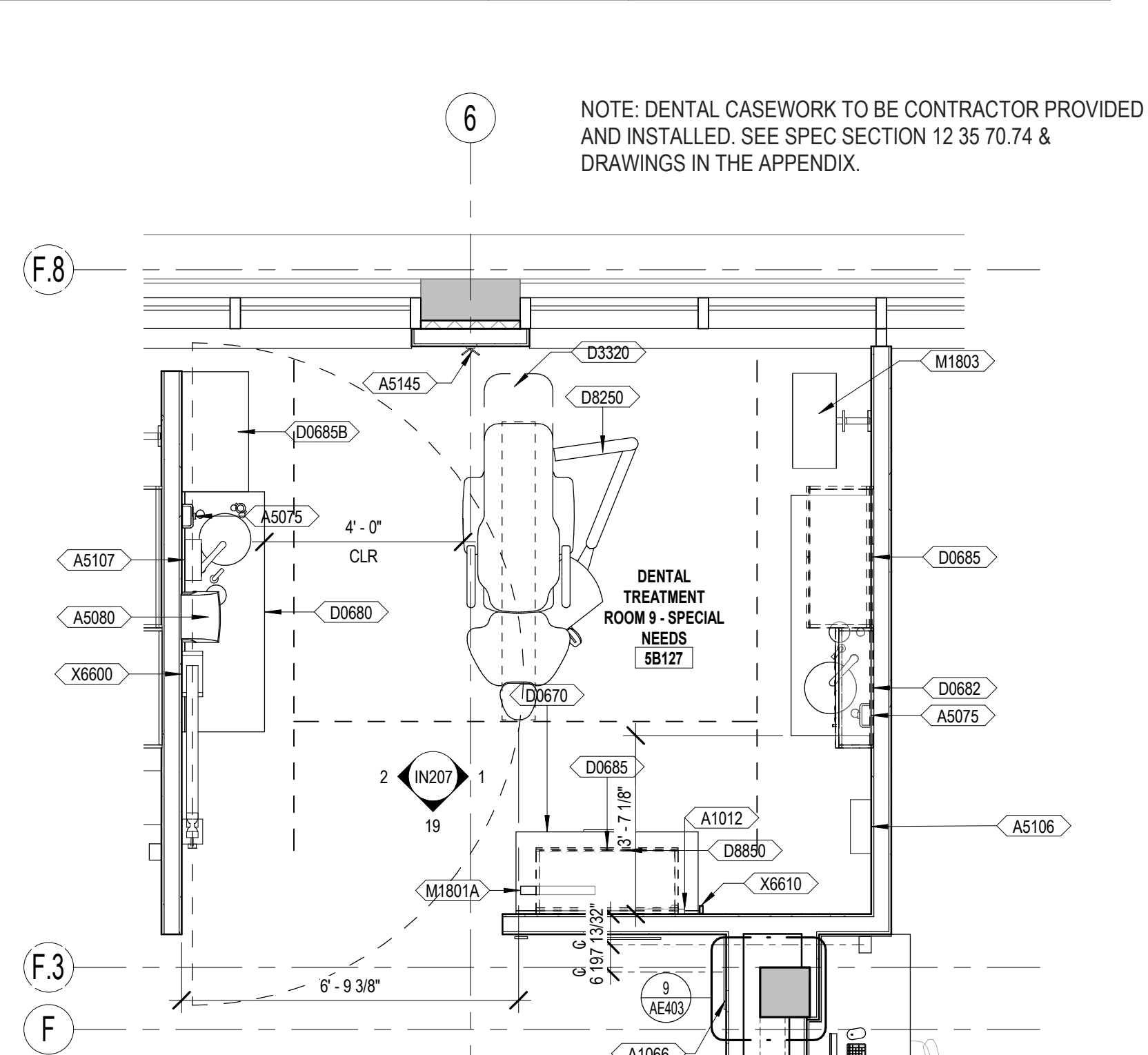
5 DENTAL TREATMENT ROOM 9 - SPECIAL NEEDS AE124 3/8" = 1'-0"
