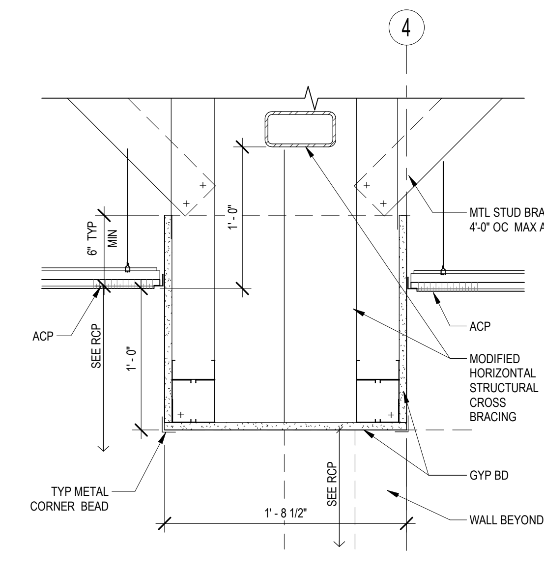
4 BULKHEAD DETAIL AE113 1 1/2\"/>
