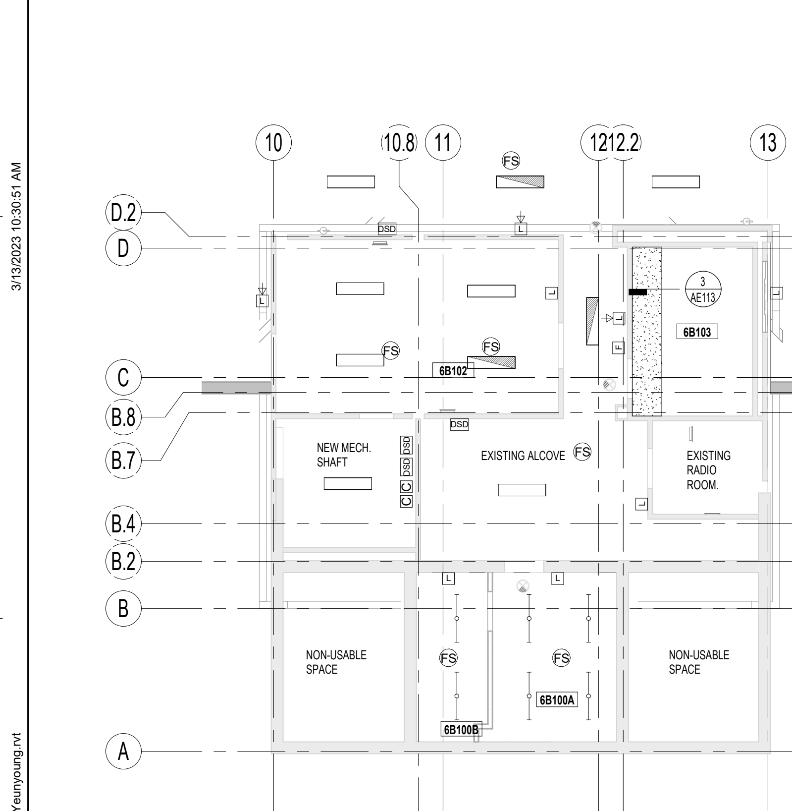
2 ATTIC REFLECTED CEILING PLAN AE113 1/8" = 1'-0"
