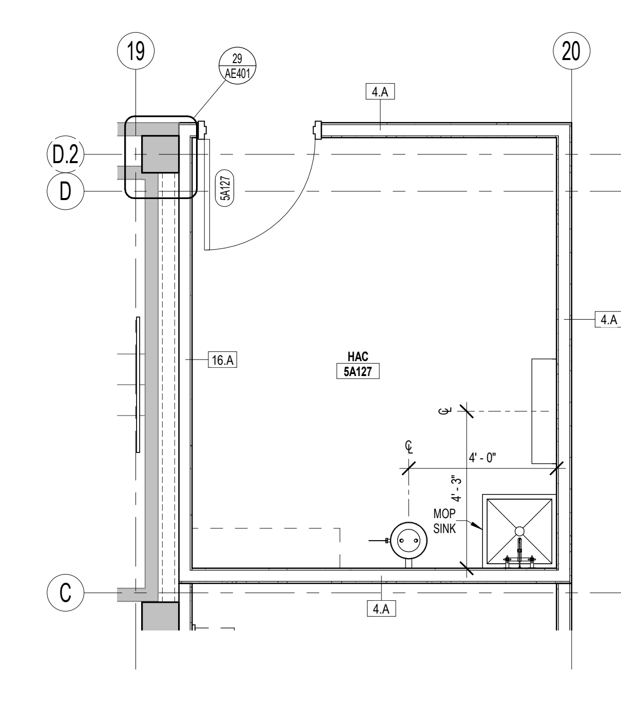
11 ENLARGED FLOOR PLAN AE125 3/8" = 1'-0"
