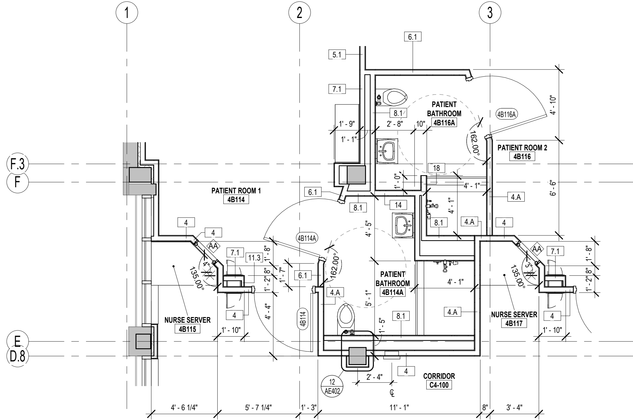
1 ENLARGED DIMENSION PLAN - 4B114/4B116A AE108.2 1/4" = 1'-0"
