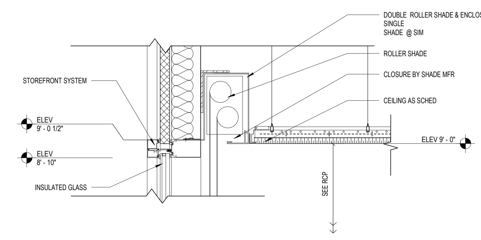
2 ACT CONNECTION AT DOUBLE ROLLER SHADE AE112 1 1/2" = 1'-0"
