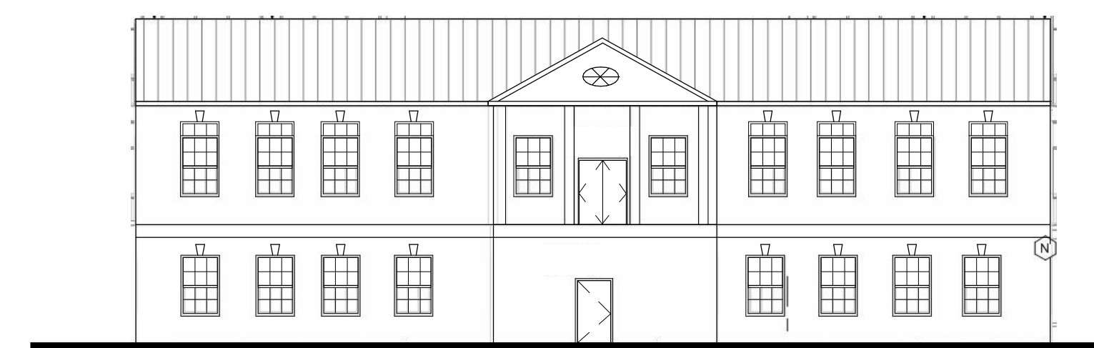
3 SOUTH ELEVATION AE203 3/32" = 1'-0"
