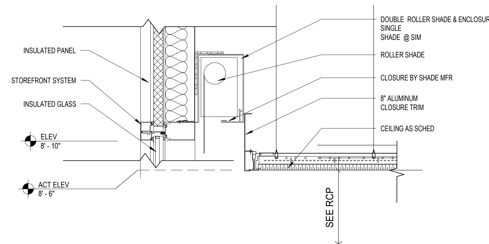
3 ACT CONNECTION AT SINGLE ROLLER SHADE AE112 1 1/2" = 1'-0"
