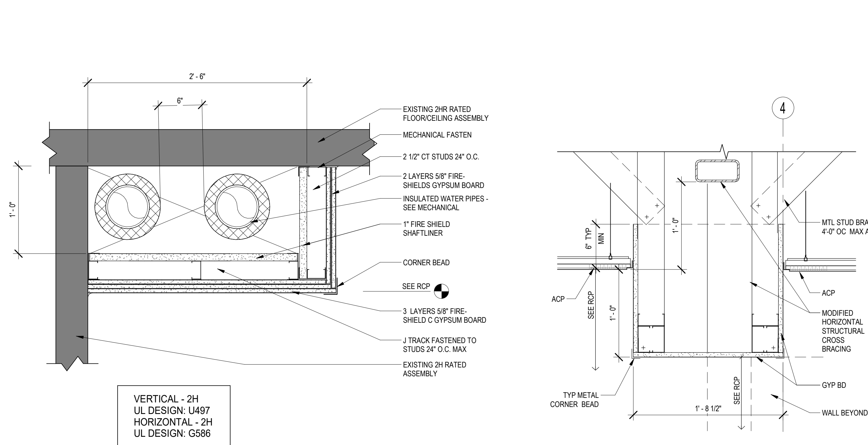
3 2 HR RATED ENCLOSURE AE113 1 1/2\"/>
