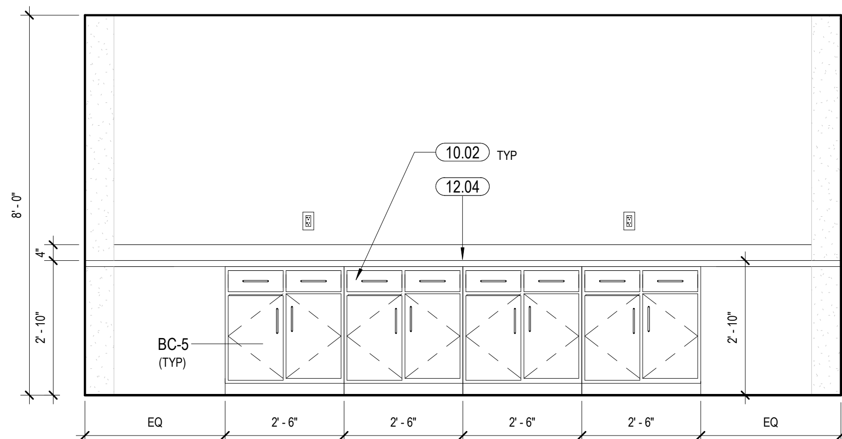
(A1) DAYROOM - INT EL 1 1/2" = 1'-0"
