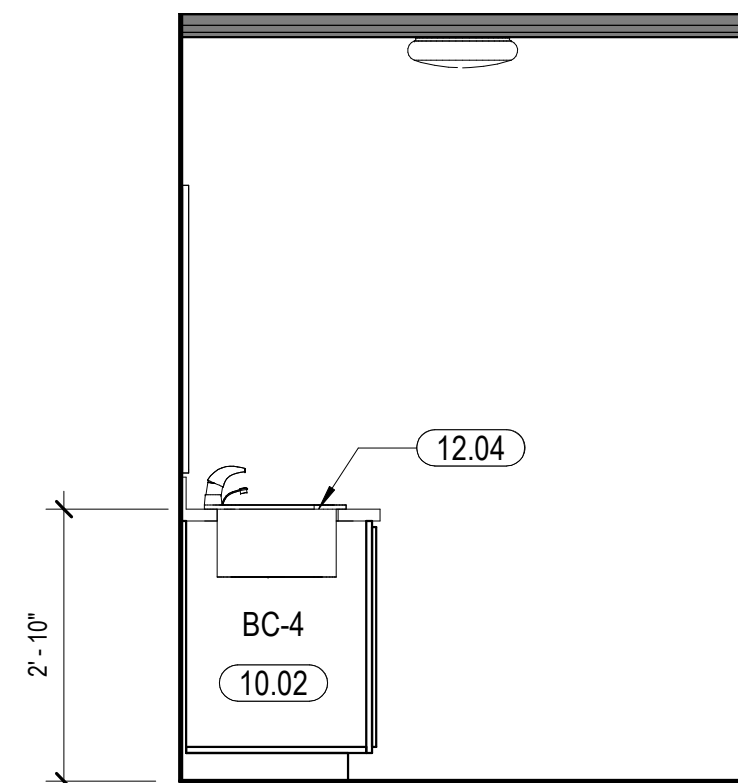
K13 BATHROOM - RM 103 - INT EL 4 1/2" = 1'-0"
