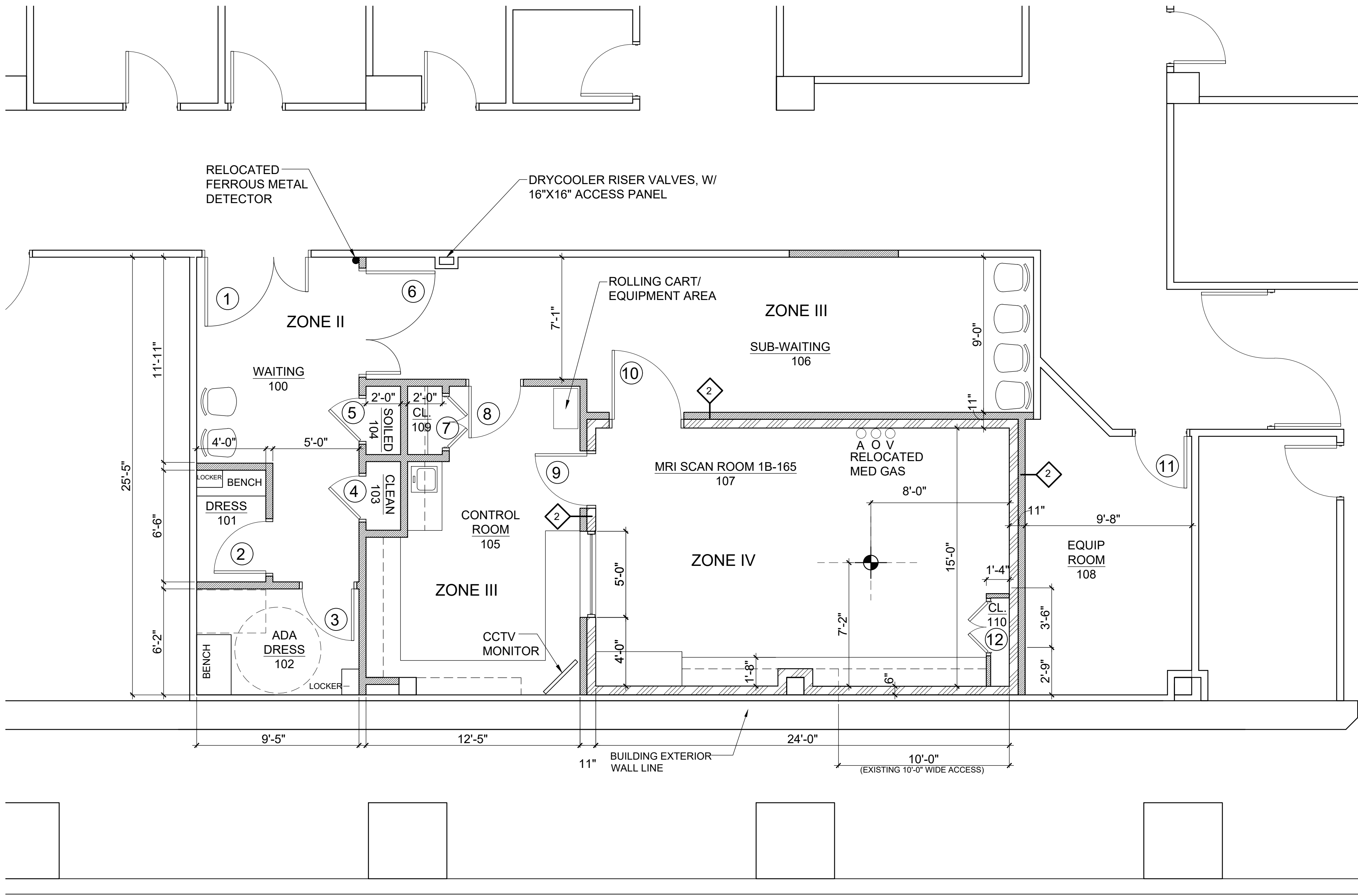
1 FLOOR PLAN SCALE: 1/4" = 1'-0"
